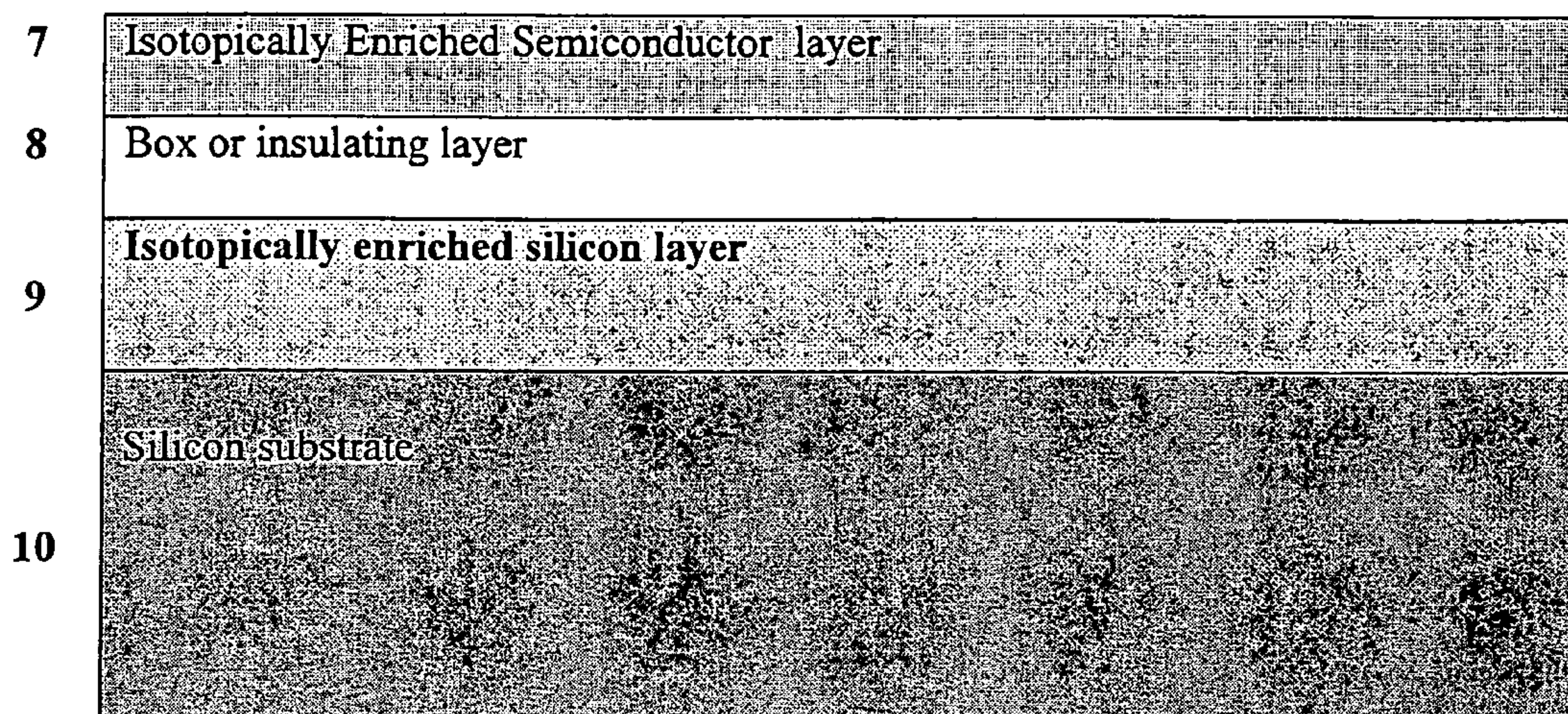
FIGURE 3 EMBODIMENT OF PRESENT INVENTION
