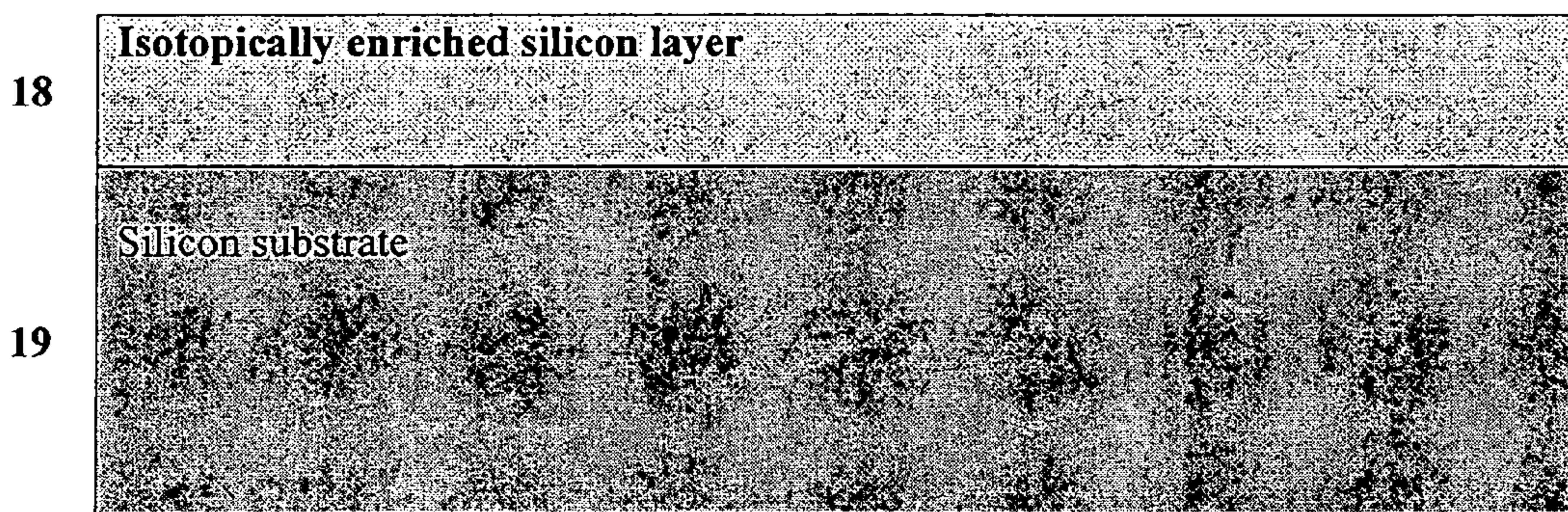
FIGURE 6 HANDLE WAFER BEFORE BONDING
