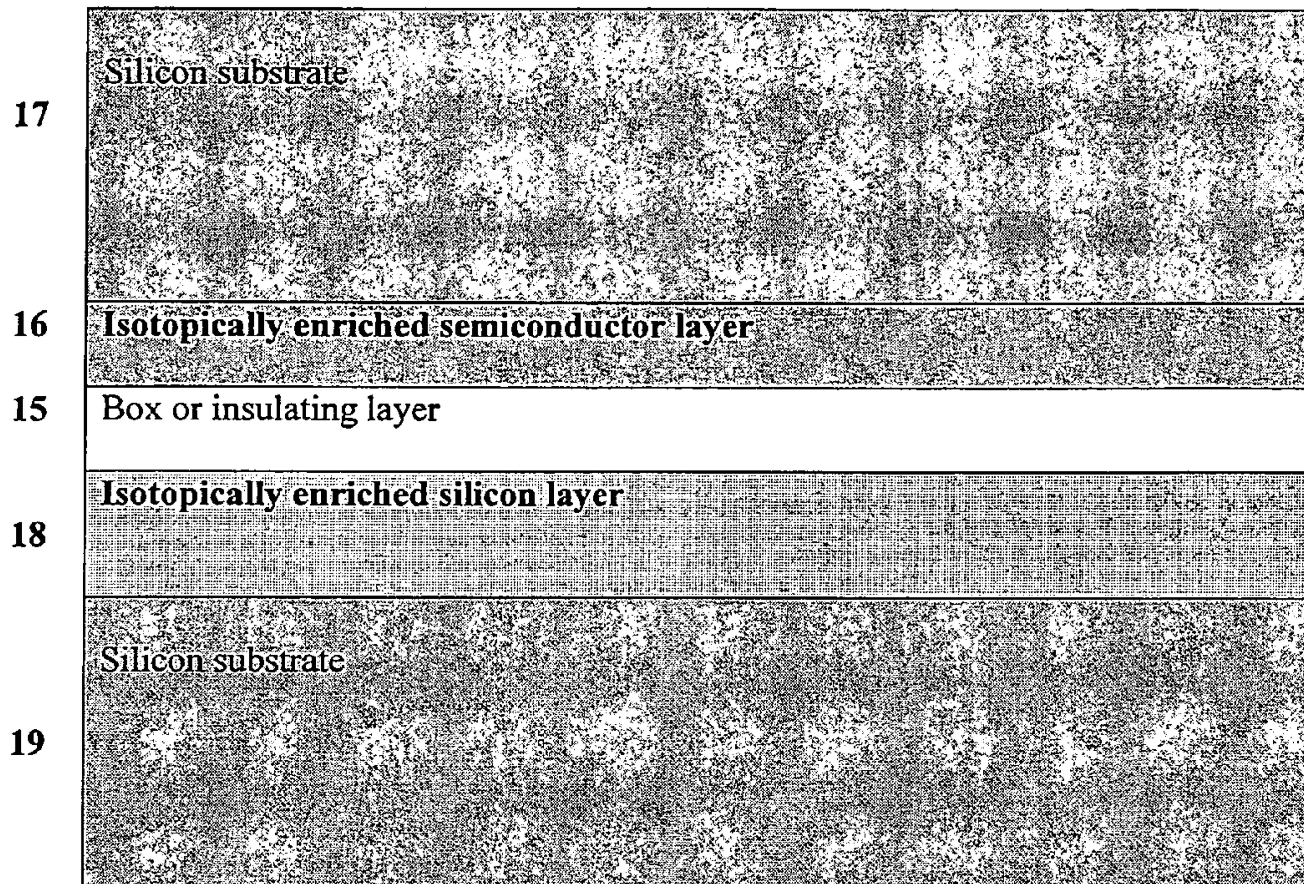
FIGURE 7 WAFER STRUCTURE AFTER BONDING
