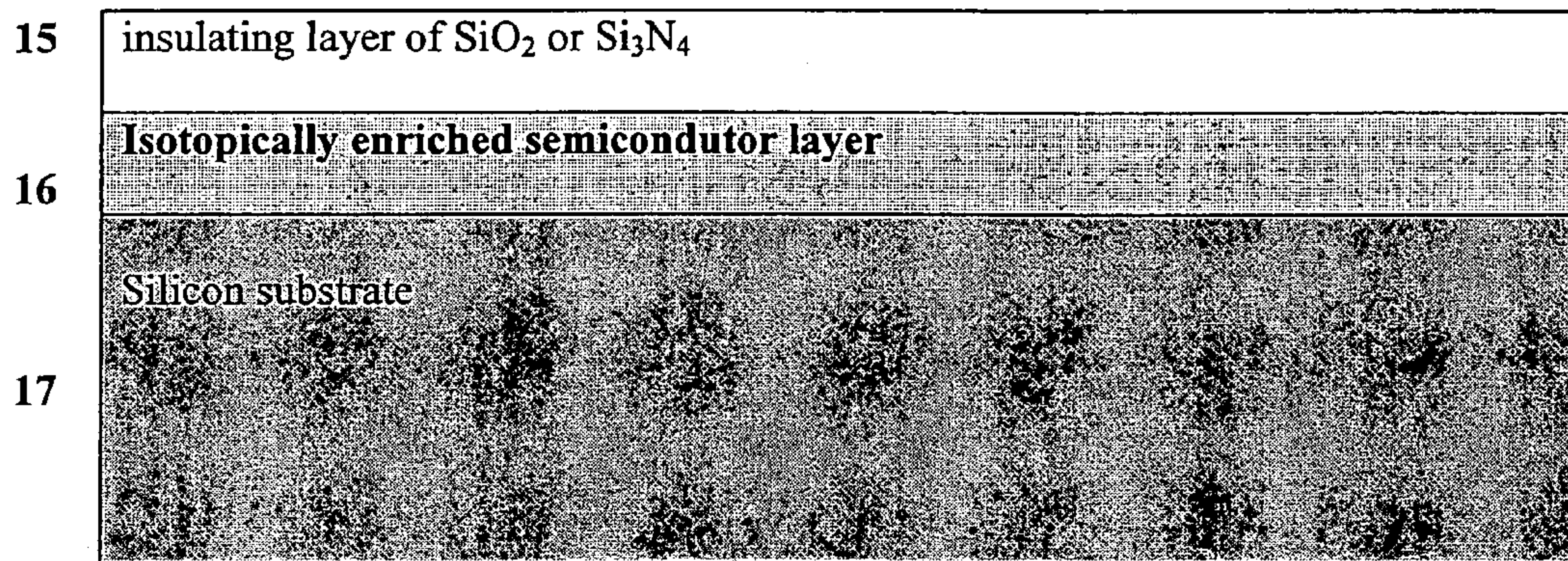
FIGURE 5 DEVICE WAFER BEFORE BONDING
