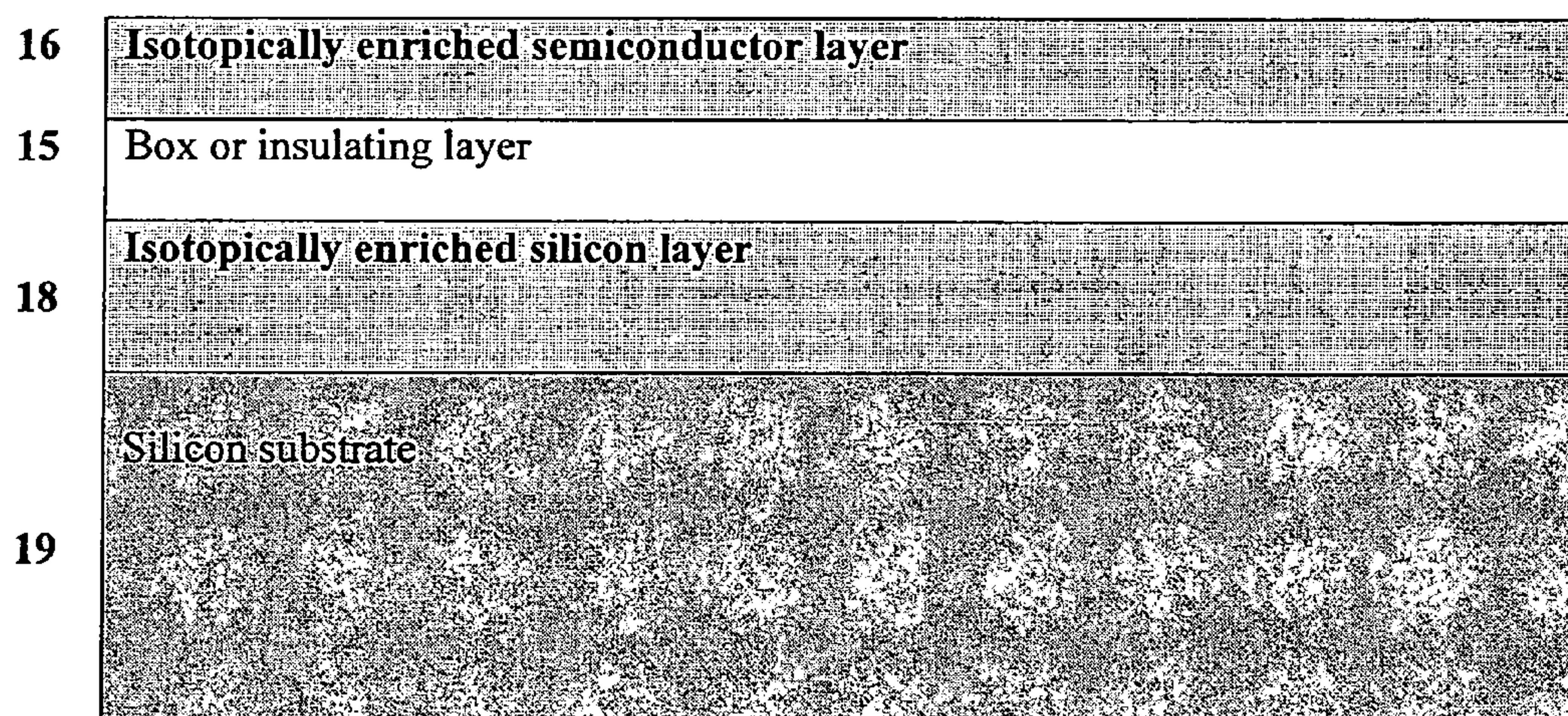
FIGURE 8 FINAL WAFER STRUCTURE
