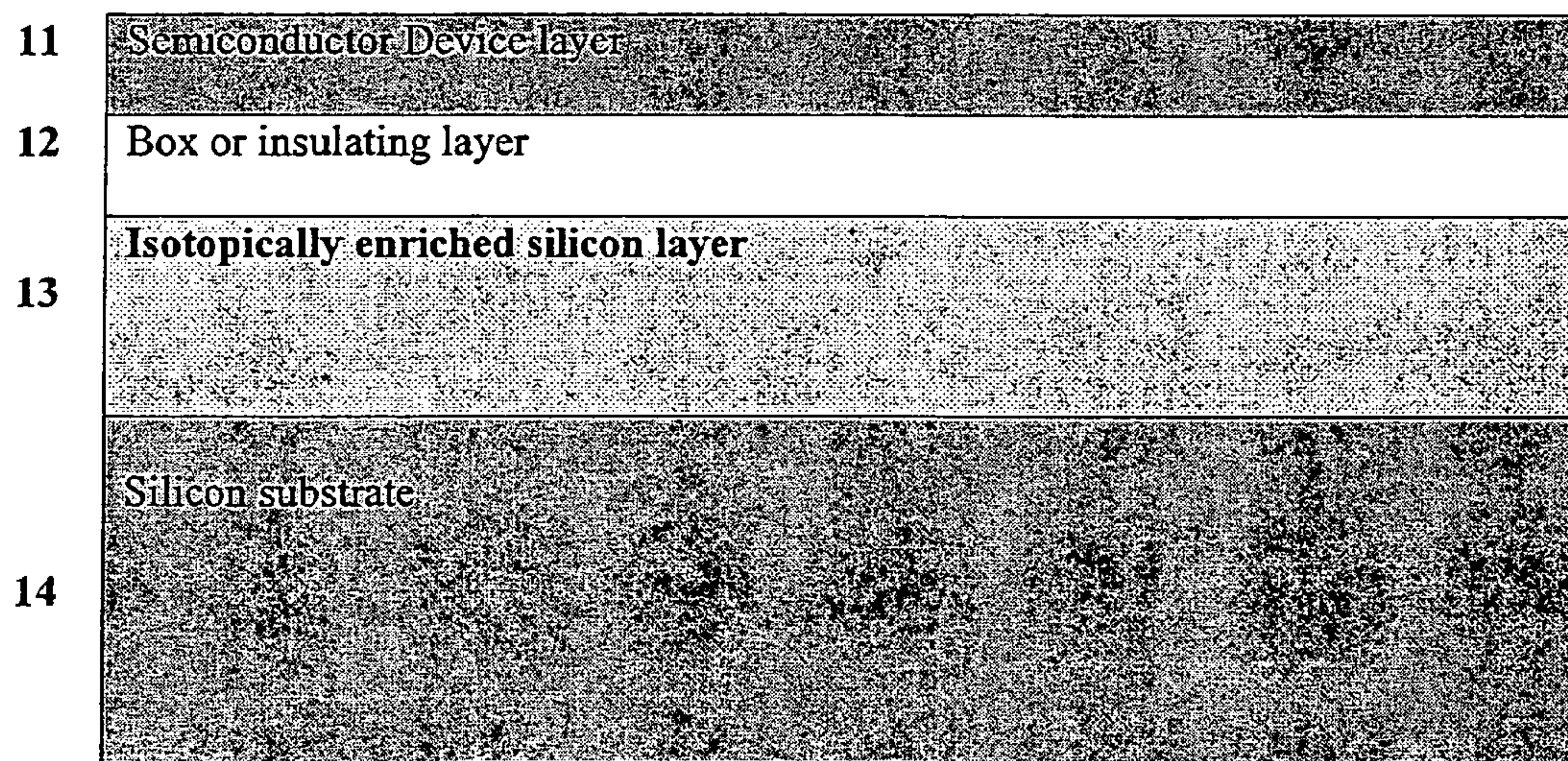
FIGURE 4 EMBODIMENT OF PRESENT INVENTION
