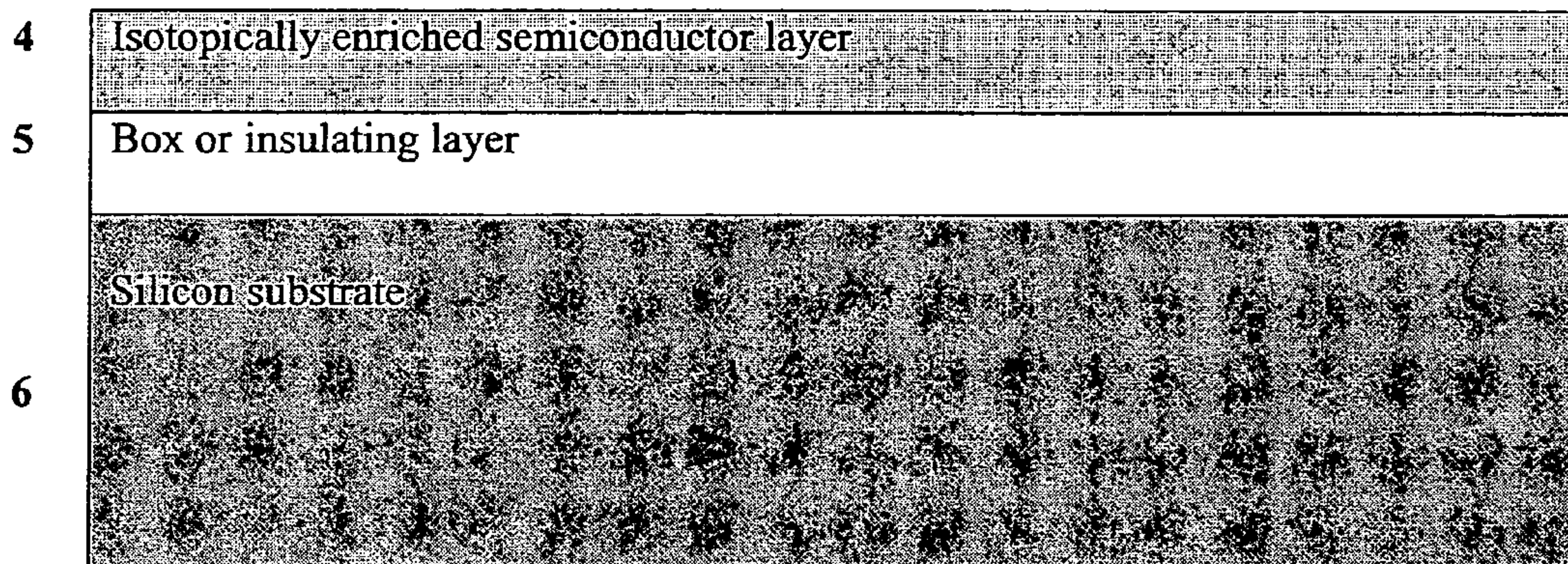
FIGURE 2 EMBODIMENT OF PRESENT INVENTION
