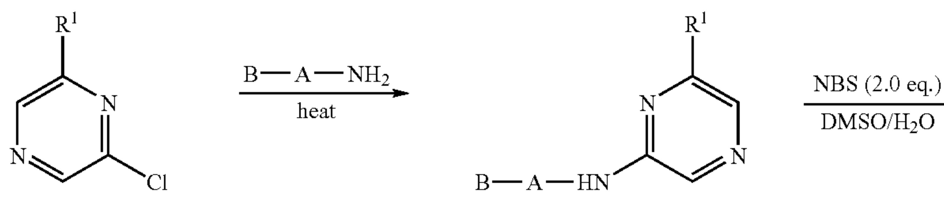
Scheme 11: Introduction of R 2 Groups into Pyrazinone Intermediates and the Resulting Products
