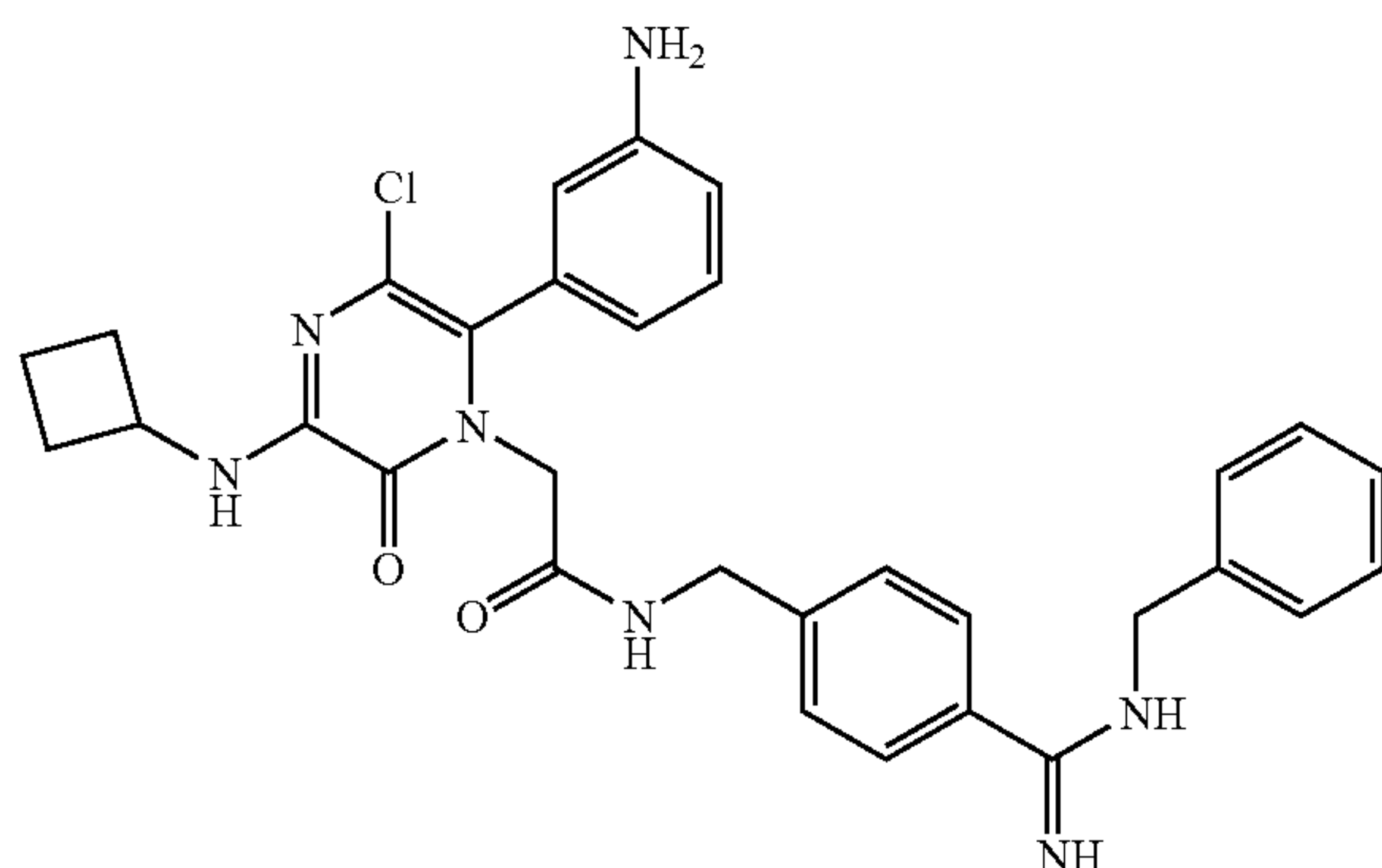
Example 160
