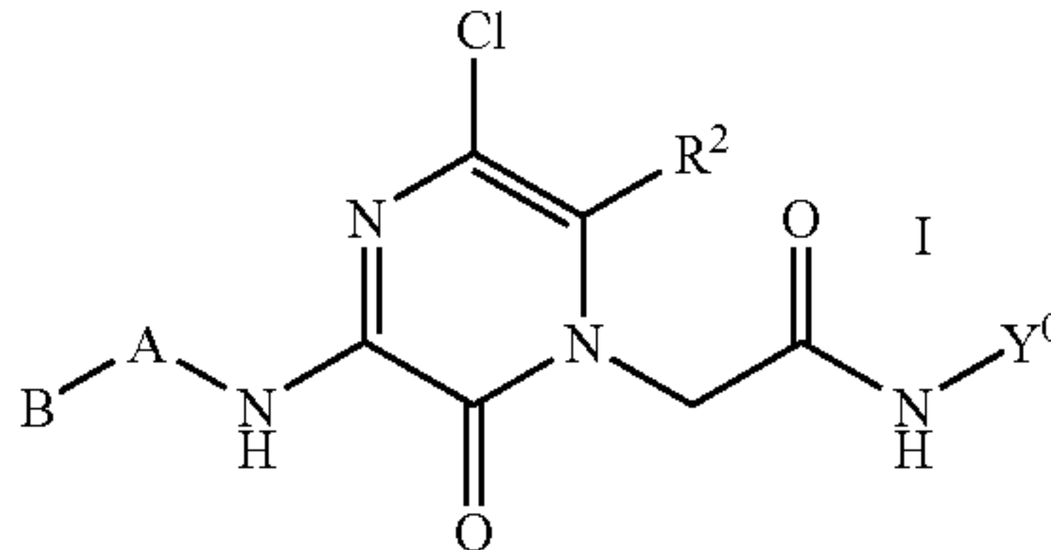
General Structur
