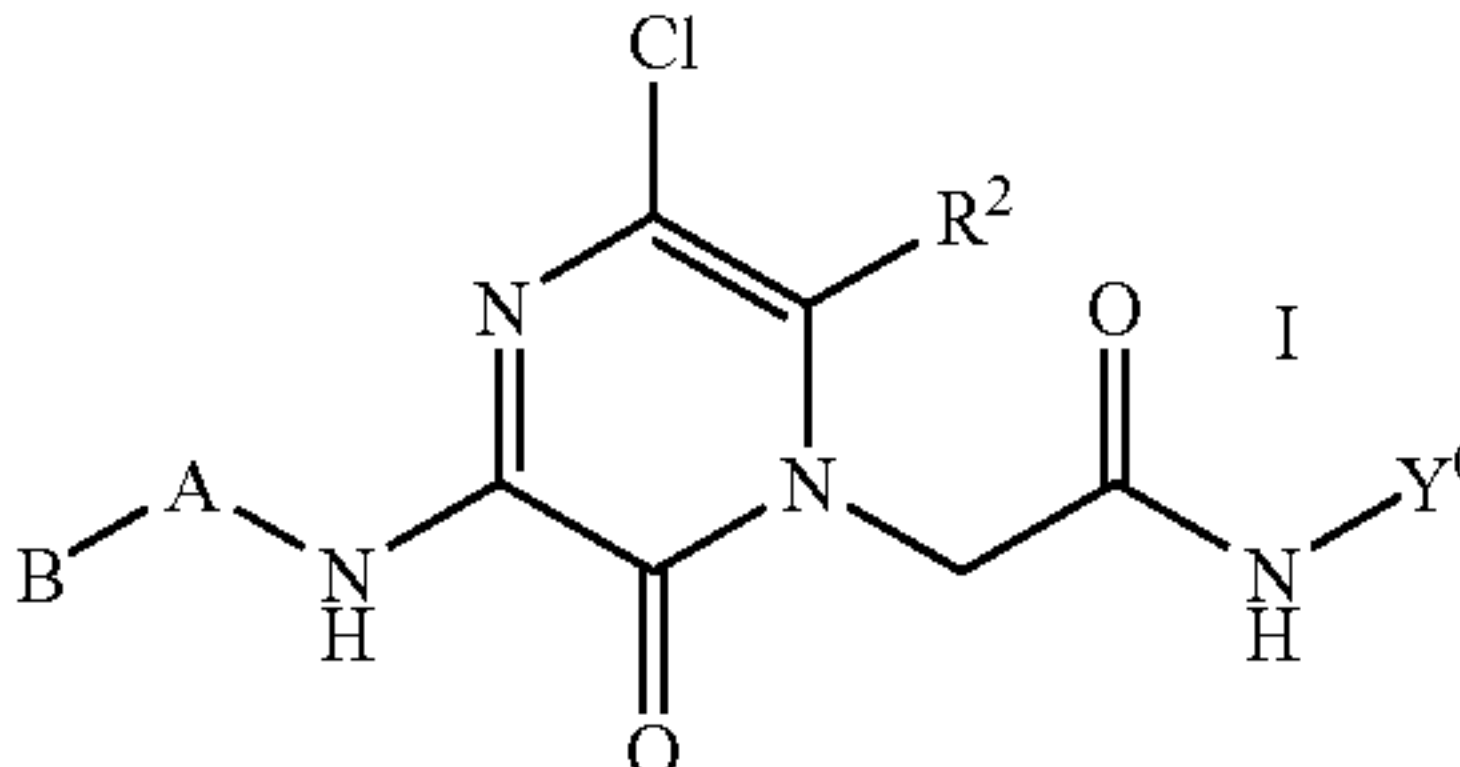
General Structure
