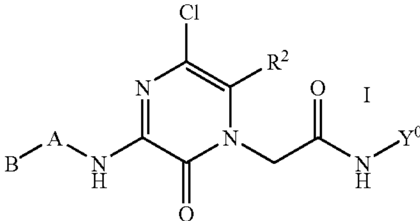
General Structure
