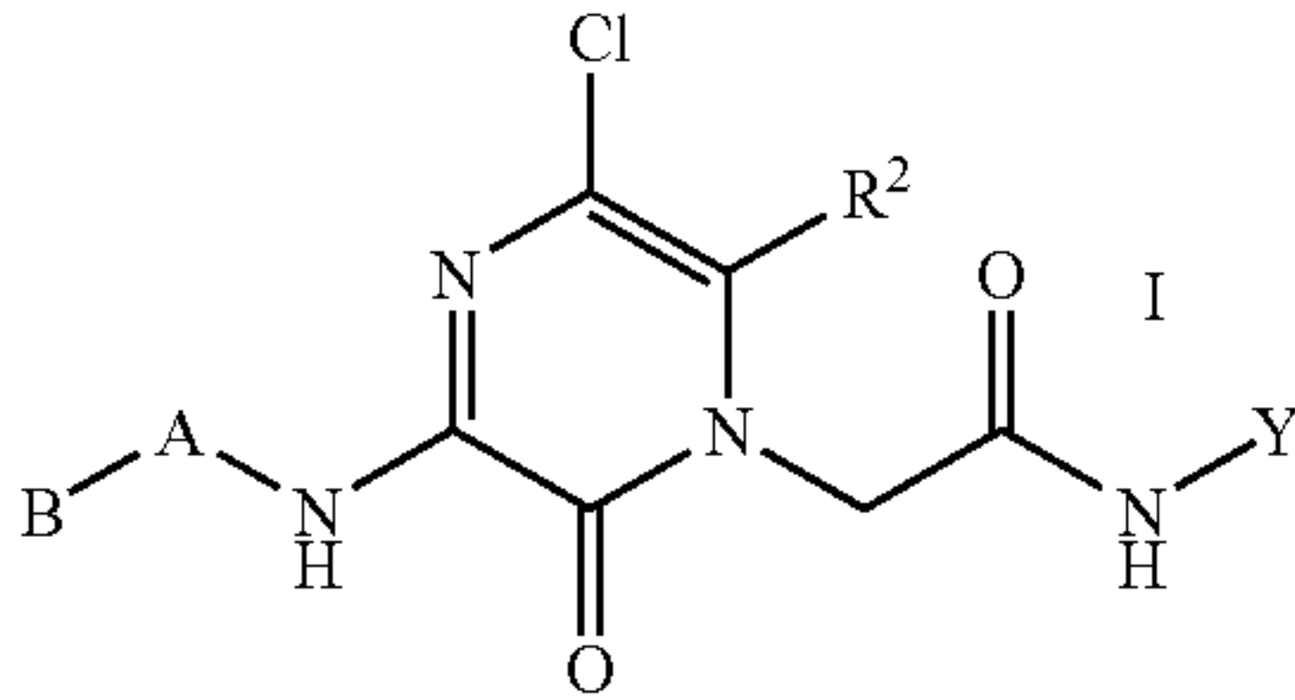
General Structure
