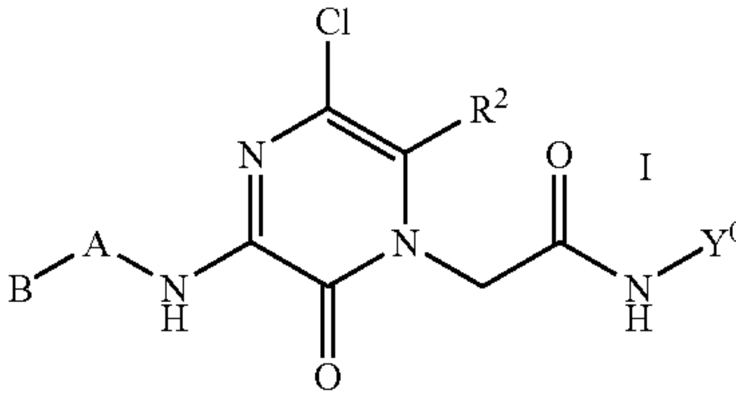
General Structure
