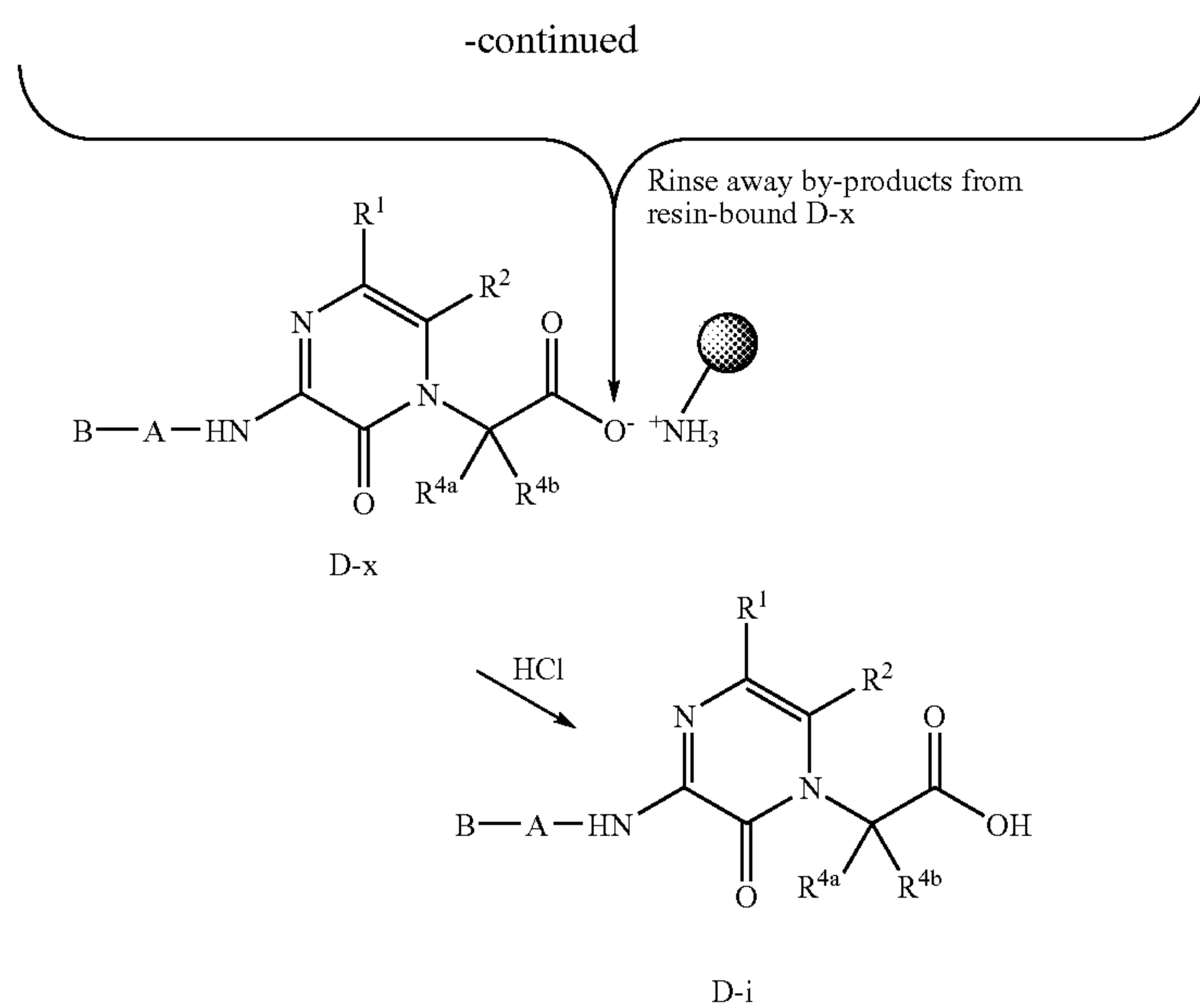
Scheme 6: General Robotic Synthesis (Continued)
