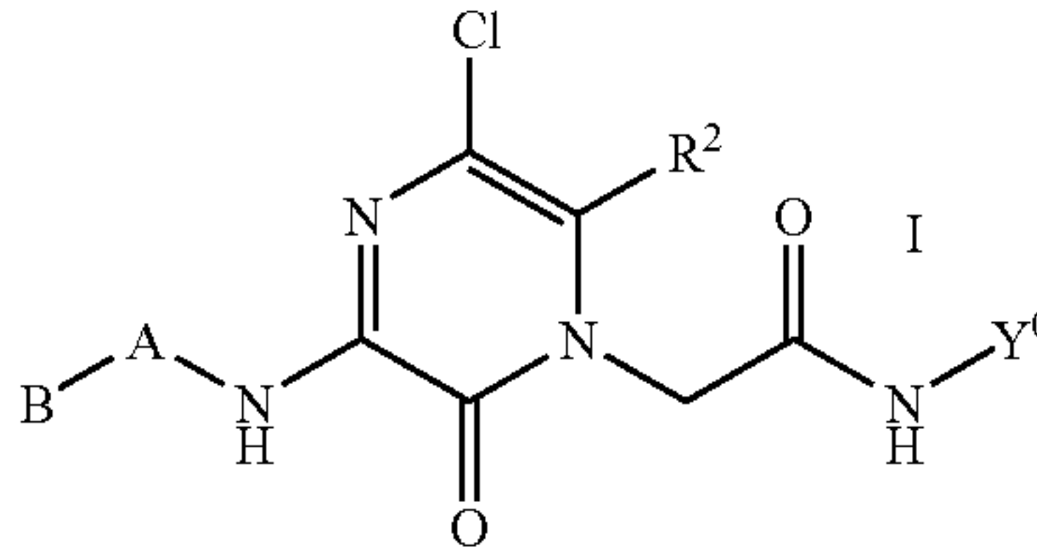
General Structur
