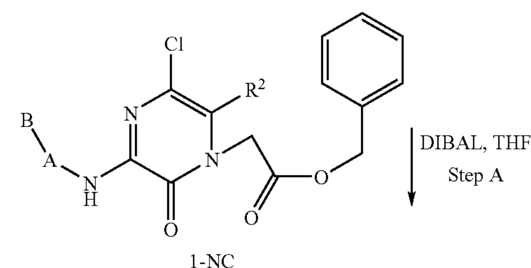
Scheme 4: Methylene Pyrazinone
