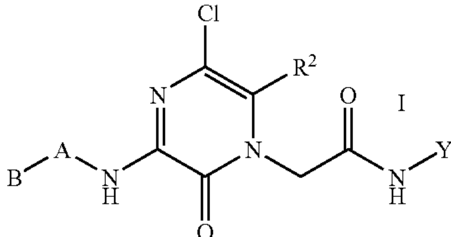
General Structure
