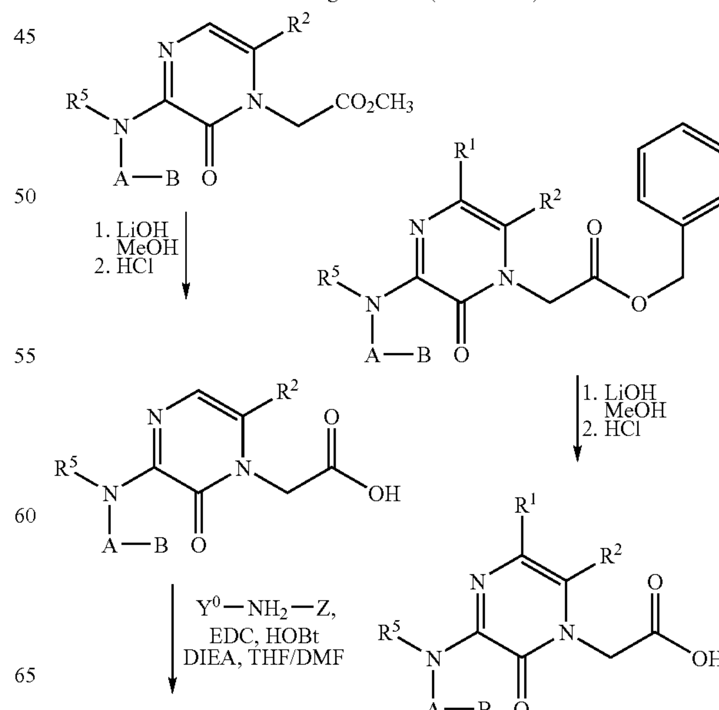
Scheme 10: Introduction of B—A—N(R 5 ) into Pyrazinone Intermediates and the Resulting Products (Concluded)
