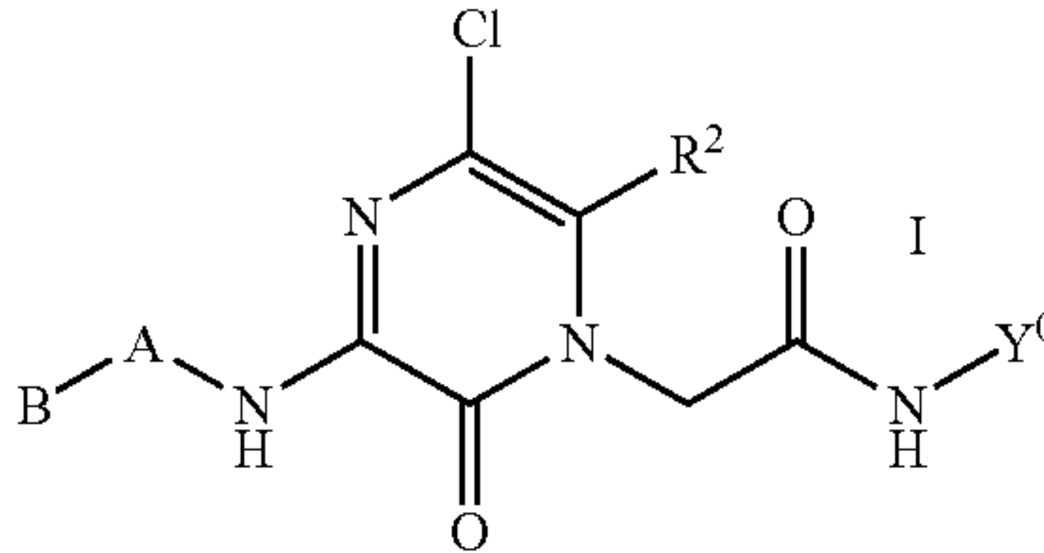
General Structure
