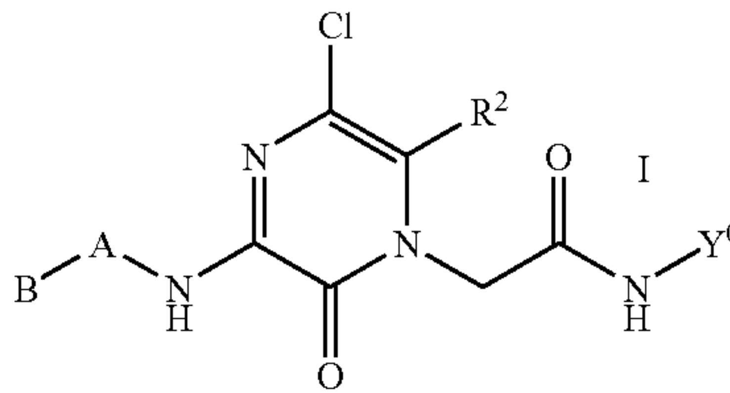
General Structure
