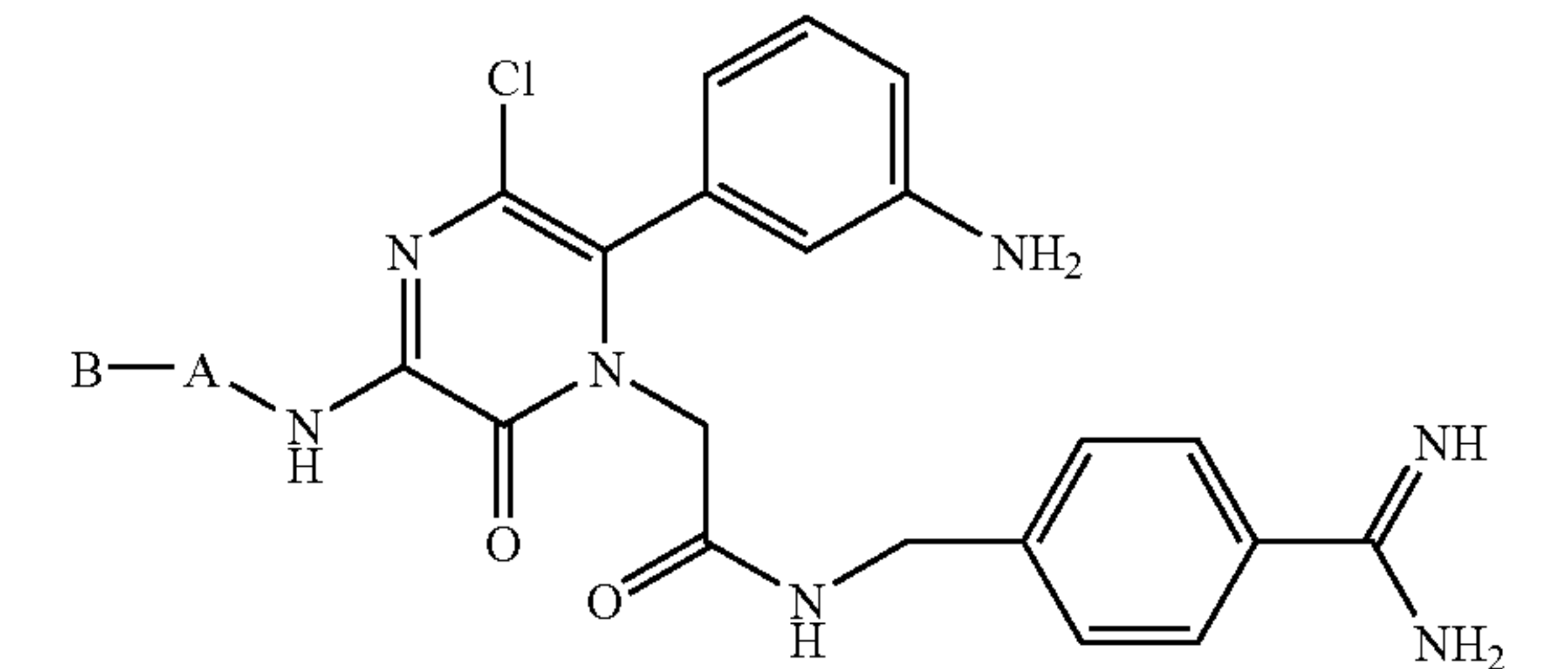
Example Table 2 Additional Substituted Pyrazinones Having a Carboxylic Acid Substituent in the B-A- Group.
