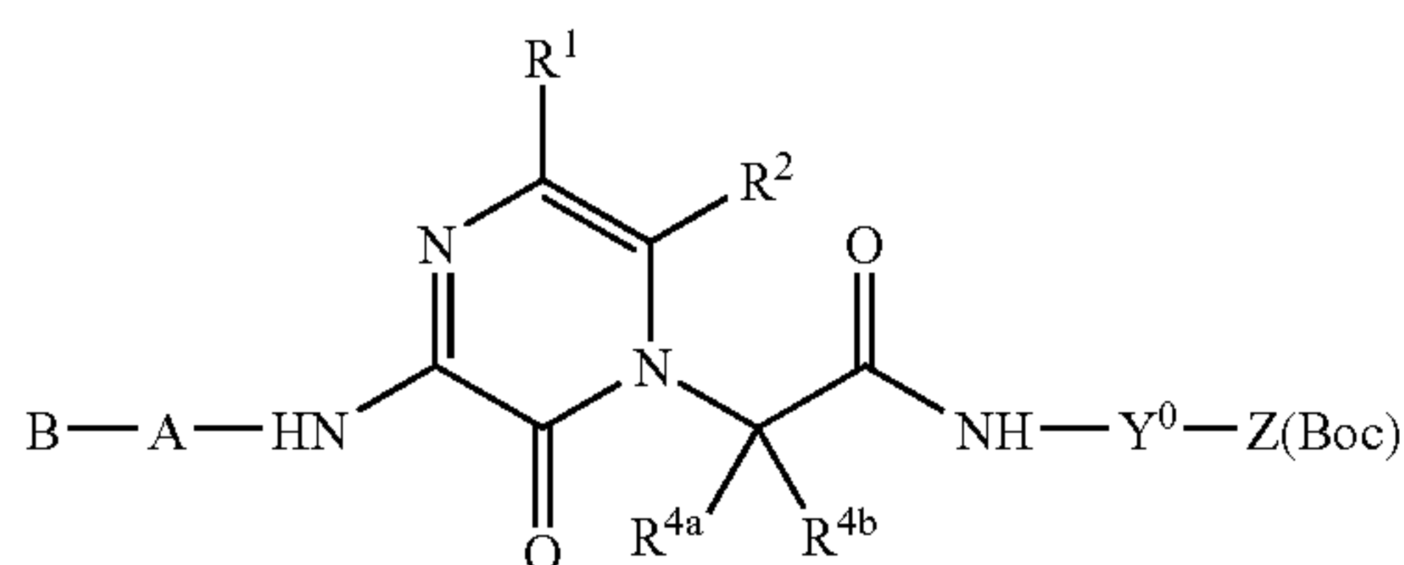
Scheme 8: General Robotic Synthesis (Concluded)
