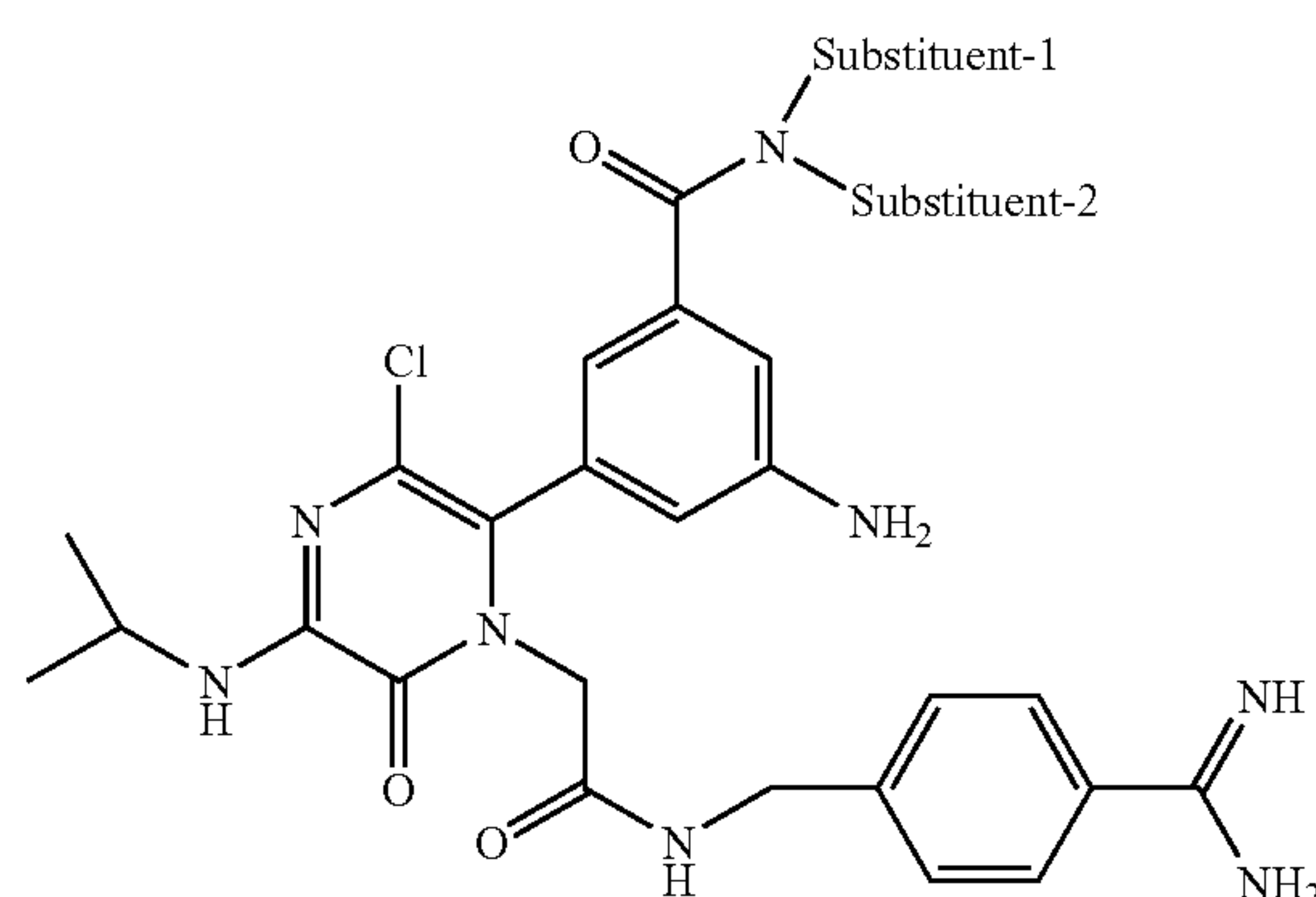
General Structure
