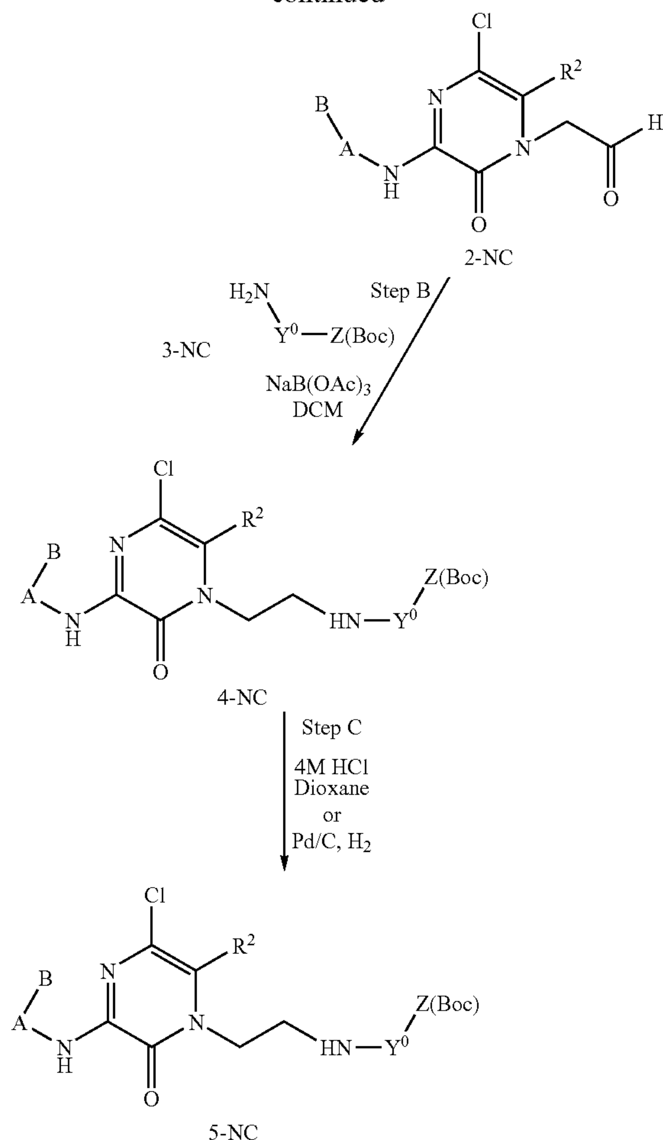
Example 71
