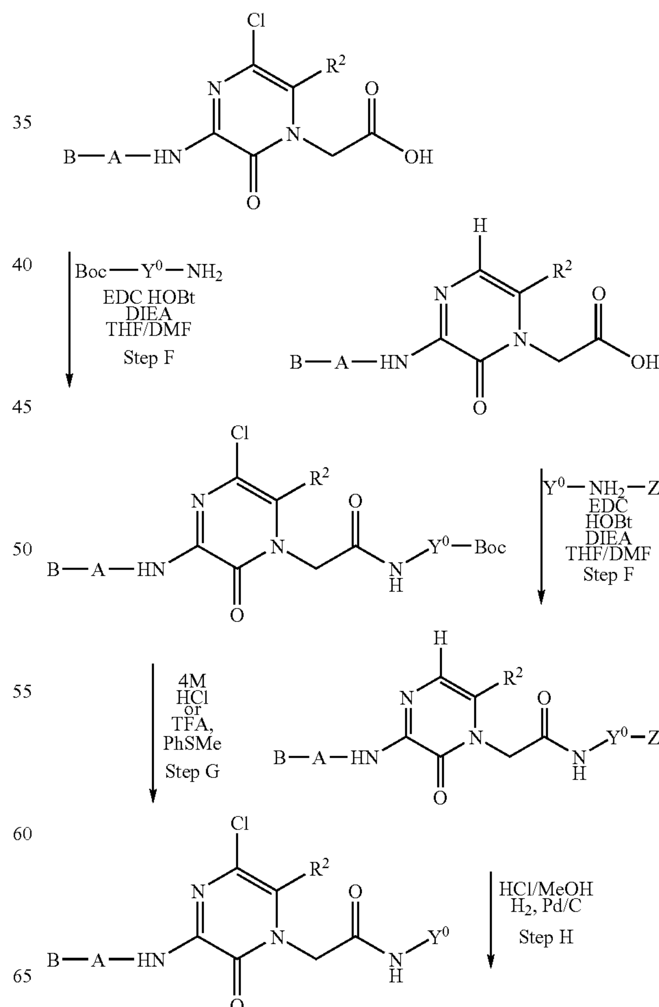
Scheme 2: General Pyrazinone Synthesis (Continued)
