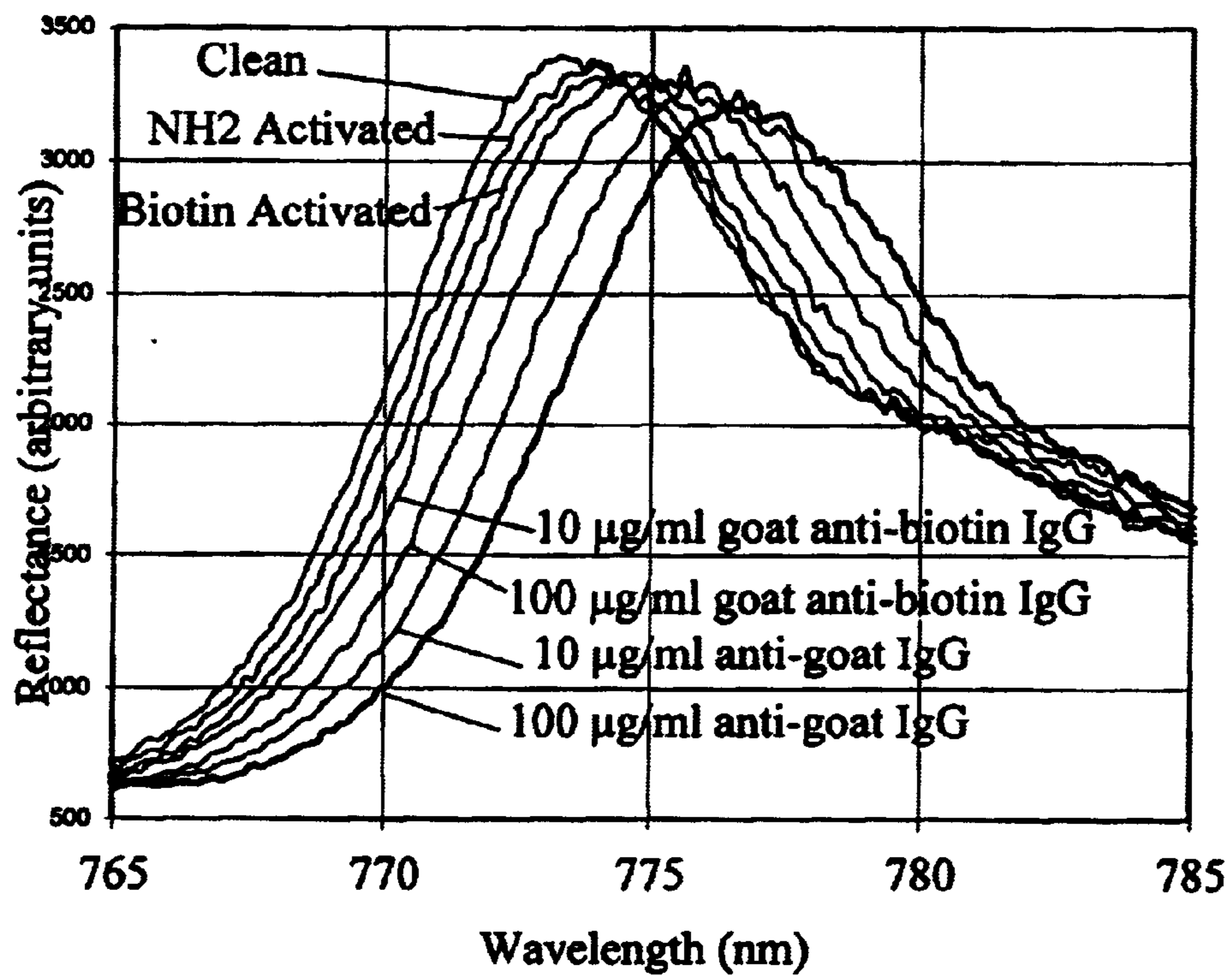
Measured shifting of the resonant wavelength caused by the binding of various biomolecular layers.
