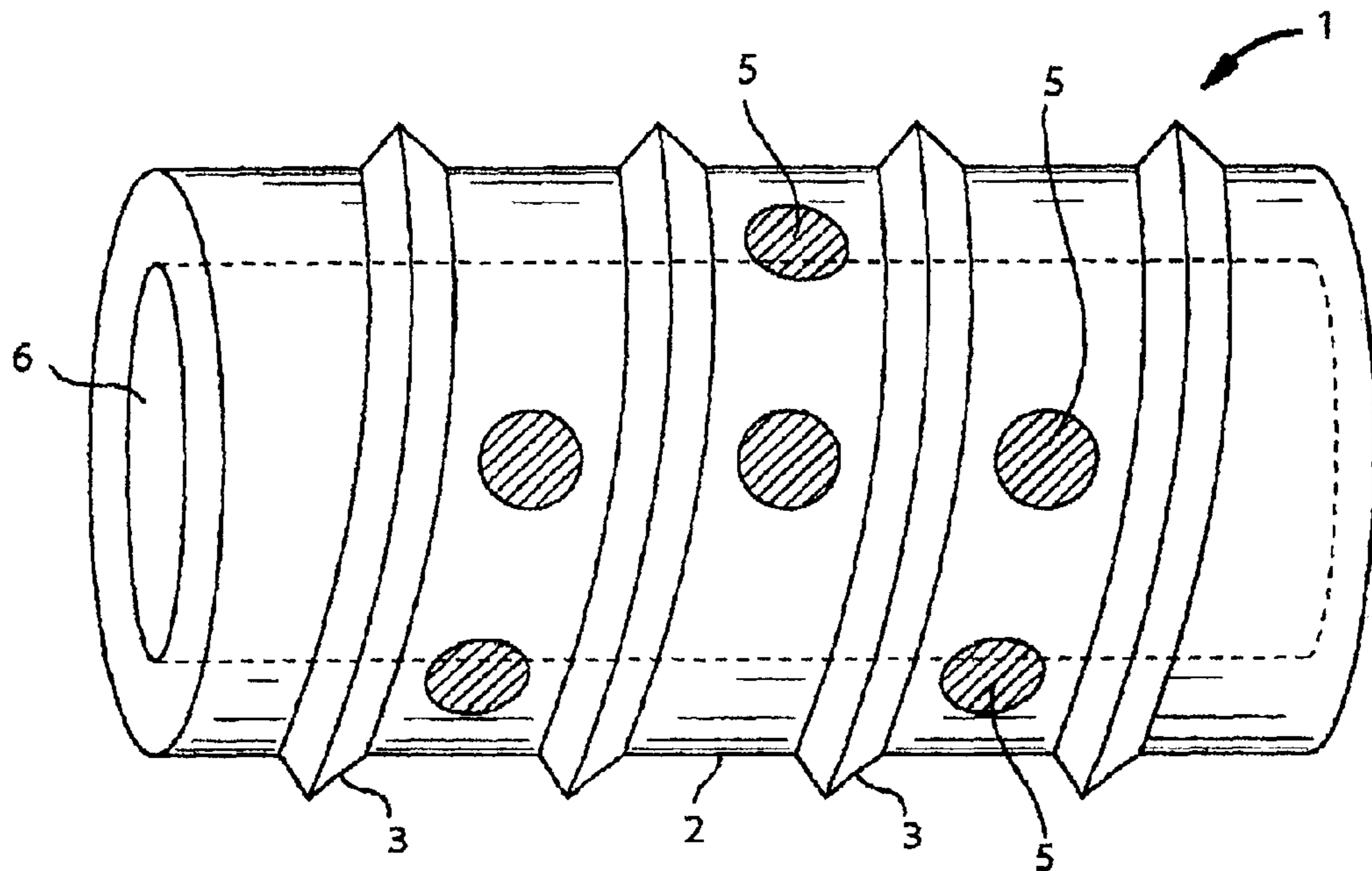
FIG. 13 (PRIOR ART)
