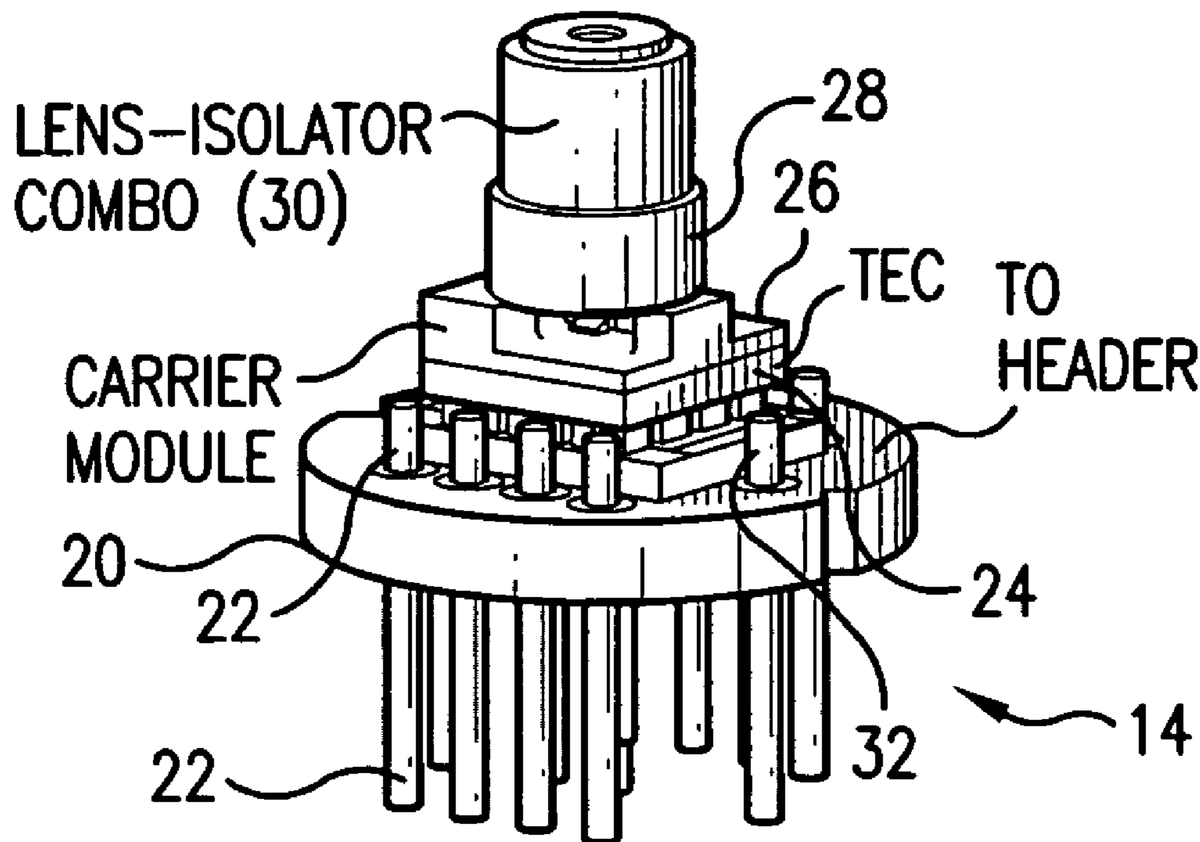
INDIVIDUAL VIEW OF TO HEADER SUBASSEMBLY AND SEALING CAP
