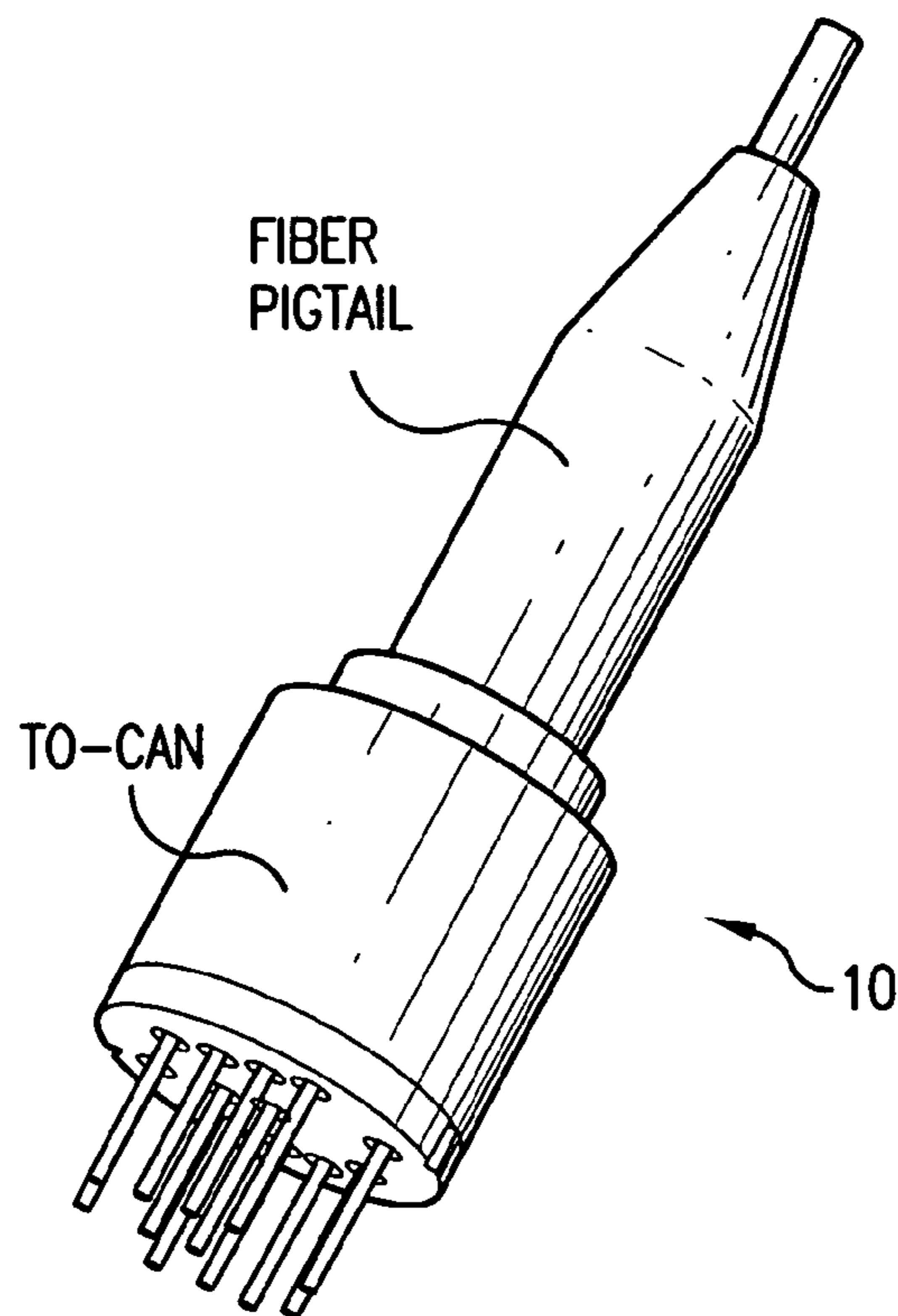
COMPLETED LASER MODULE FIG. 1
