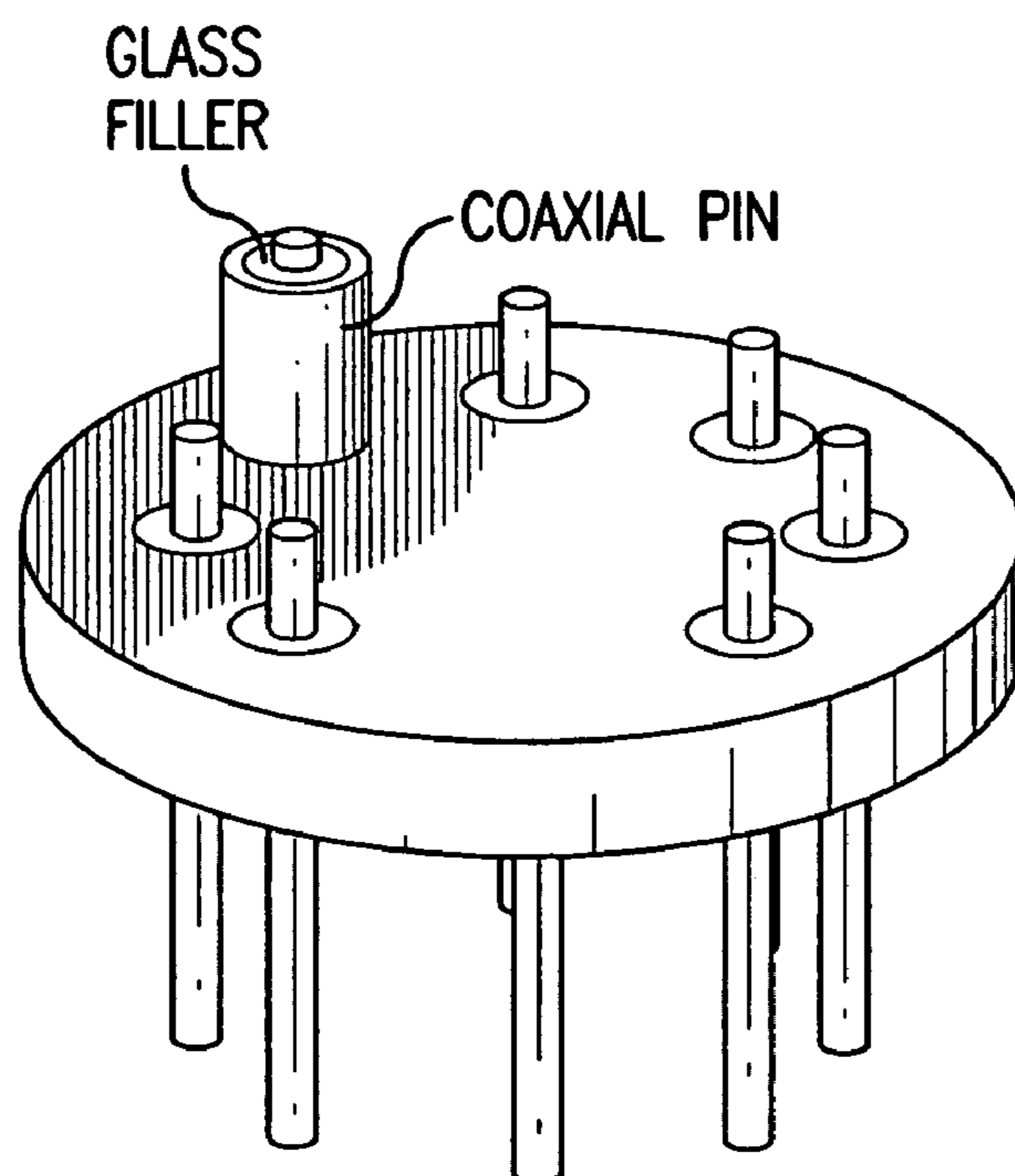
TO HEADER WITH CIRCULAR PIN CONFIGURATION
