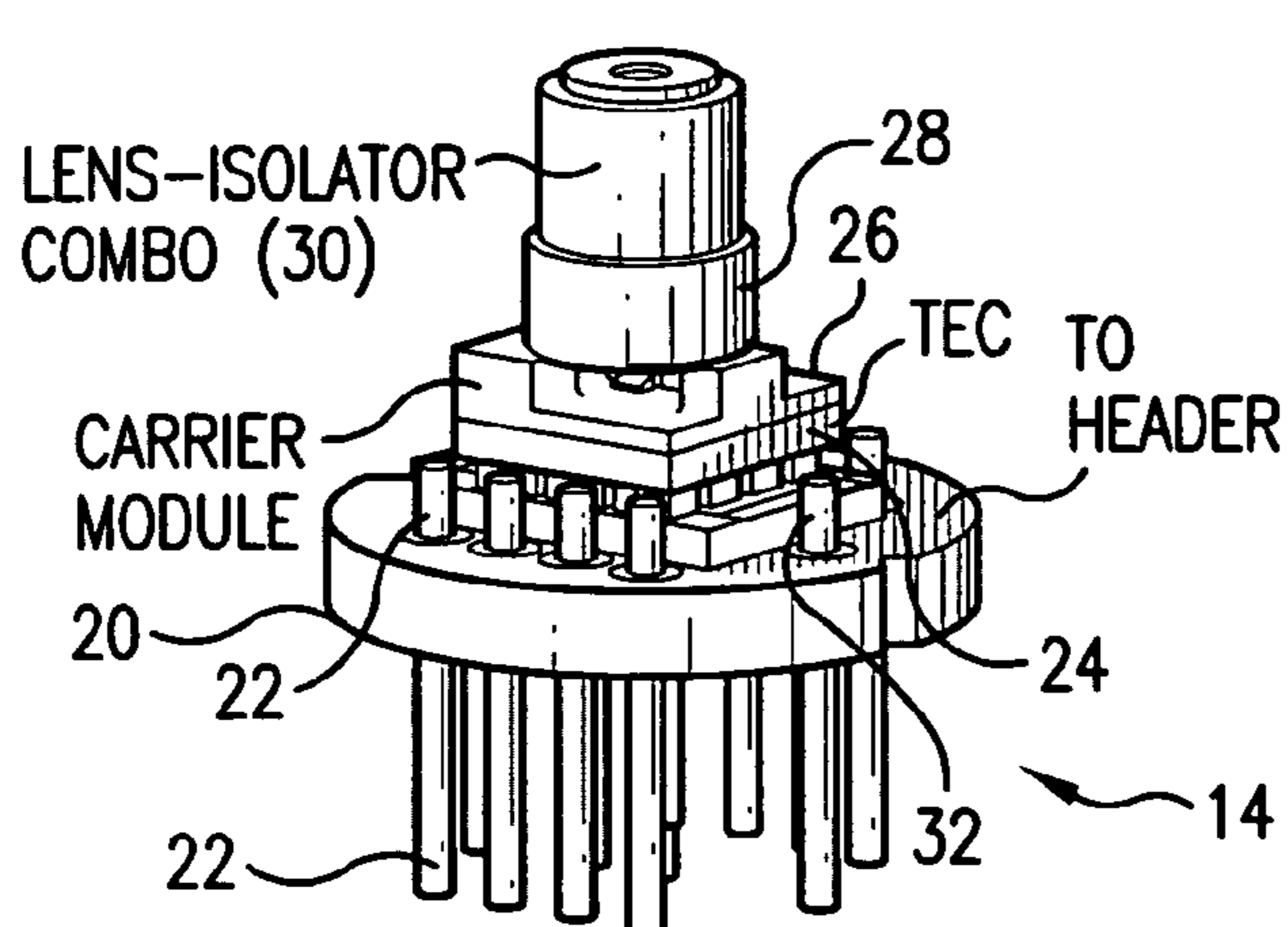
INDIVIDUAL VIEW OF TO HEADER SUBASSEMBLY AND SEALING CAP FIG. 2a
