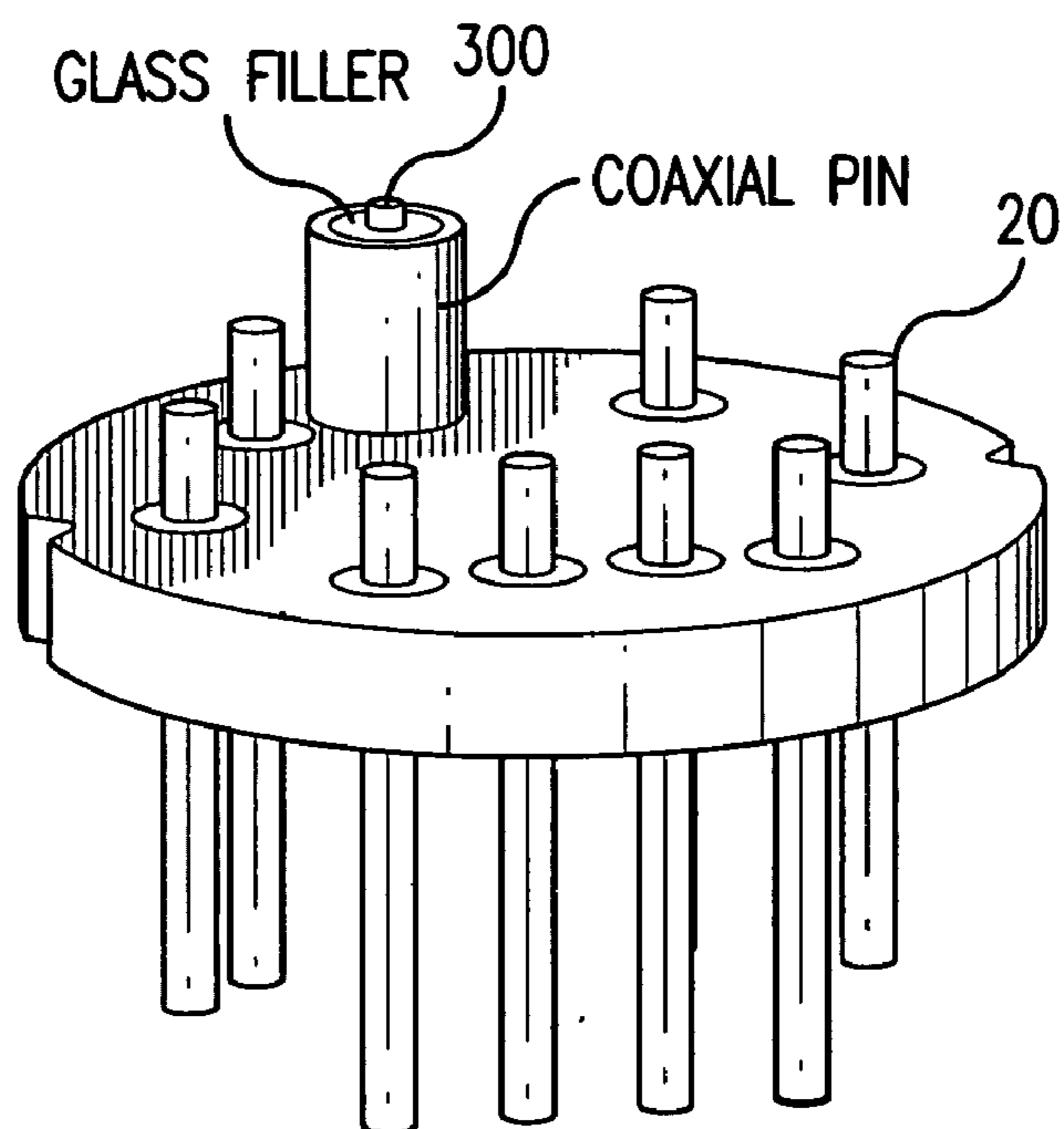
TO HEADER WITH INLINE PIN CONFIGURATION
