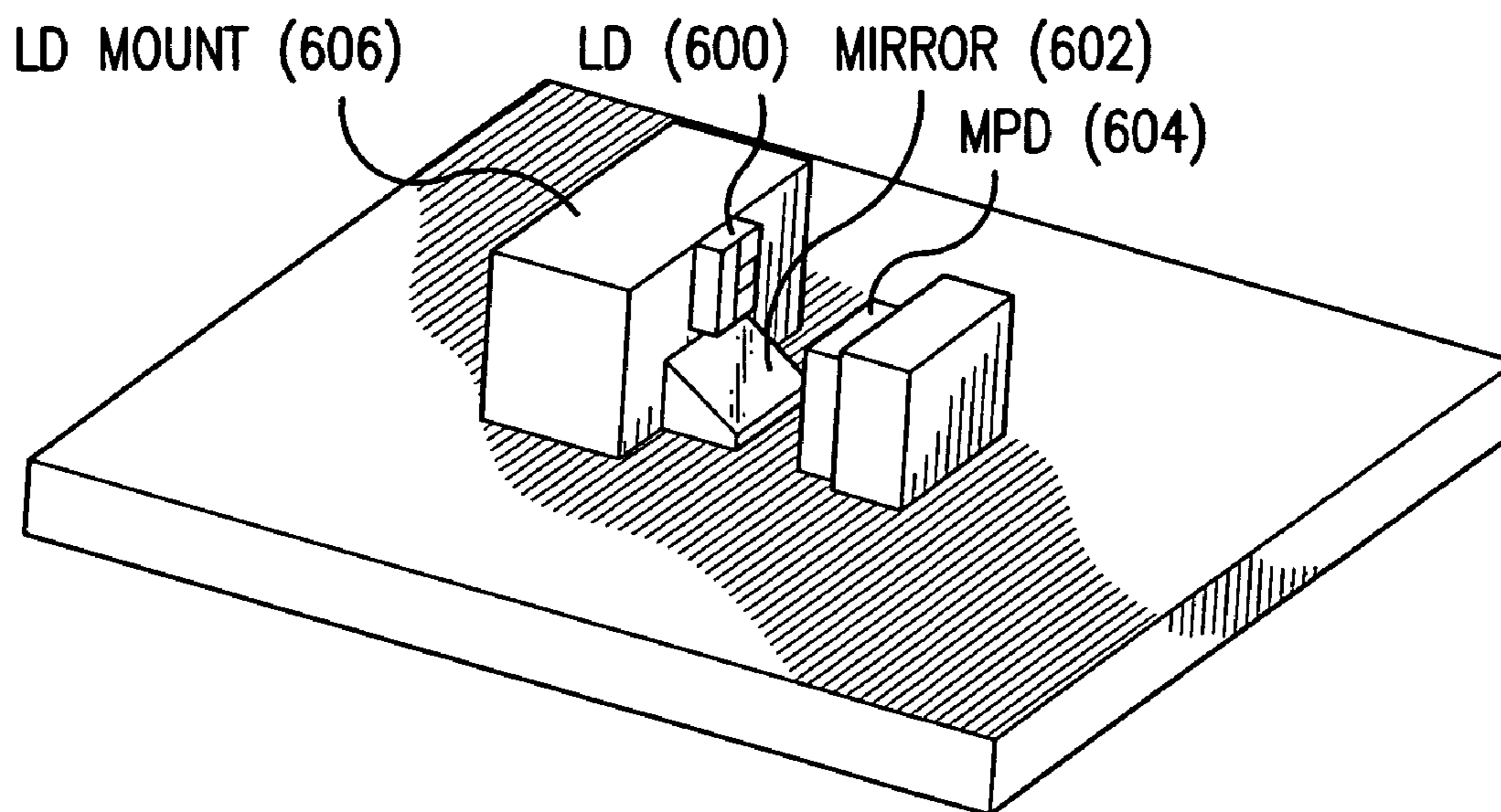
COMPACT LD-MPD PLACEMENT FIG. 6
