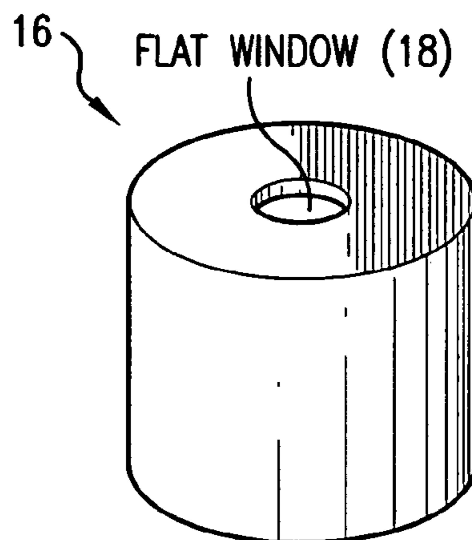
INDIVIDUAL VIEW OF TO HEADER SUBASSEMBLY AND SEALING CAP FIG. 2b
