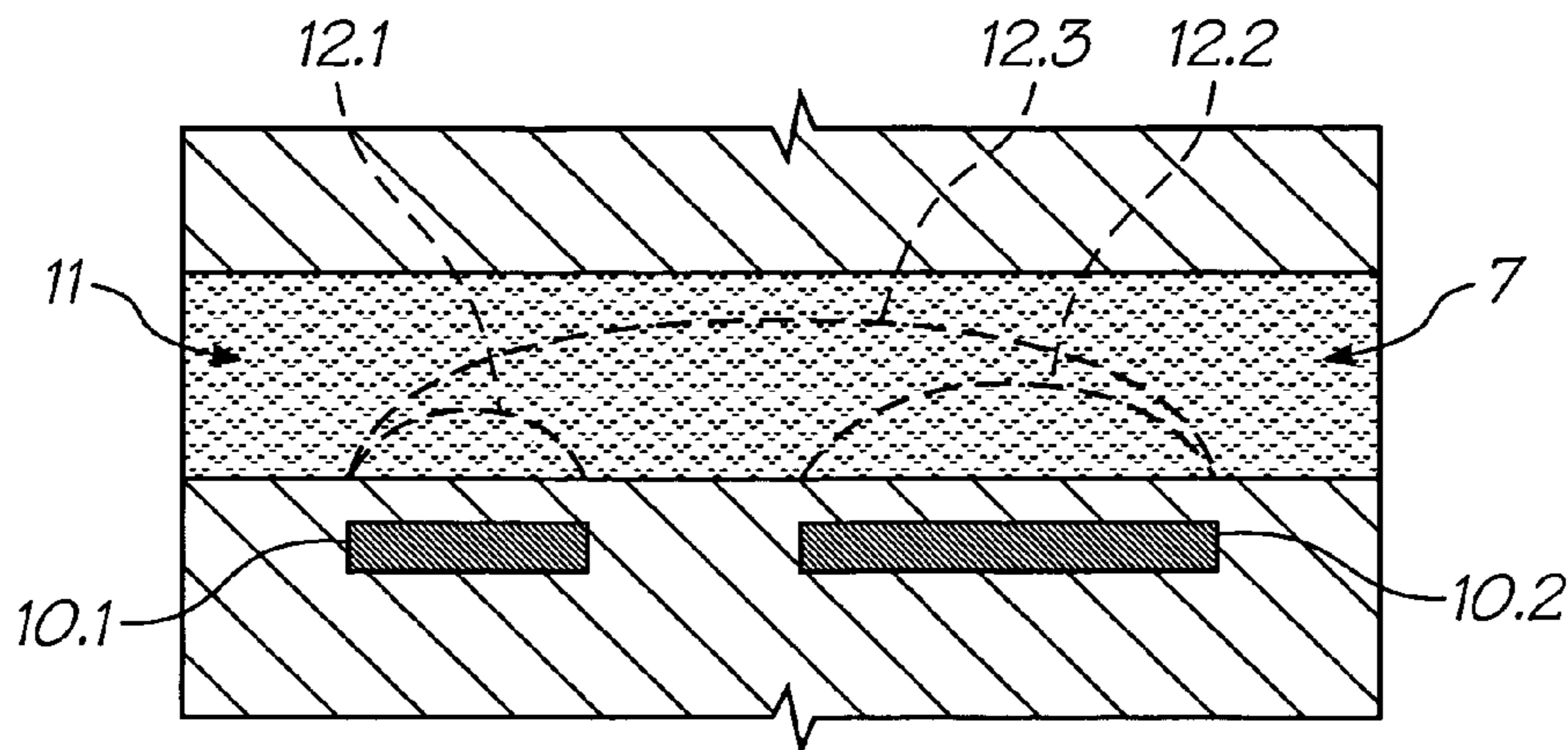
FIG. 52 (PRIOR ART)
