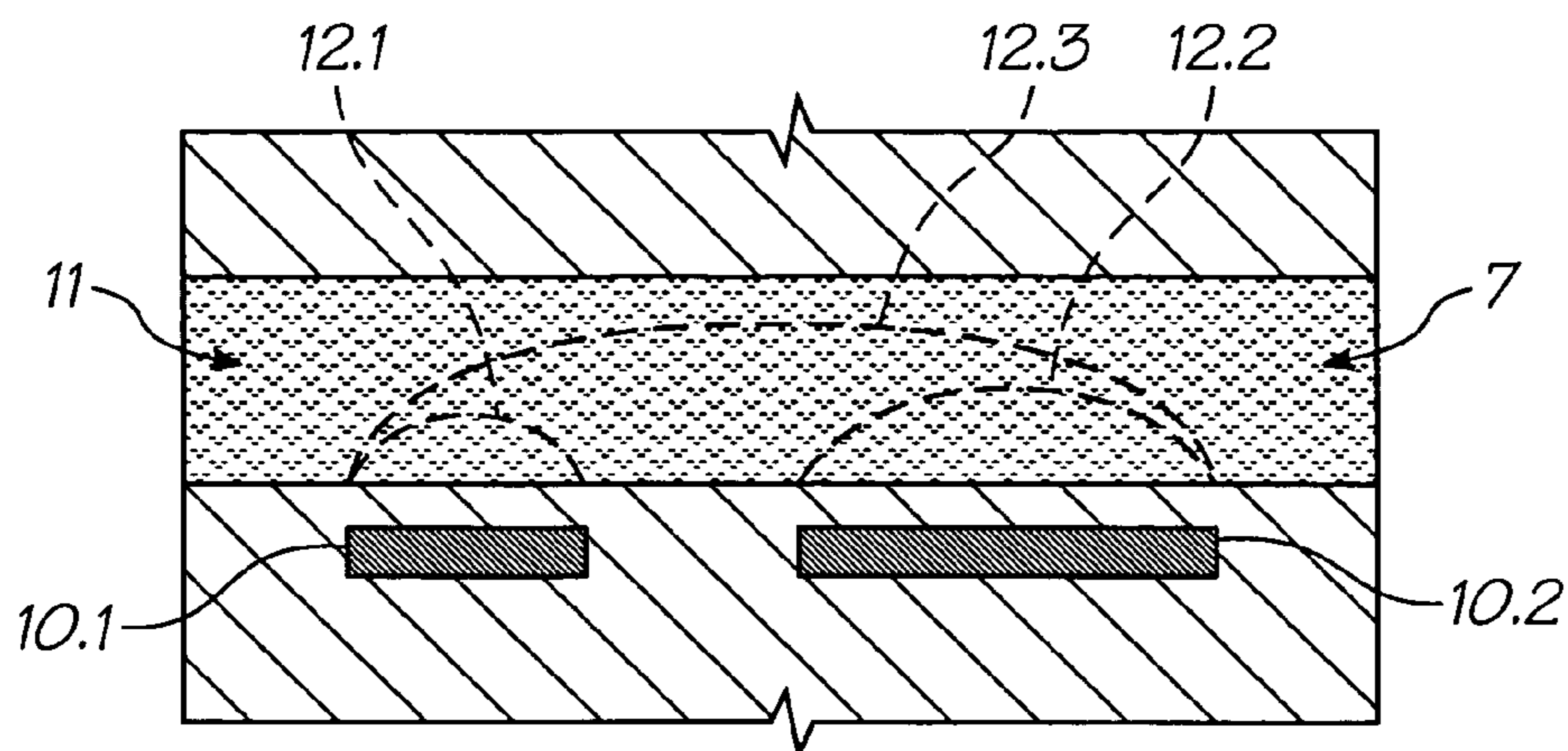
FIG. 52 (PRIOR ART)
