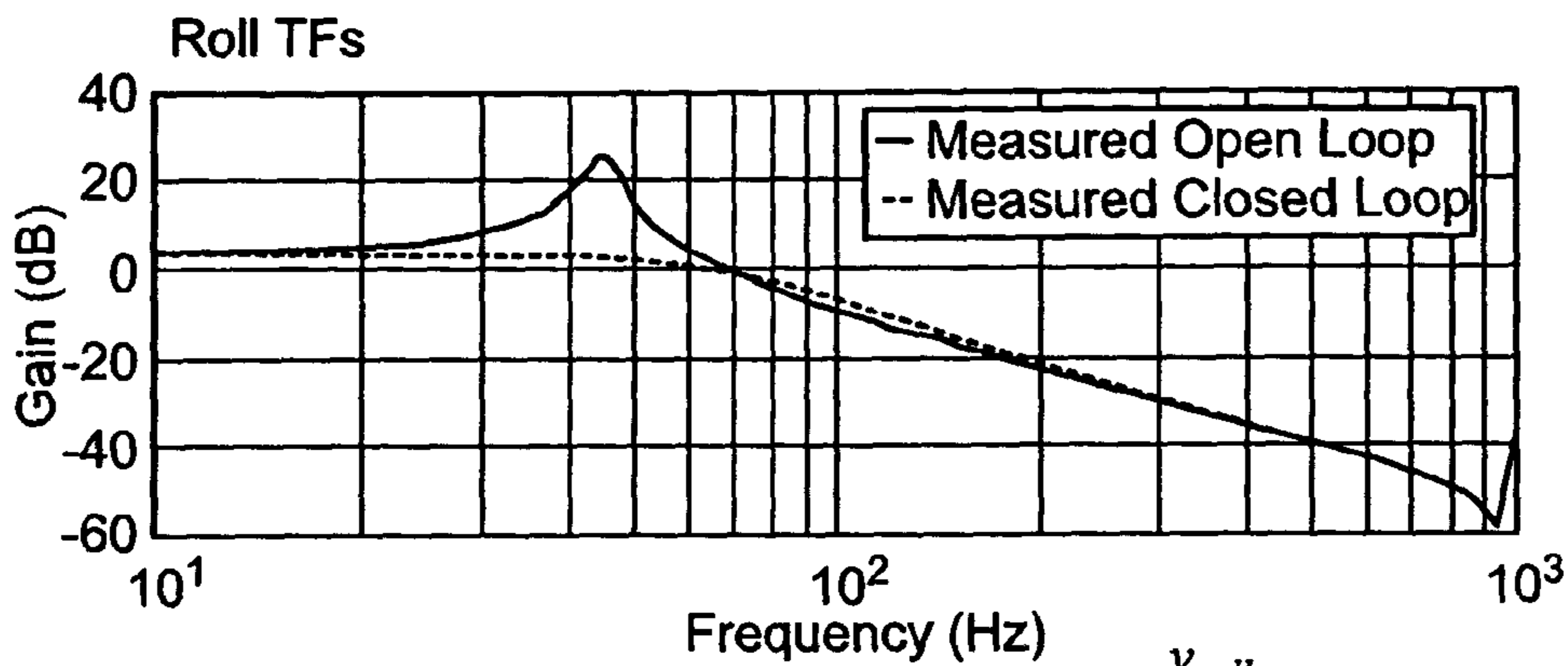
Roll mode transfer functions, \frac{y_{roll}}{u_{roll}} FIG. 25A
