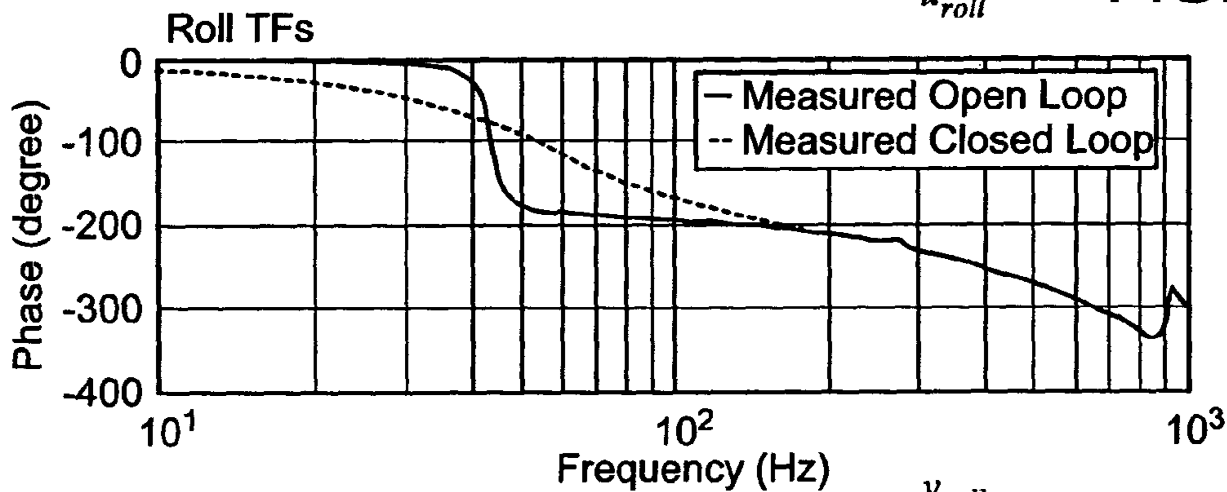
Roll mode transfer functions, \frac{y_{roll}}{u_{roll}} FIG. 25B
