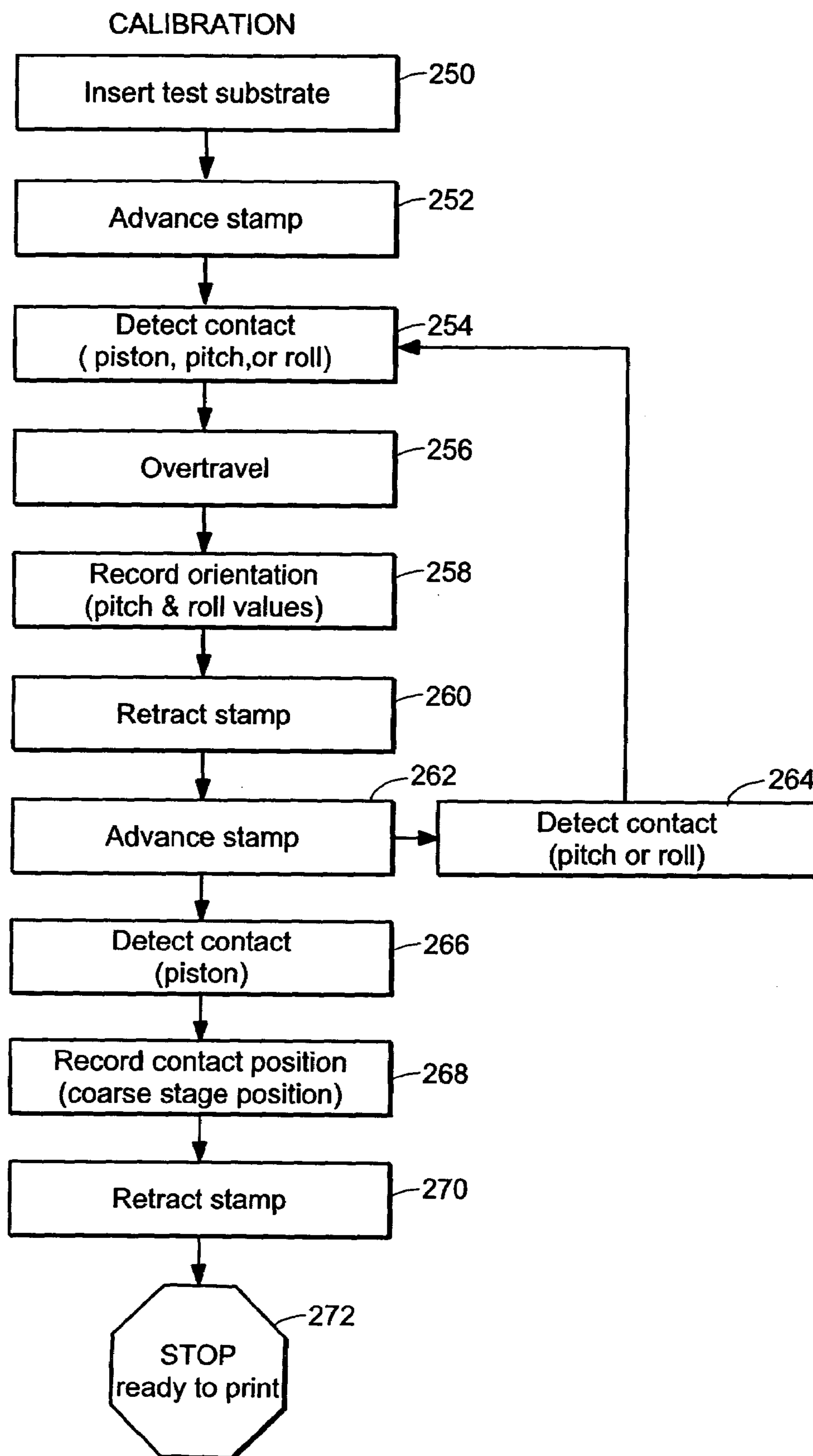
Calibration algorithm
