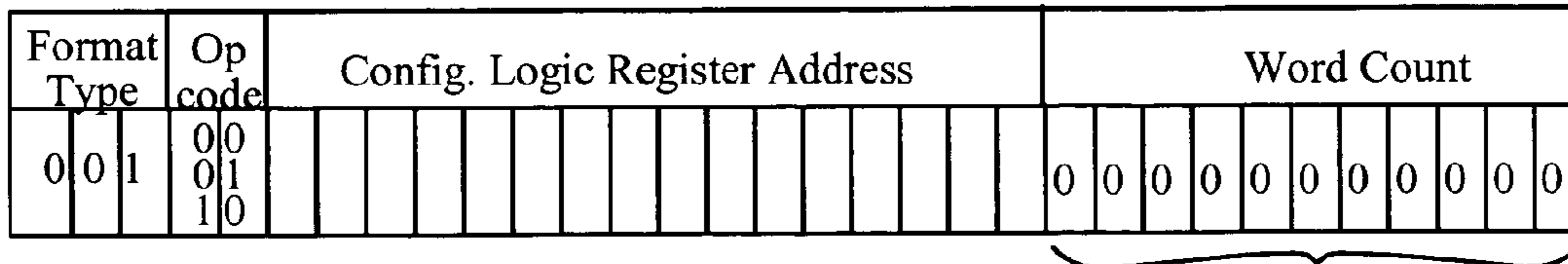
32-bit Command Header Format 2
