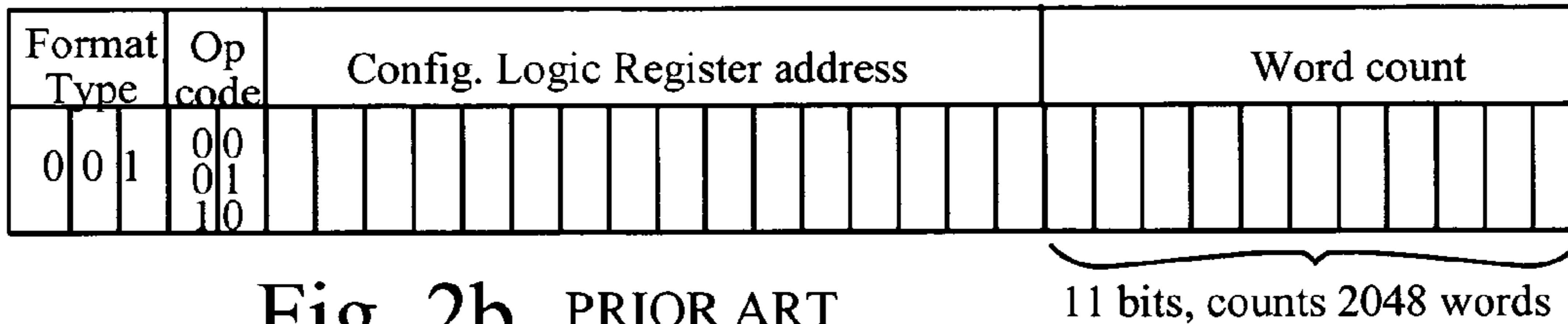
32-bit Command Header Format 1
