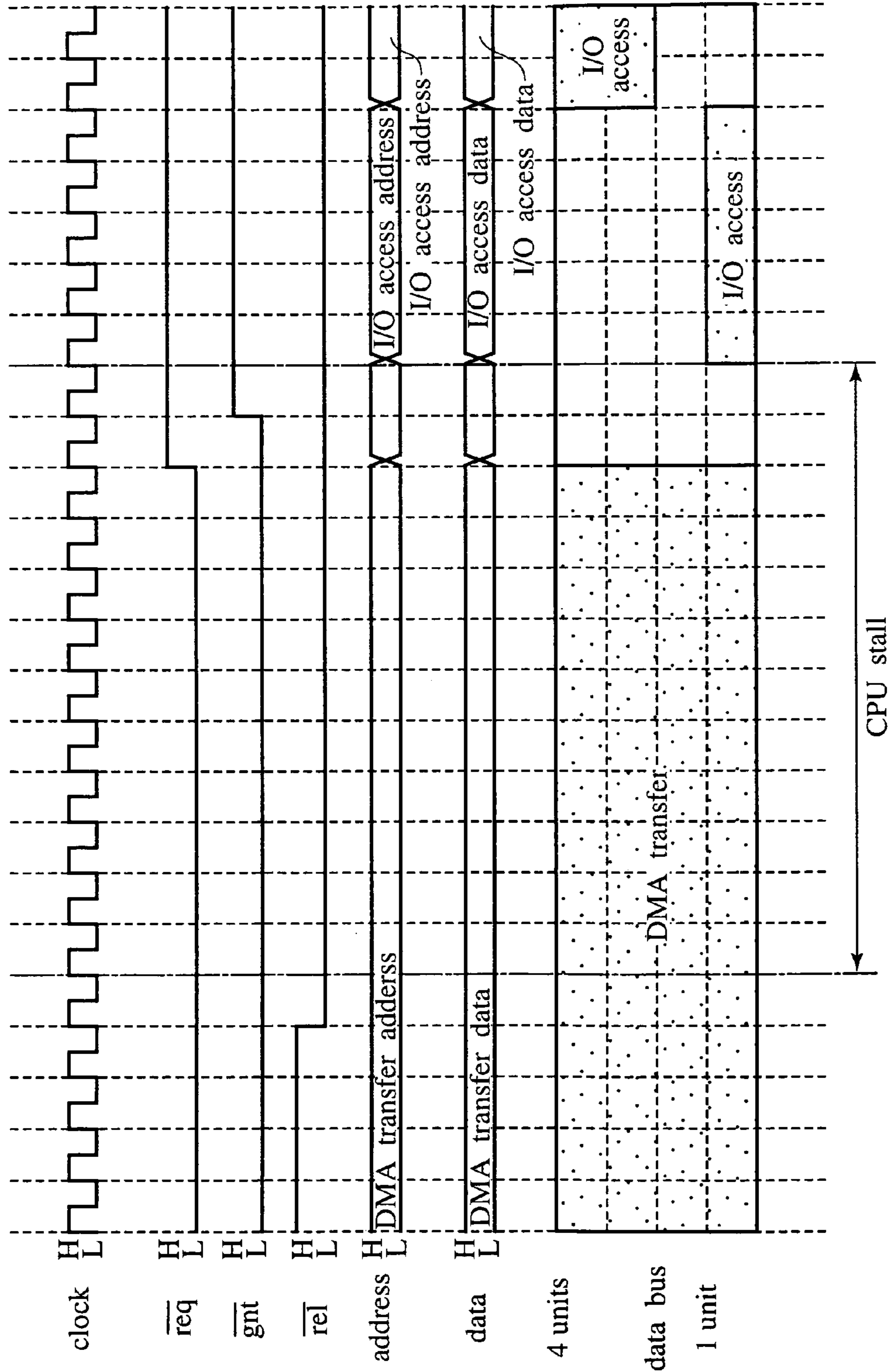
FIG. 4 PRIOR ART
