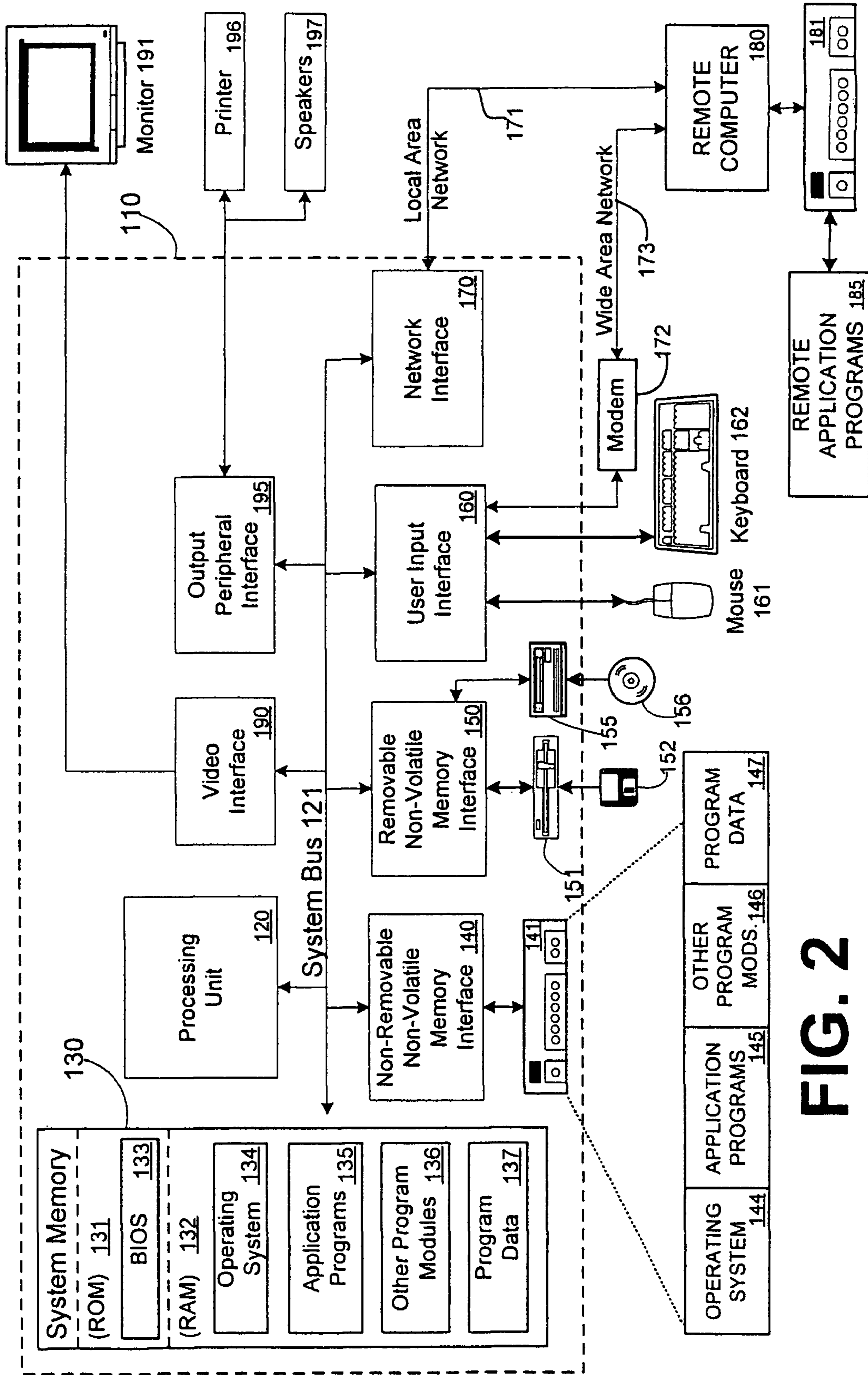
Computing Environment 100
