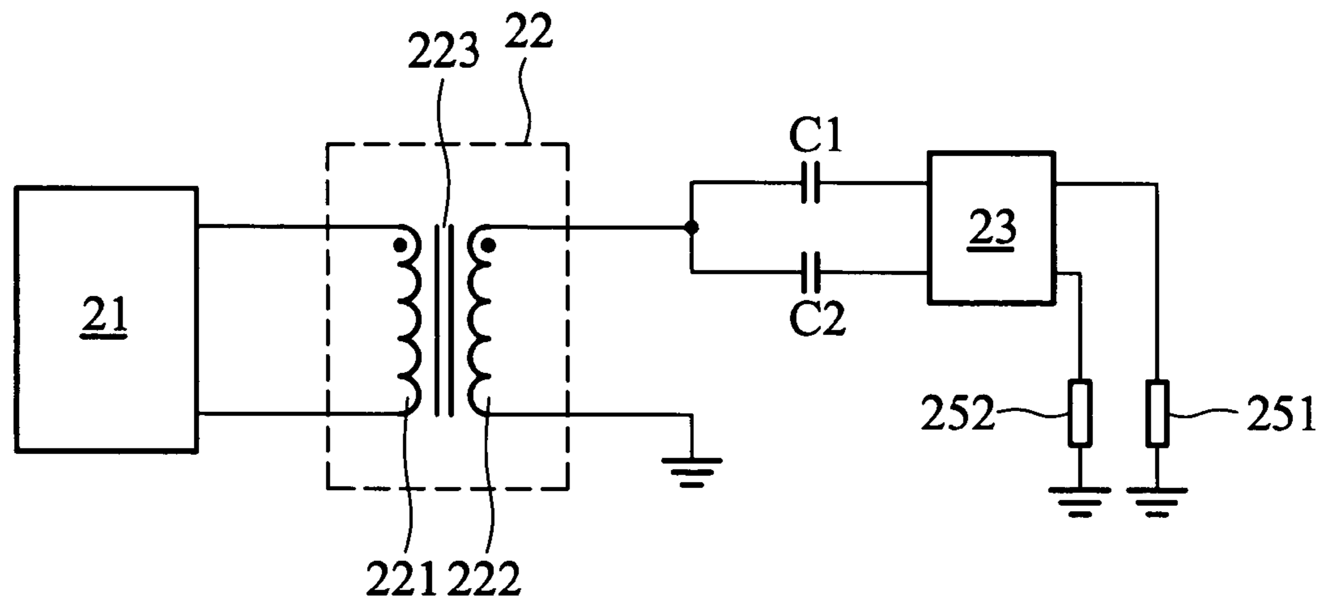
FIG. 2 (RELATED ART)
