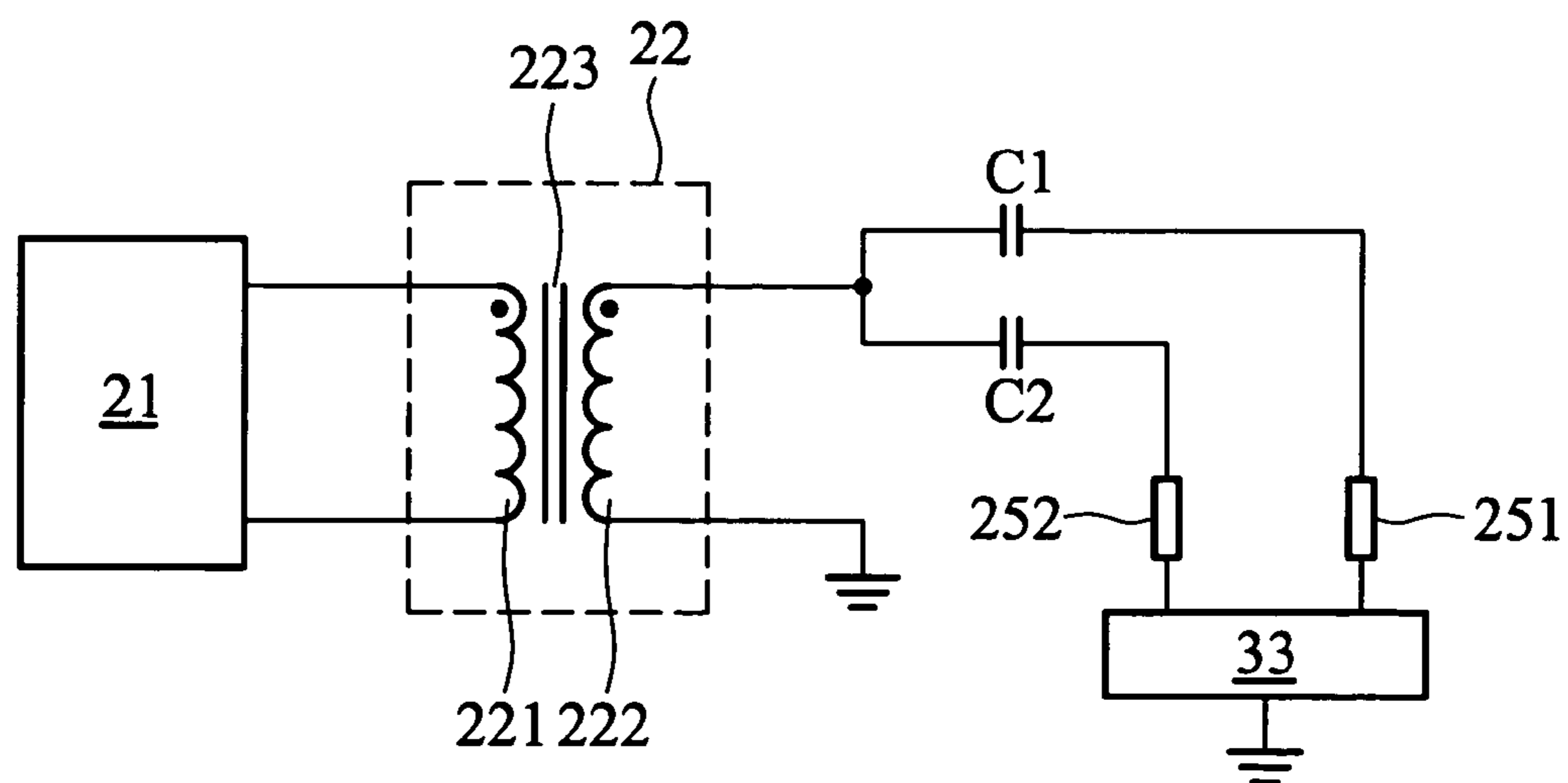
FIG. 3 (RELATED ART)
