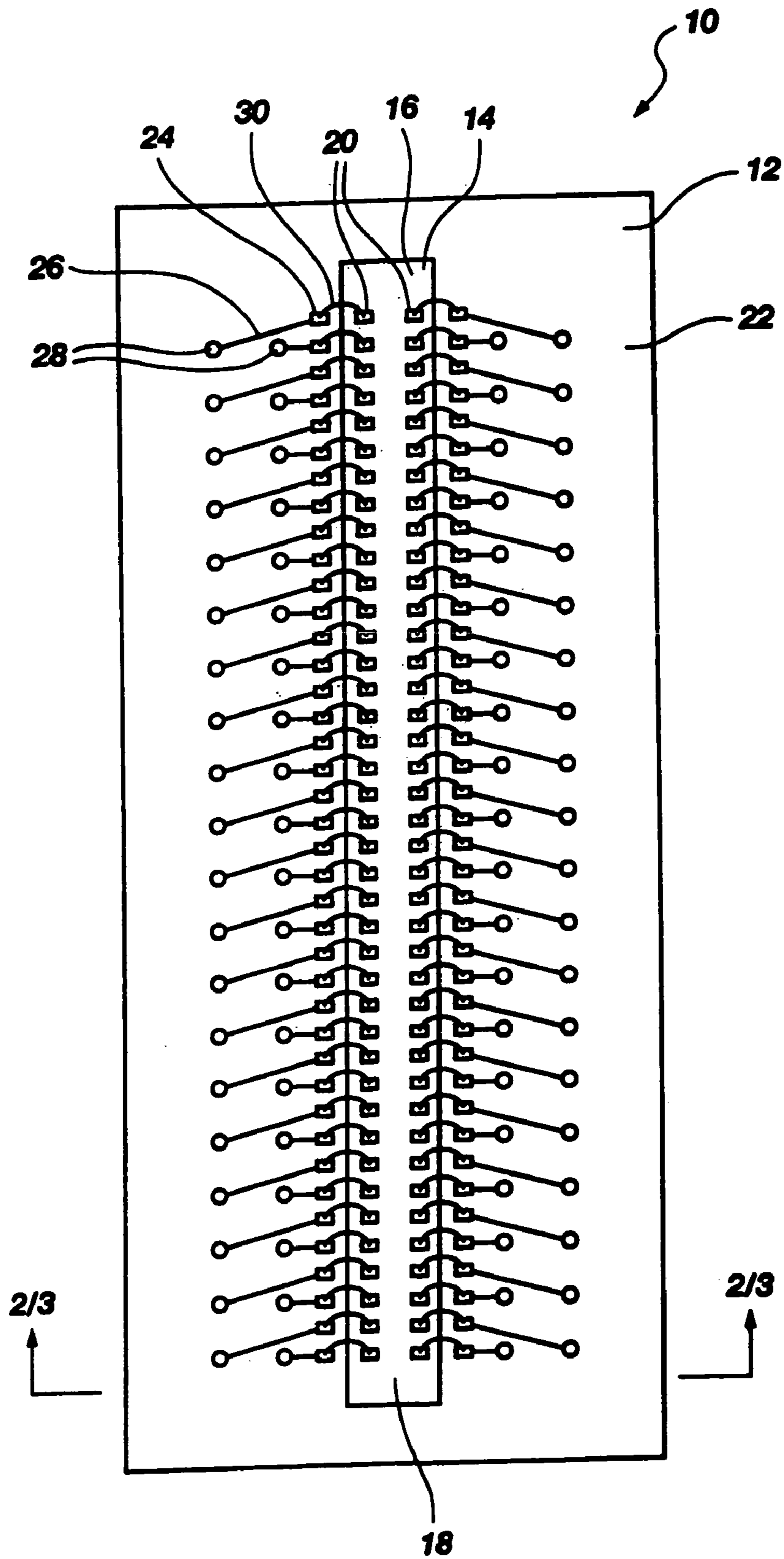
Fig. 1 (PRIOR ART)
