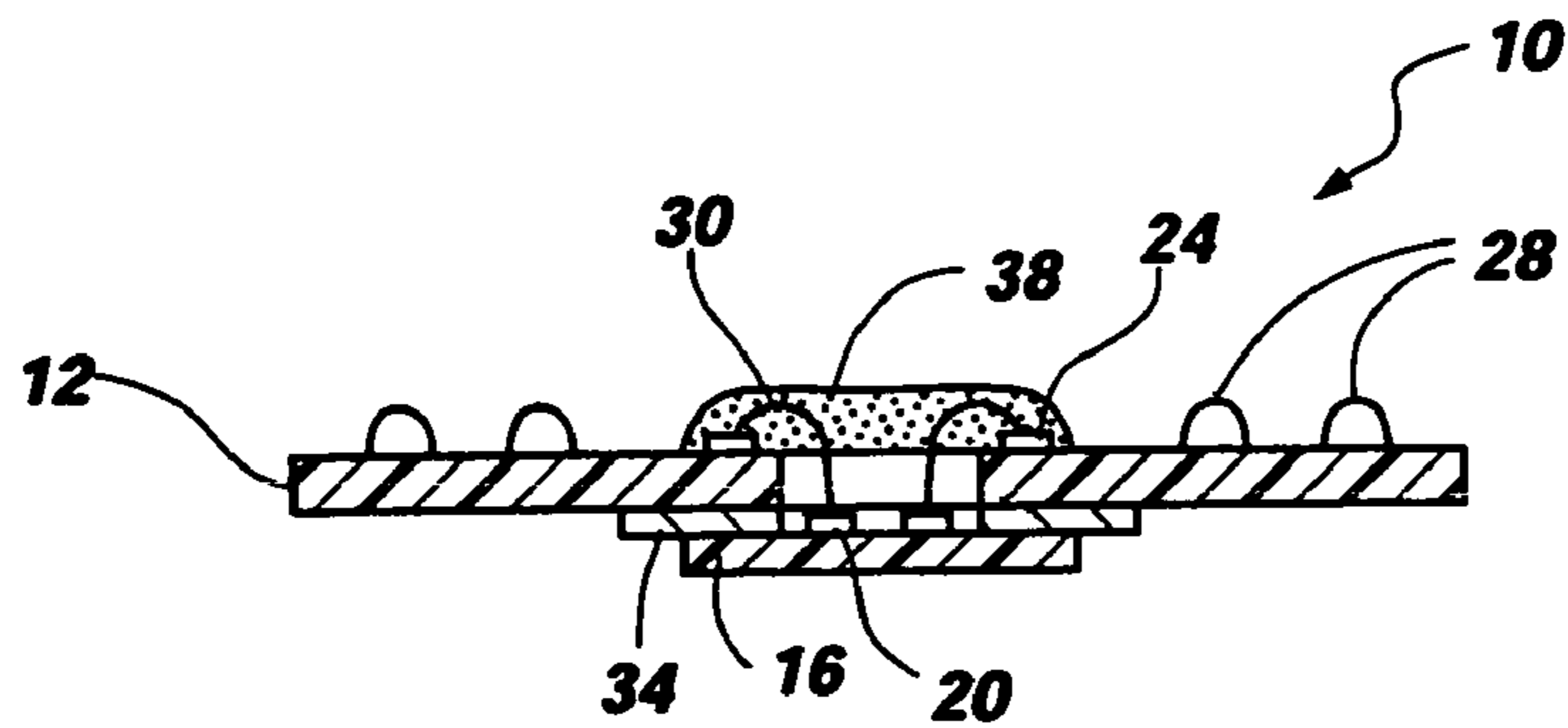
Fig. 3 (PRIOR ART)
