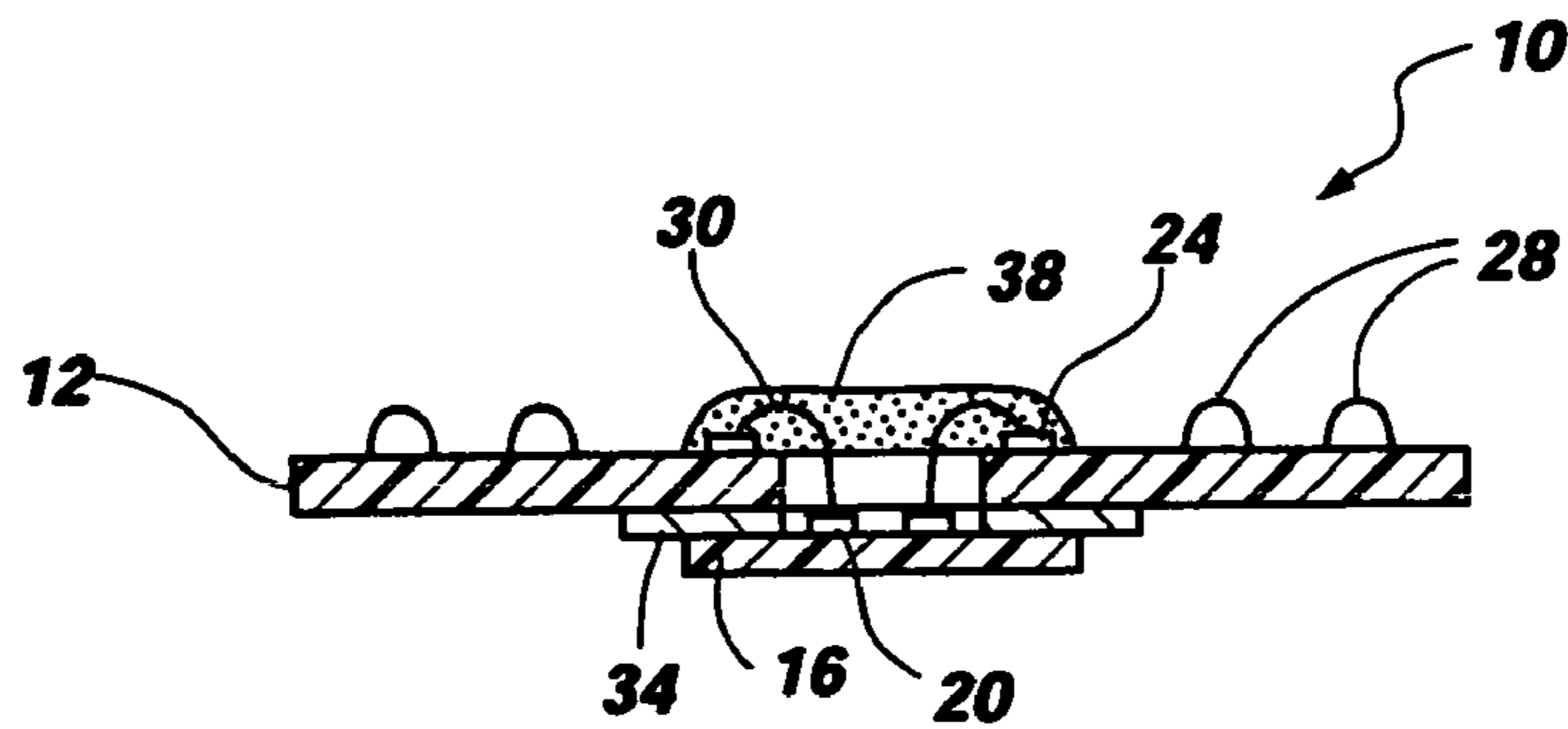
Fig. 3 (PRIOR ART)
