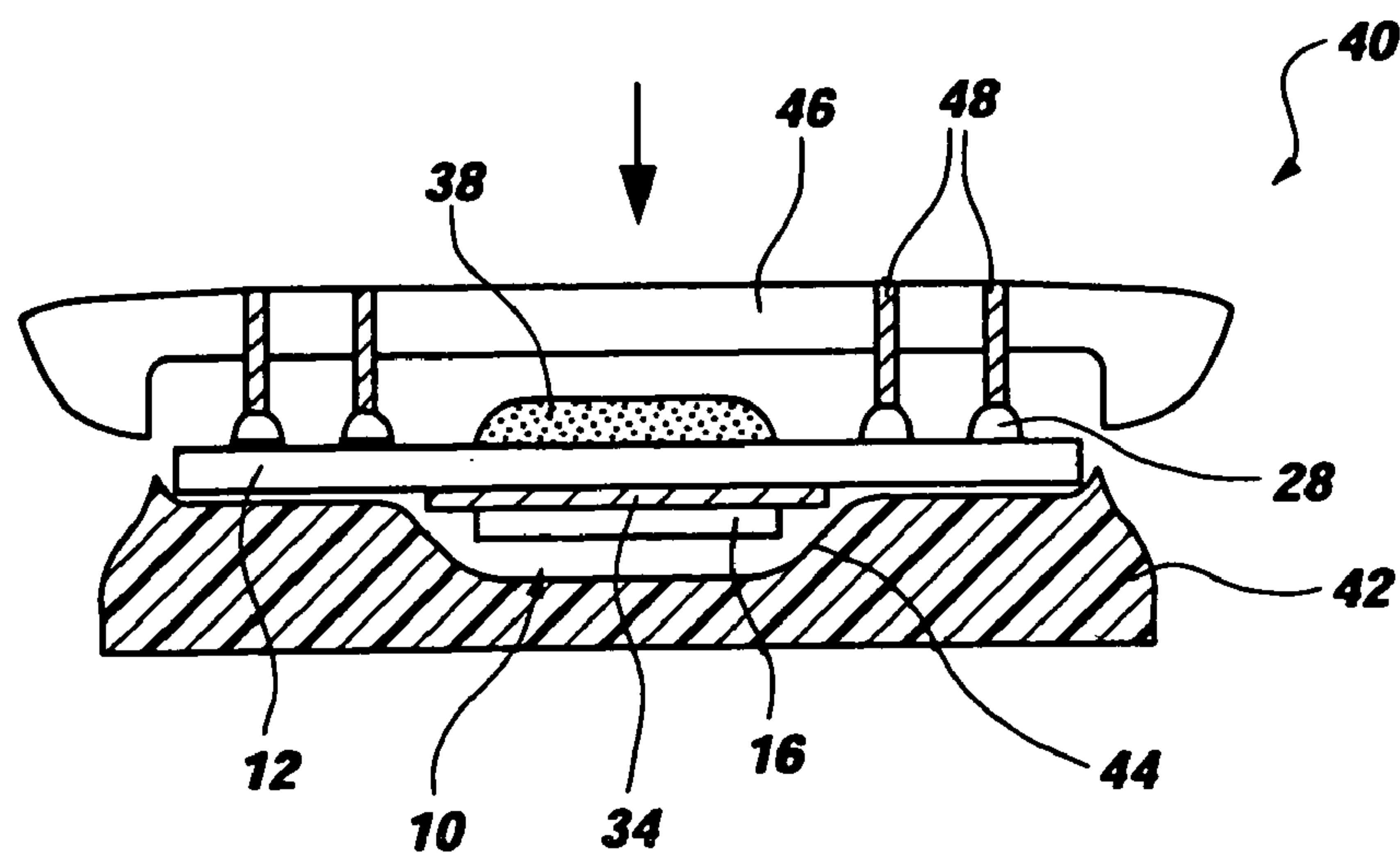
Fig. 4 (PRIOR ART)
