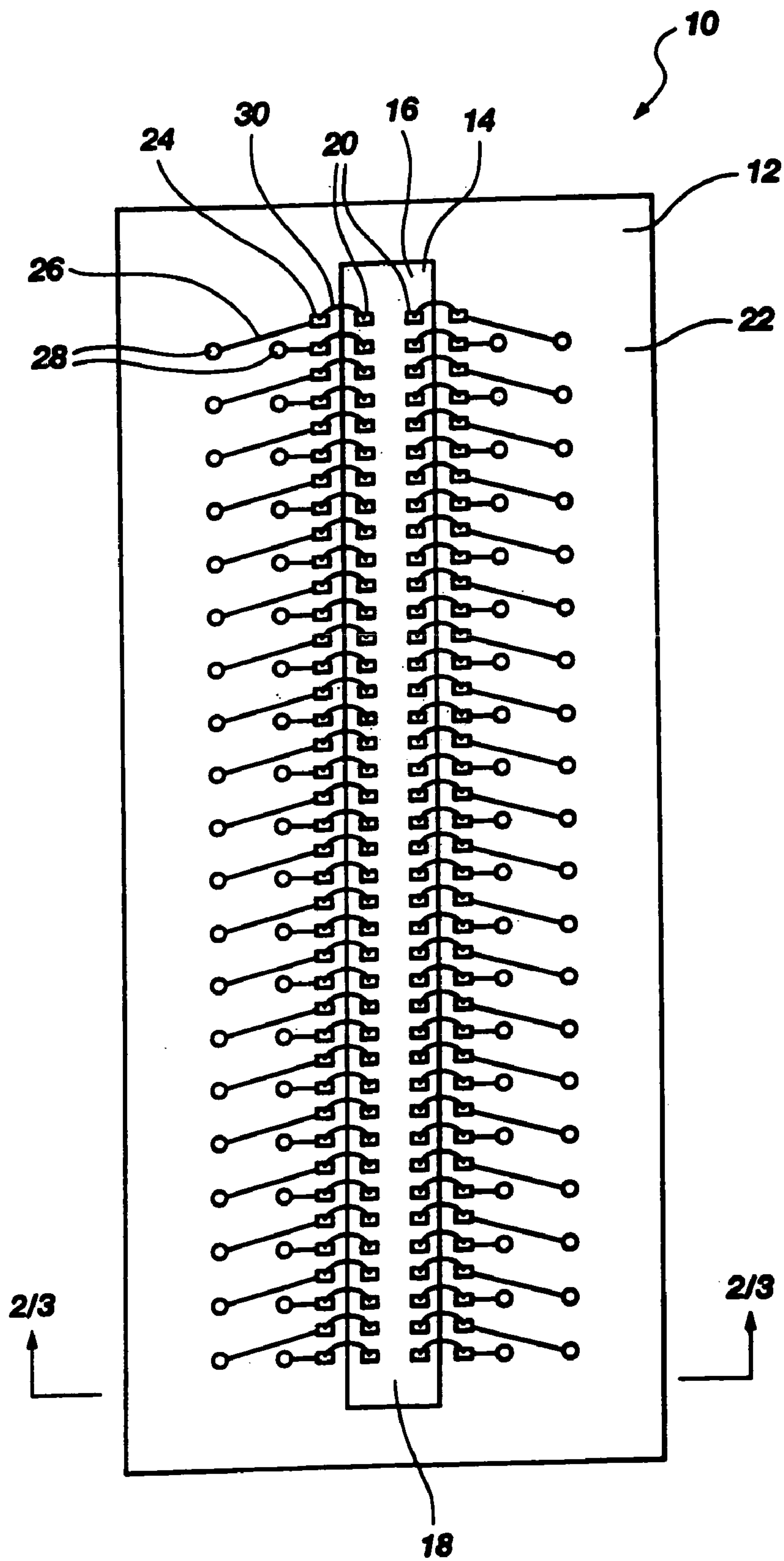
Fig. 1 (PRIOR ART)
