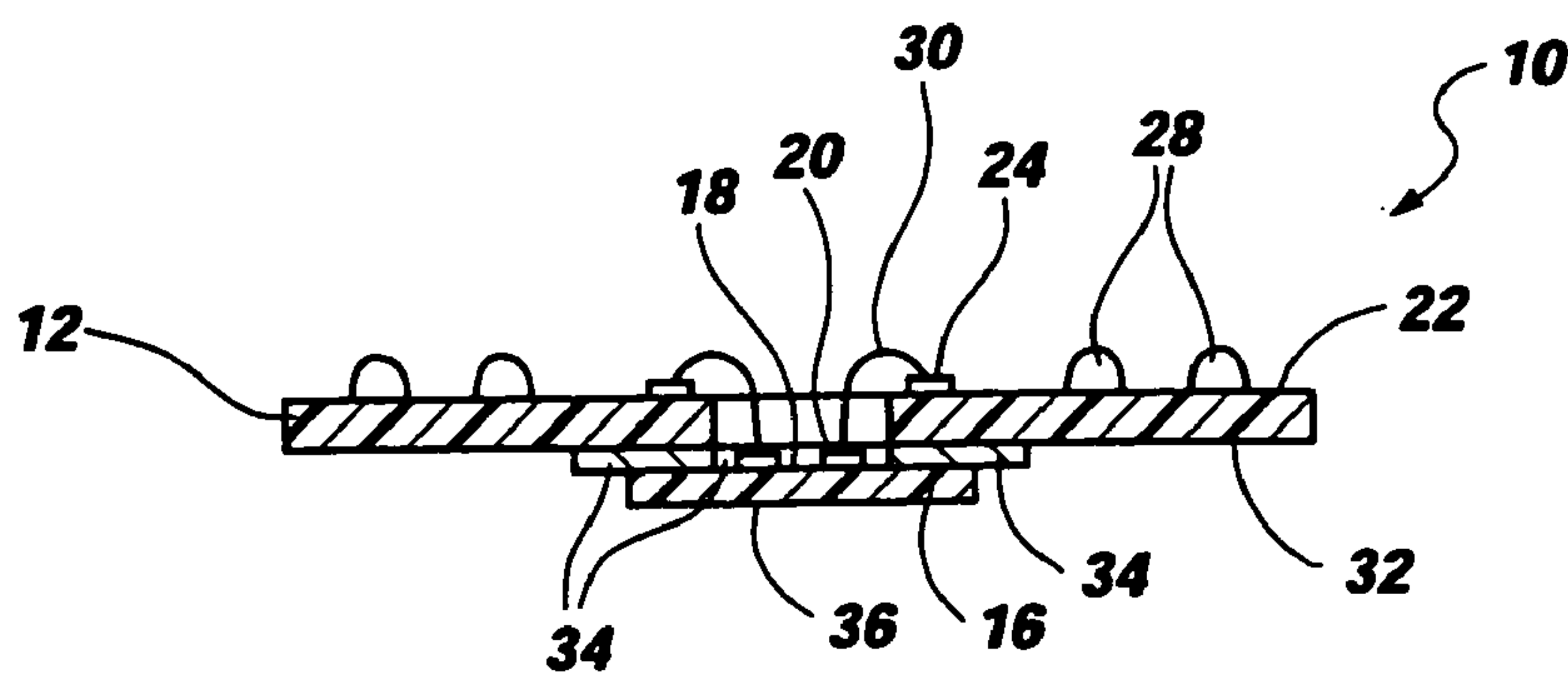
Fig. 2 (PRIOR ART)
