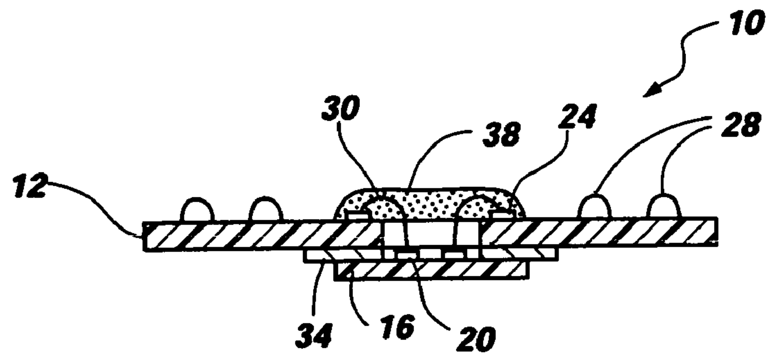
Fig. 3 (PRIOR ART)
