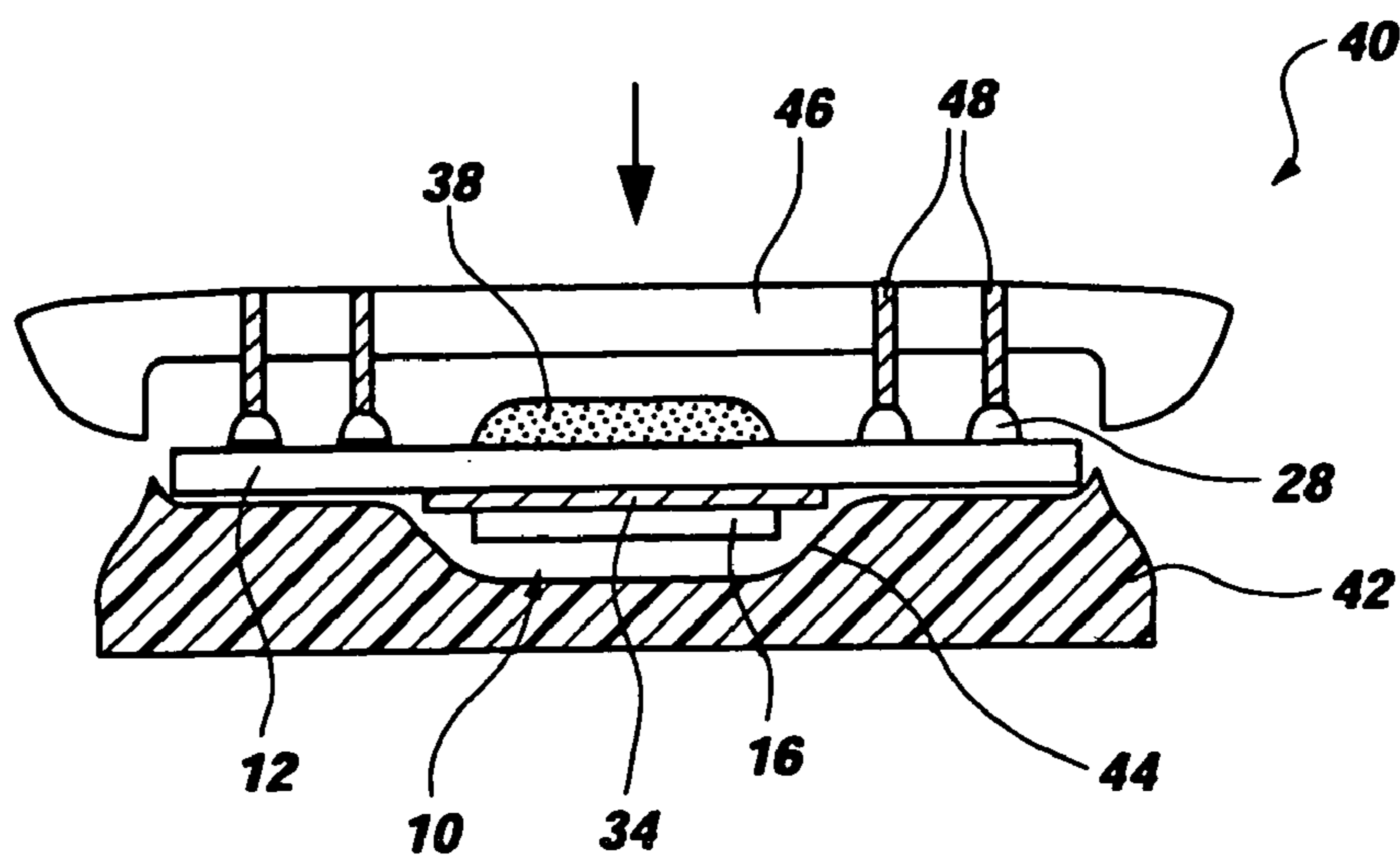
Fig. 4 (PRIOR ART)
