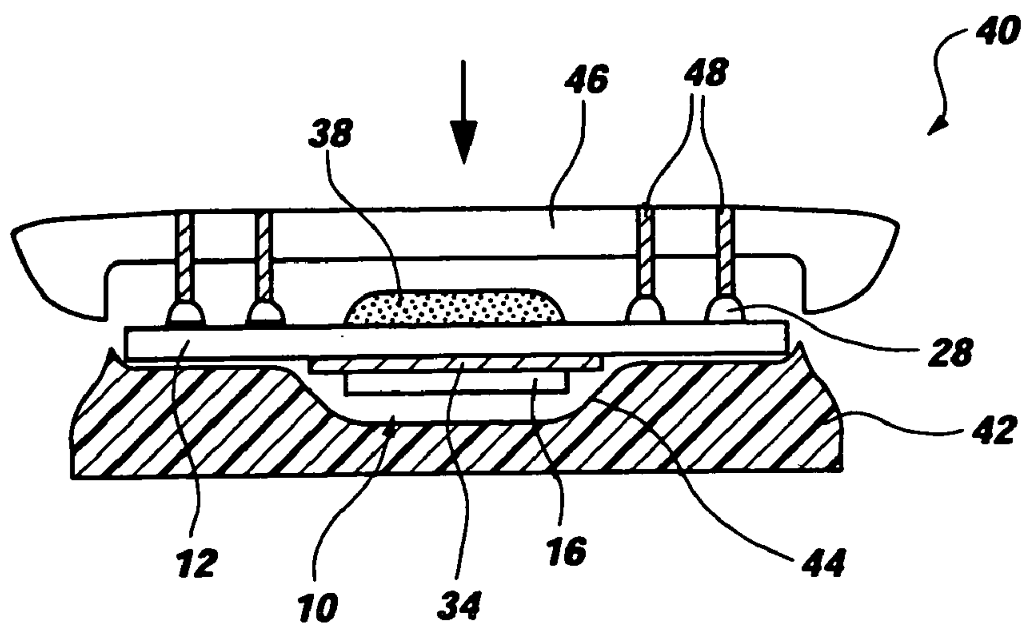
Fig. 4 (PRIOR ART)
