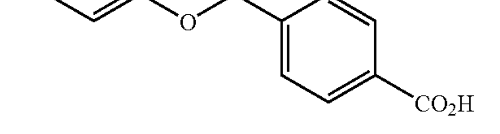
Compound A
