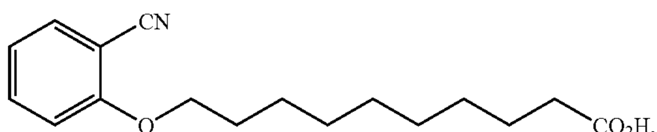
Compound 7
