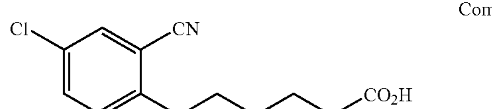
Compound 8
