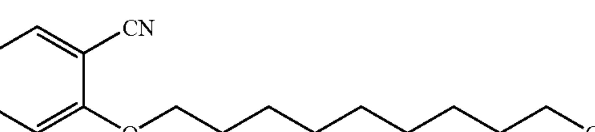
Compound 7
