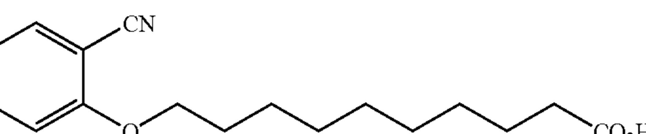
Compound 7
