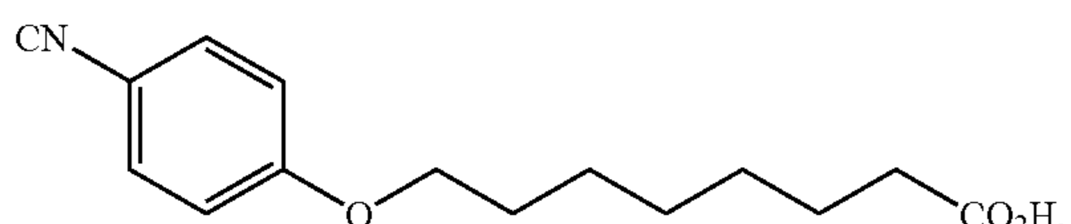
Compound 9
