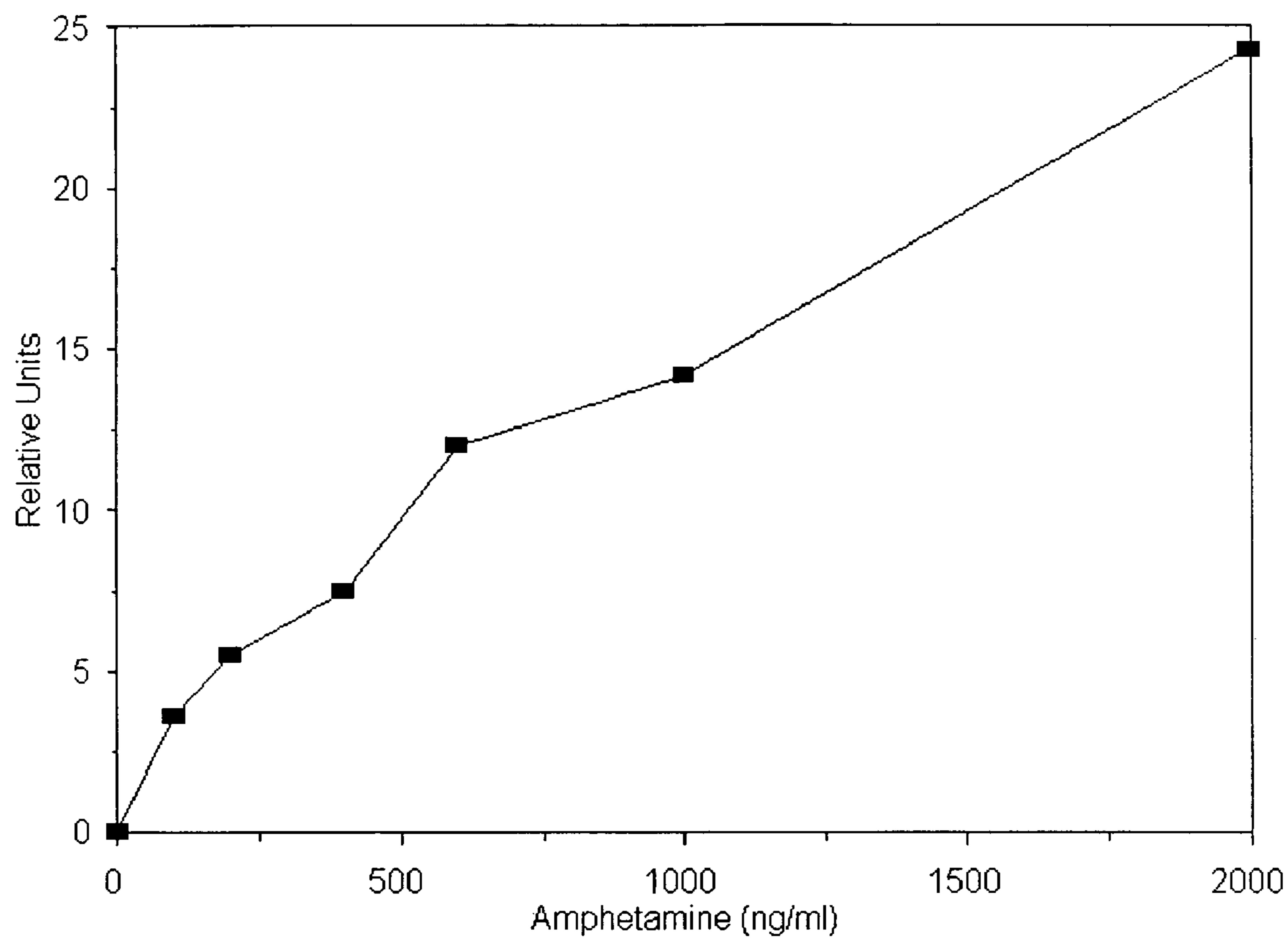
Standard Curve for Amphetamine with Bivalent Hapten/Enzyme Conjugate and Amphetamine Antibody
