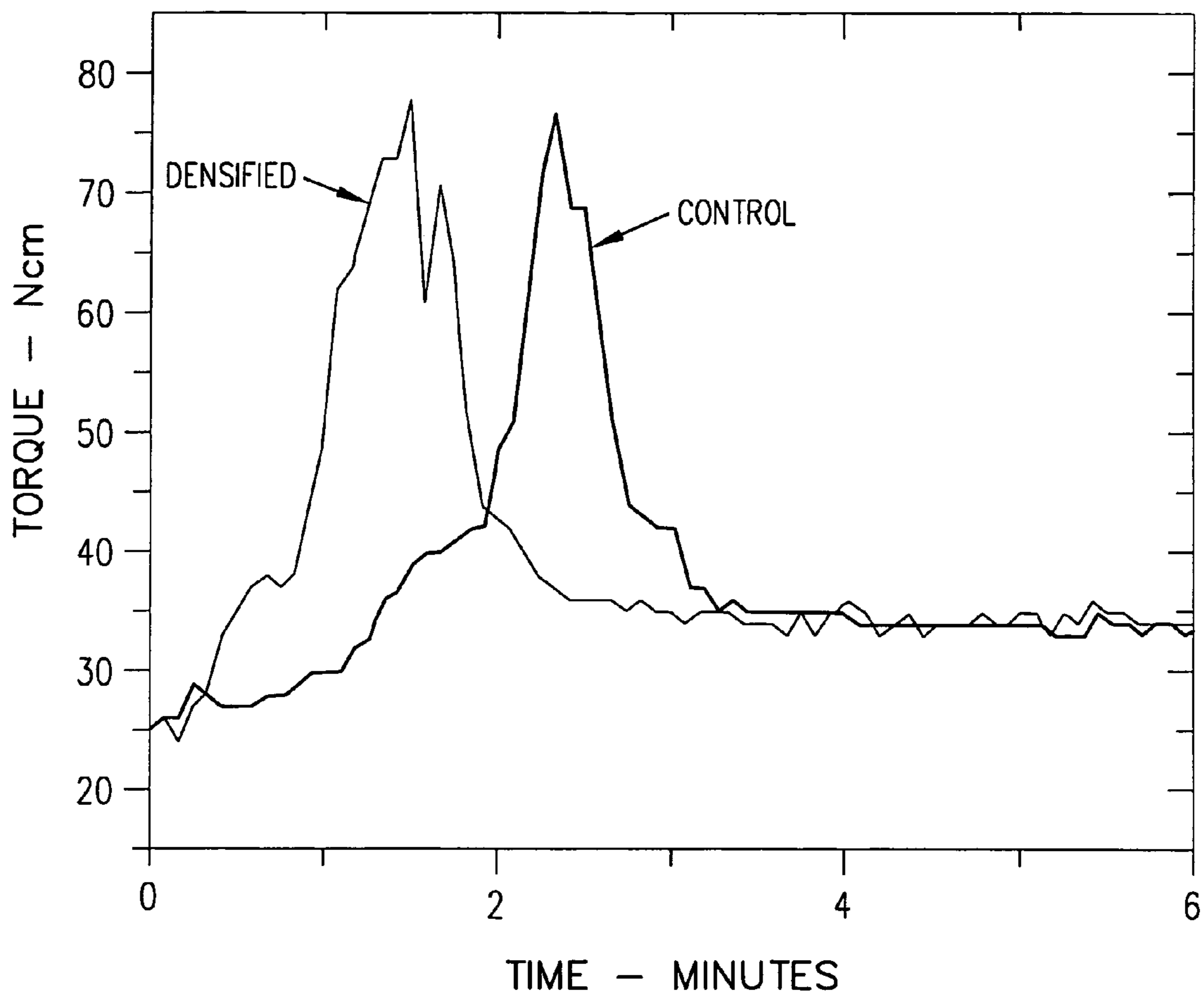
'WET-IN' TIME VERSUS TORQUE
