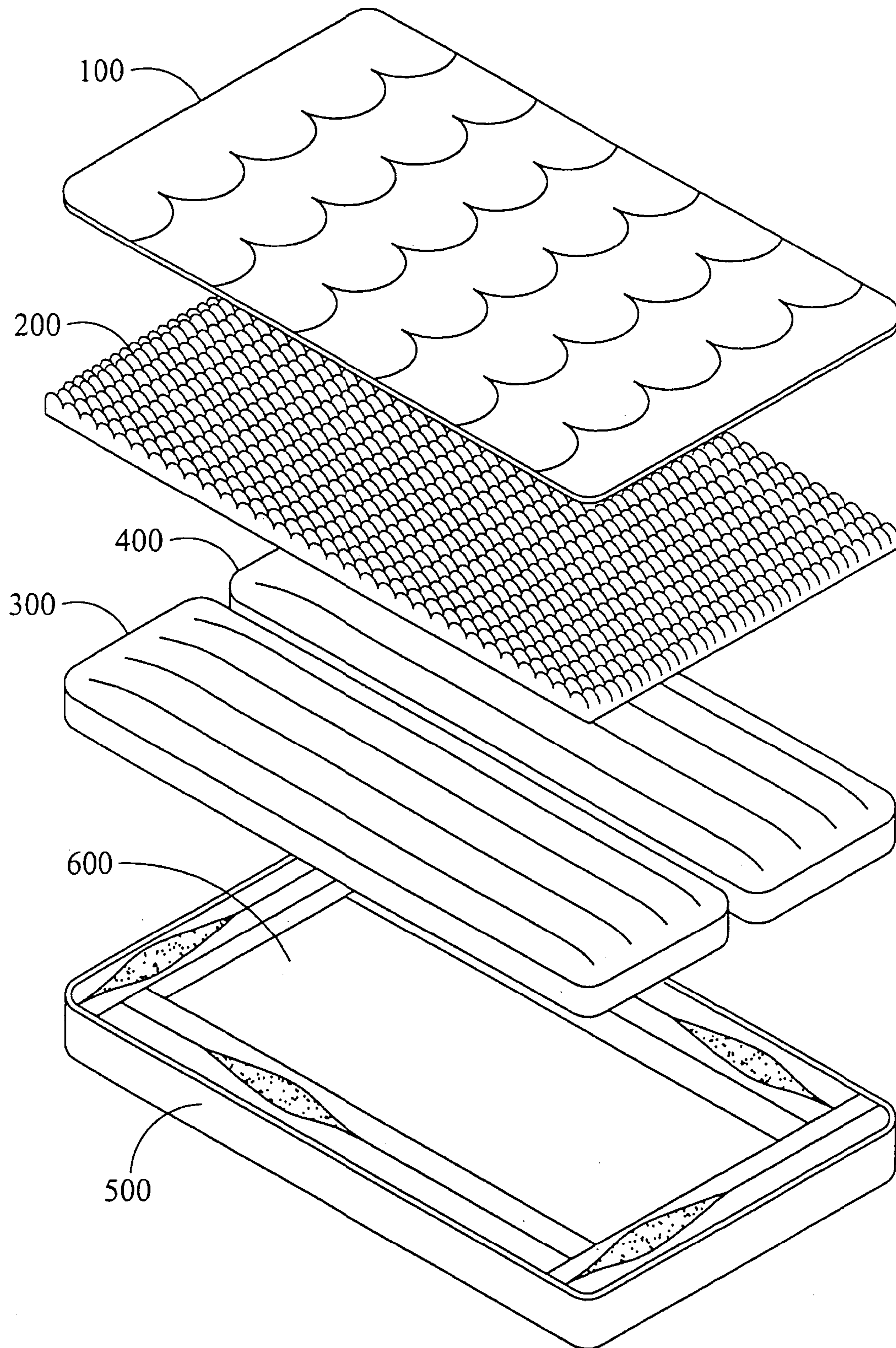
FIG. 11 ( PRIOR ART )
