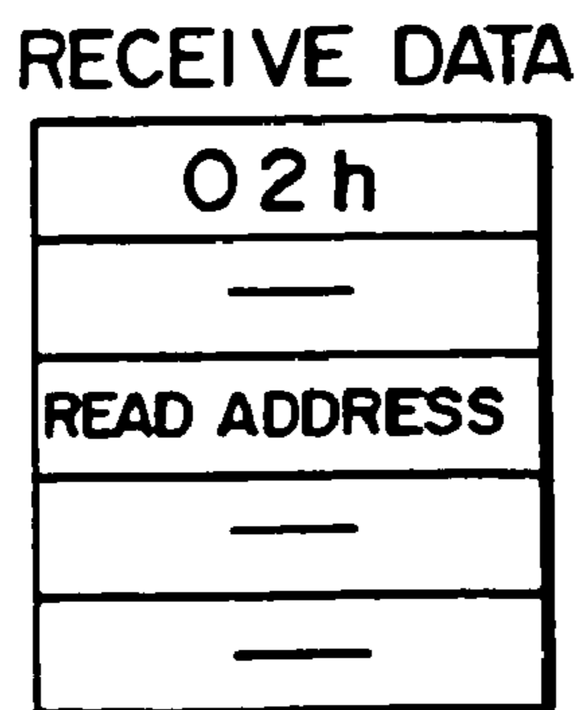
FIG. 10D READ COMMAND
