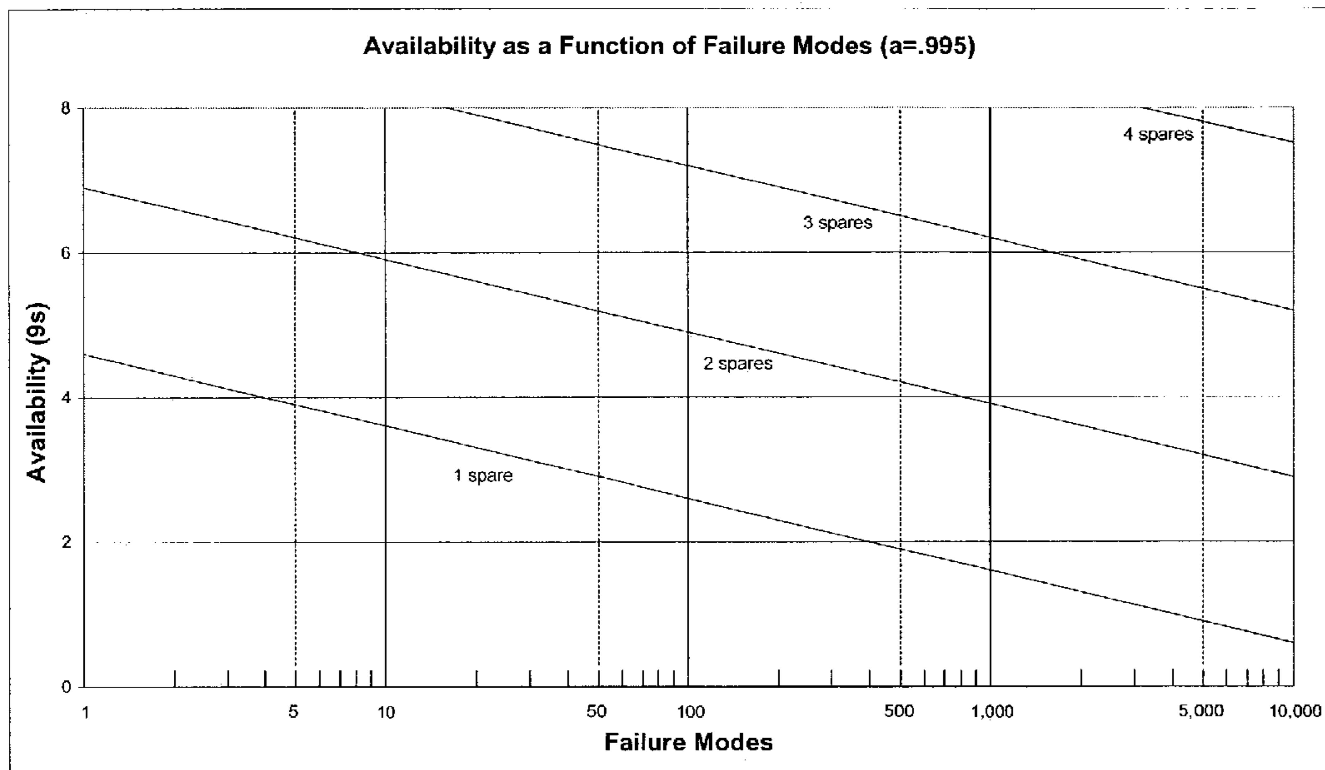
Failure Mode Impact on Availability
