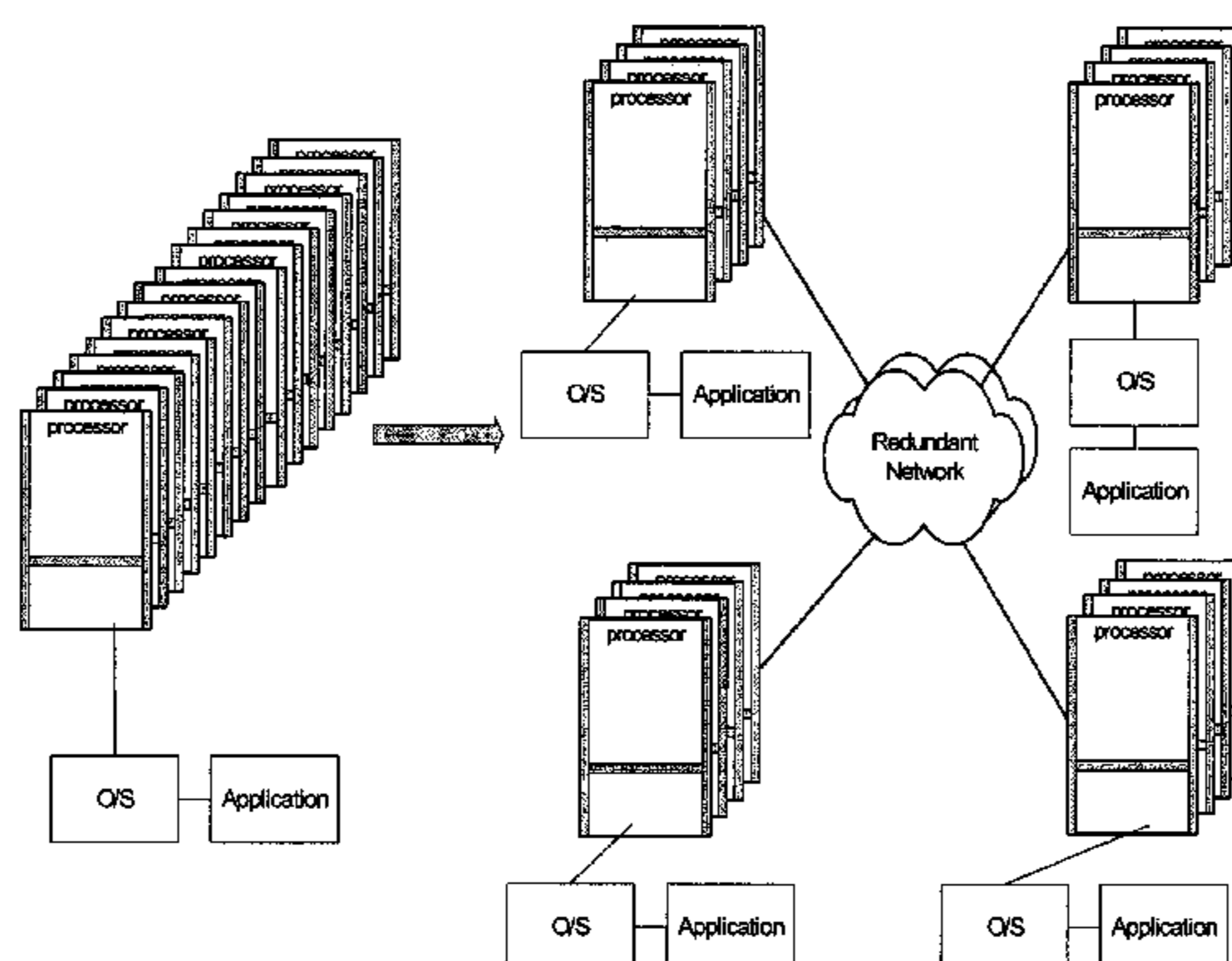
Node Splitting
