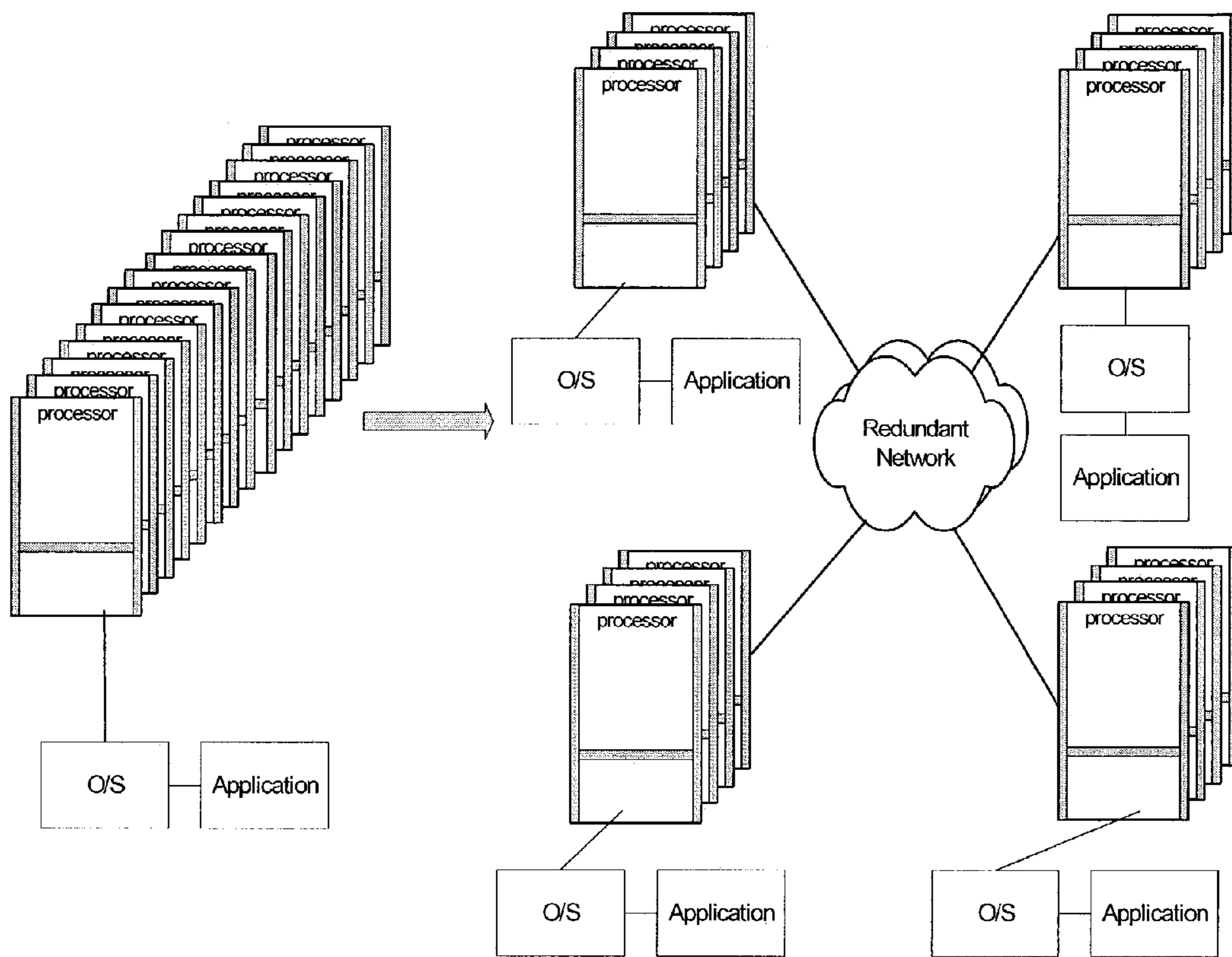
Node Splitting
