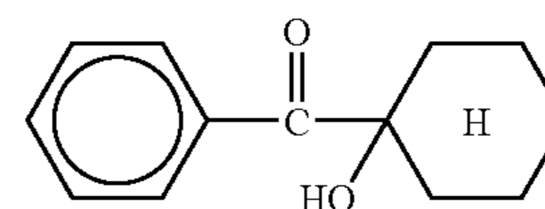
Irgacure 184:
