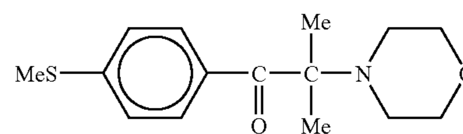
Irgacure 907:
