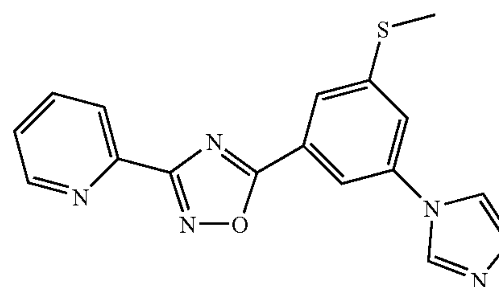
3-(2-Pyridyl)-5-(3-(1H-imidazol-1-yl)-5-thiomethoxyphenyl)-1,2,4-oxadiazole
