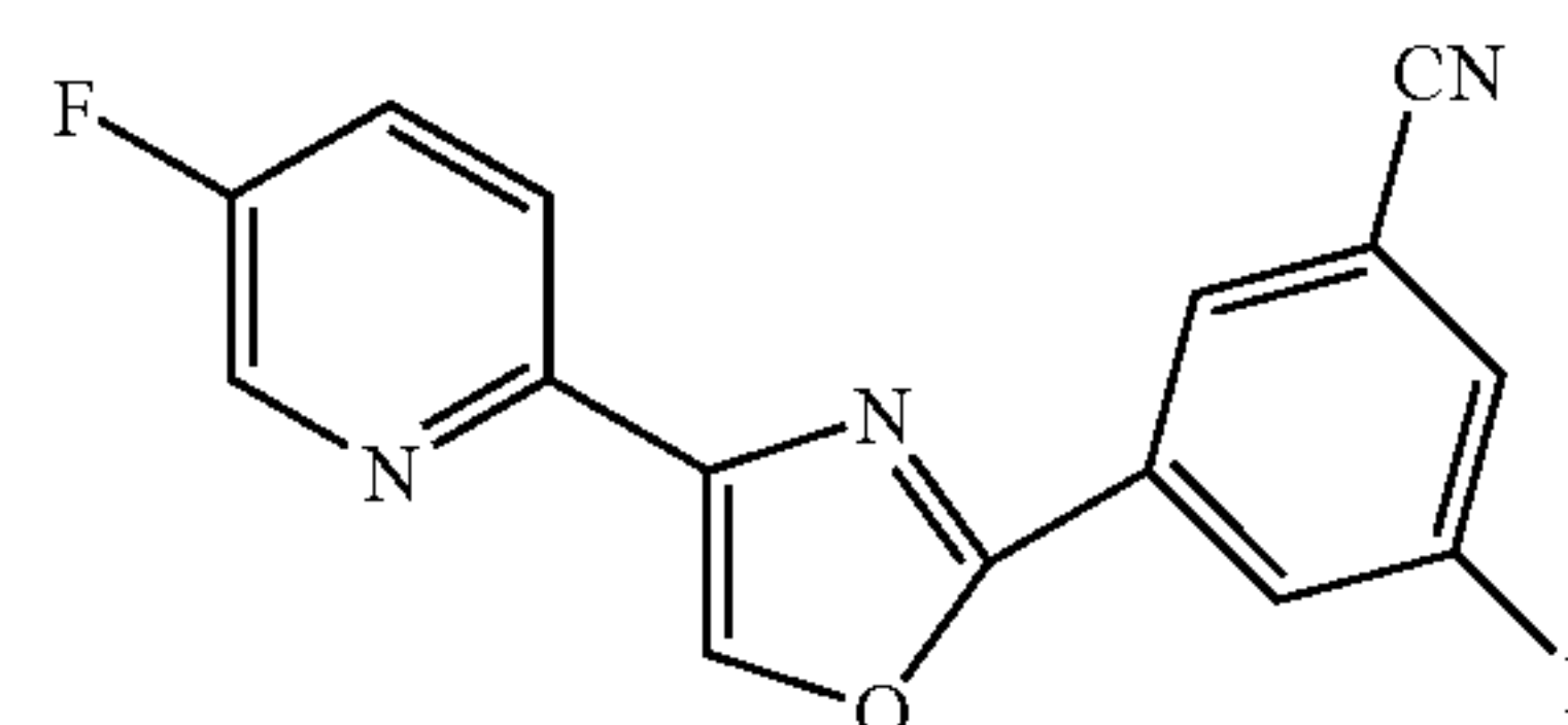
2-(3-cyano-5-fluorophenyl)-4-(5-Fluoropyrid-2-yl)-1,3-oxazole
