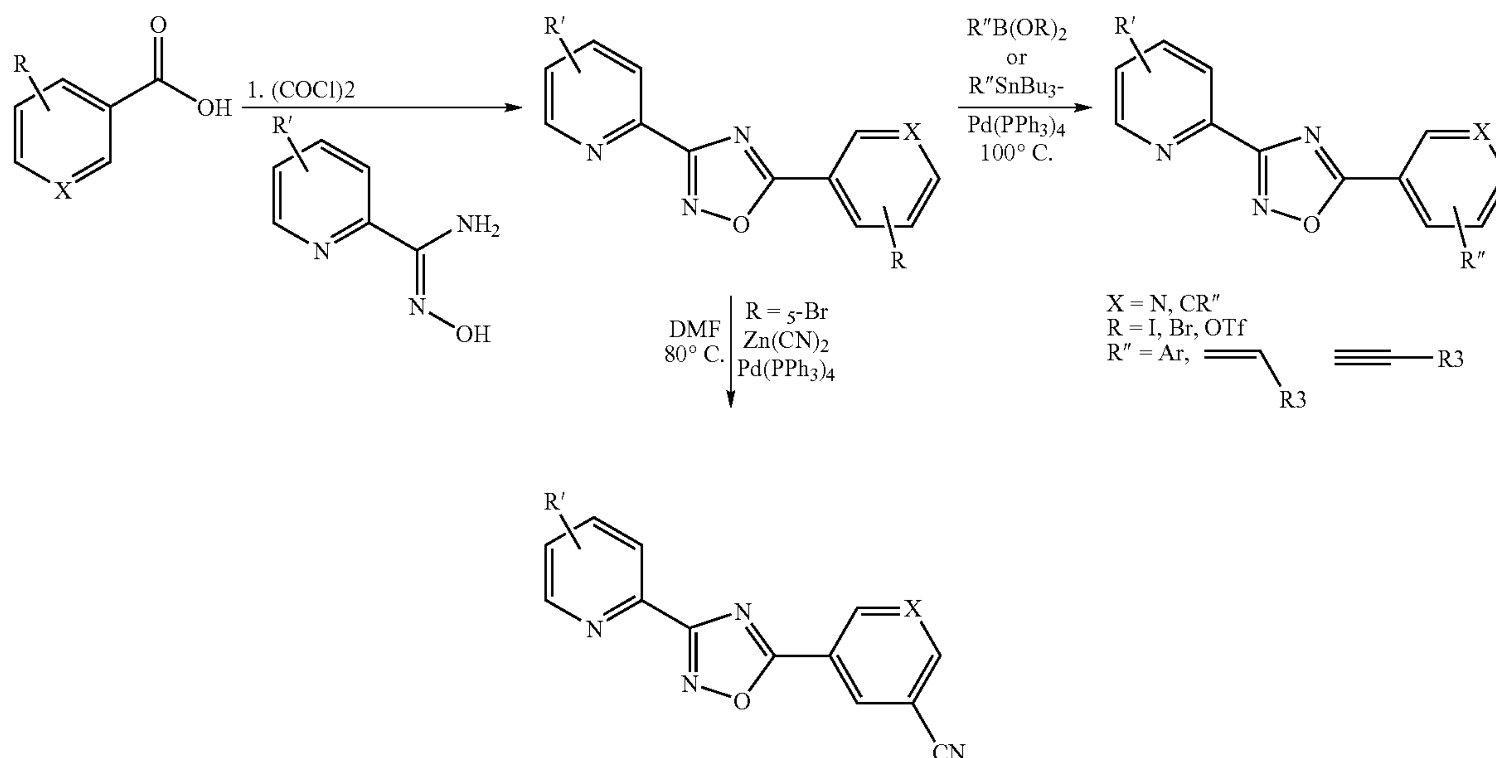
Scheme 3
