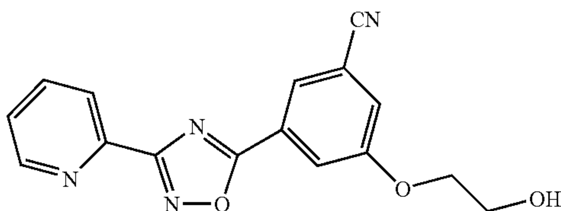
3-(2-Pyridyl)-5-(3-cyano-5-(2-hydroxyethoxy)phenyl)-1,2,4-oxadiazole
