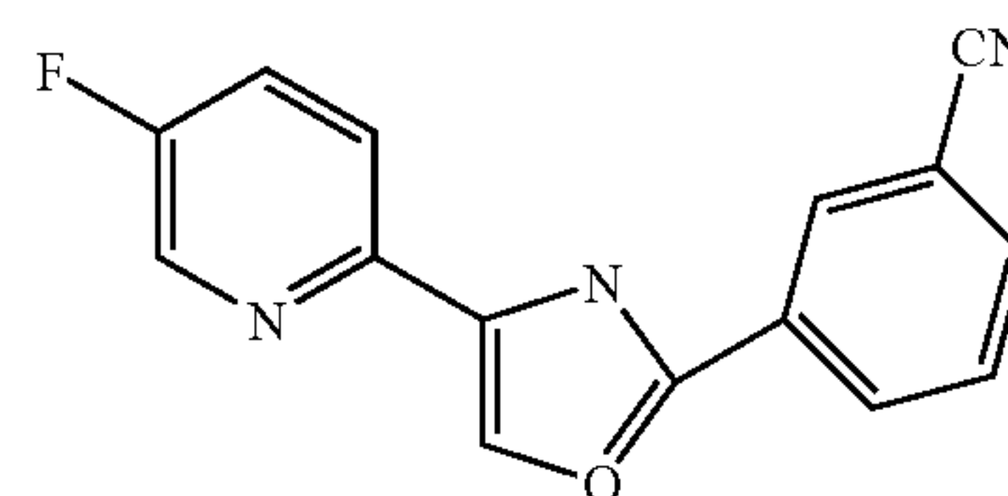
2-(3-cyanophenyl)-4-(5-Fluoropyrid-2-yl)-1,3-oxazole
