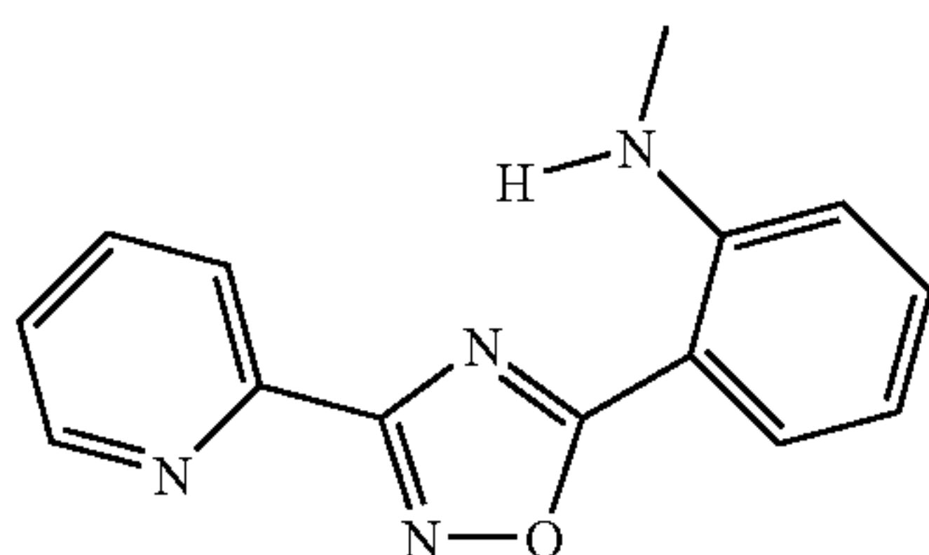
3-(2-Pyridyl)-5-(2-N-methylaminophenyl)-1,2,4-oxadiazole
