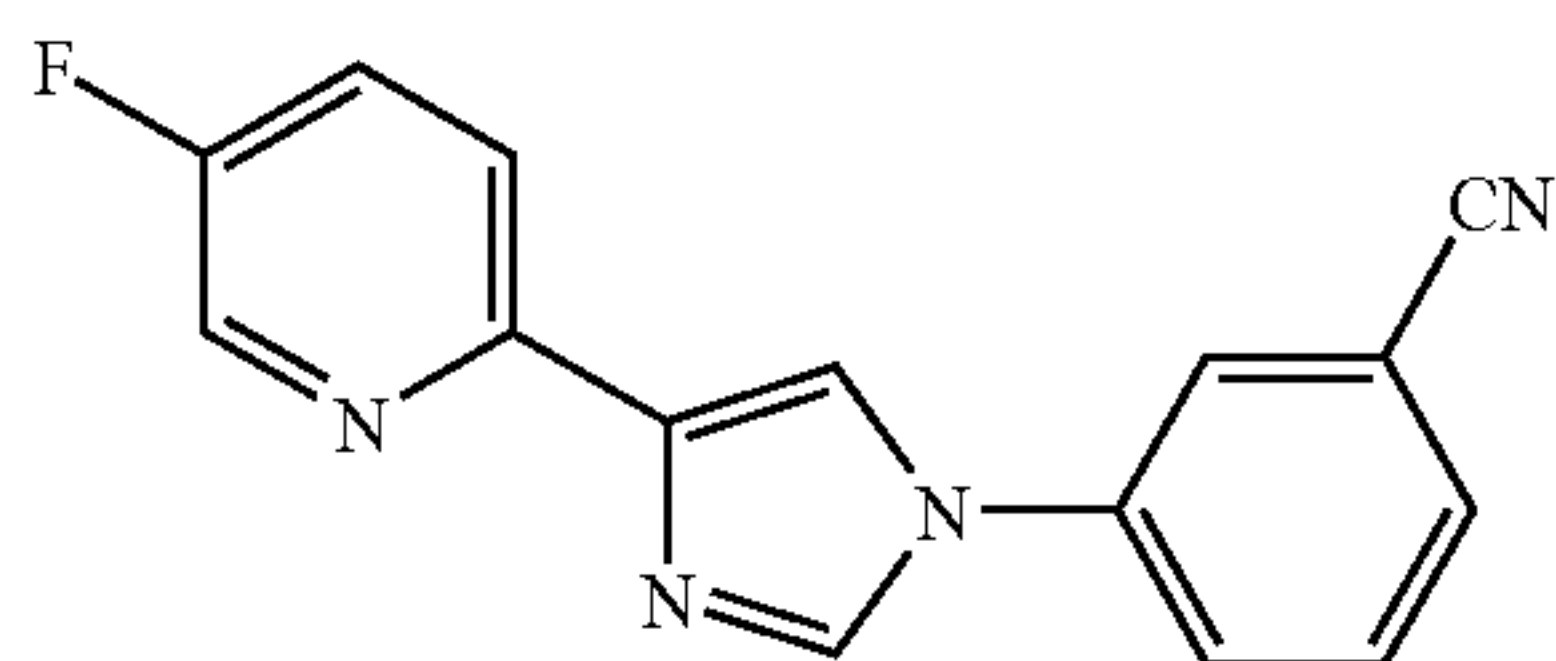
1-(3-Cyanophenyl)-4-(5-fluoro-2-pyridyl)-1H-imidazole
