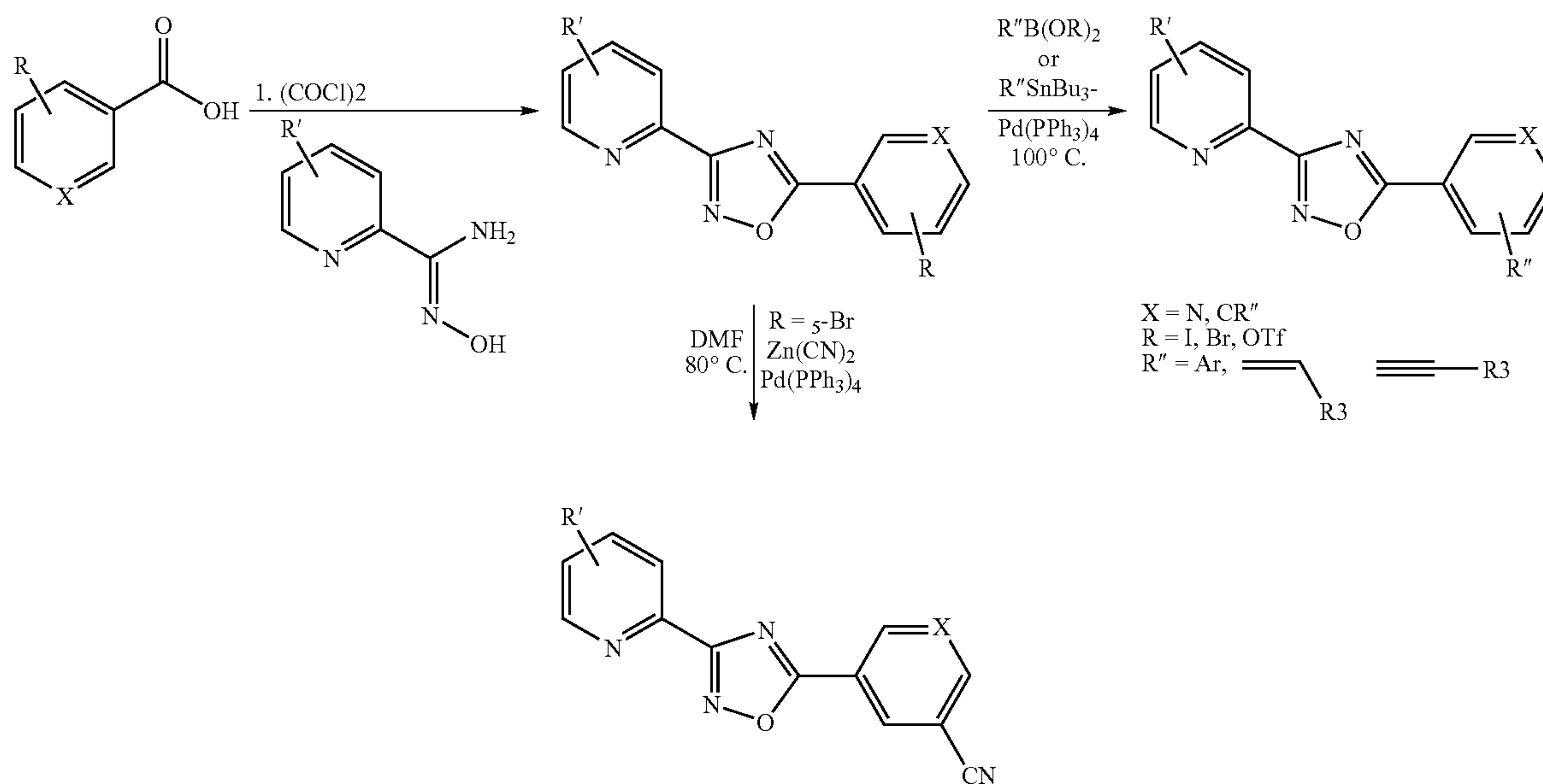
Scheme 3
