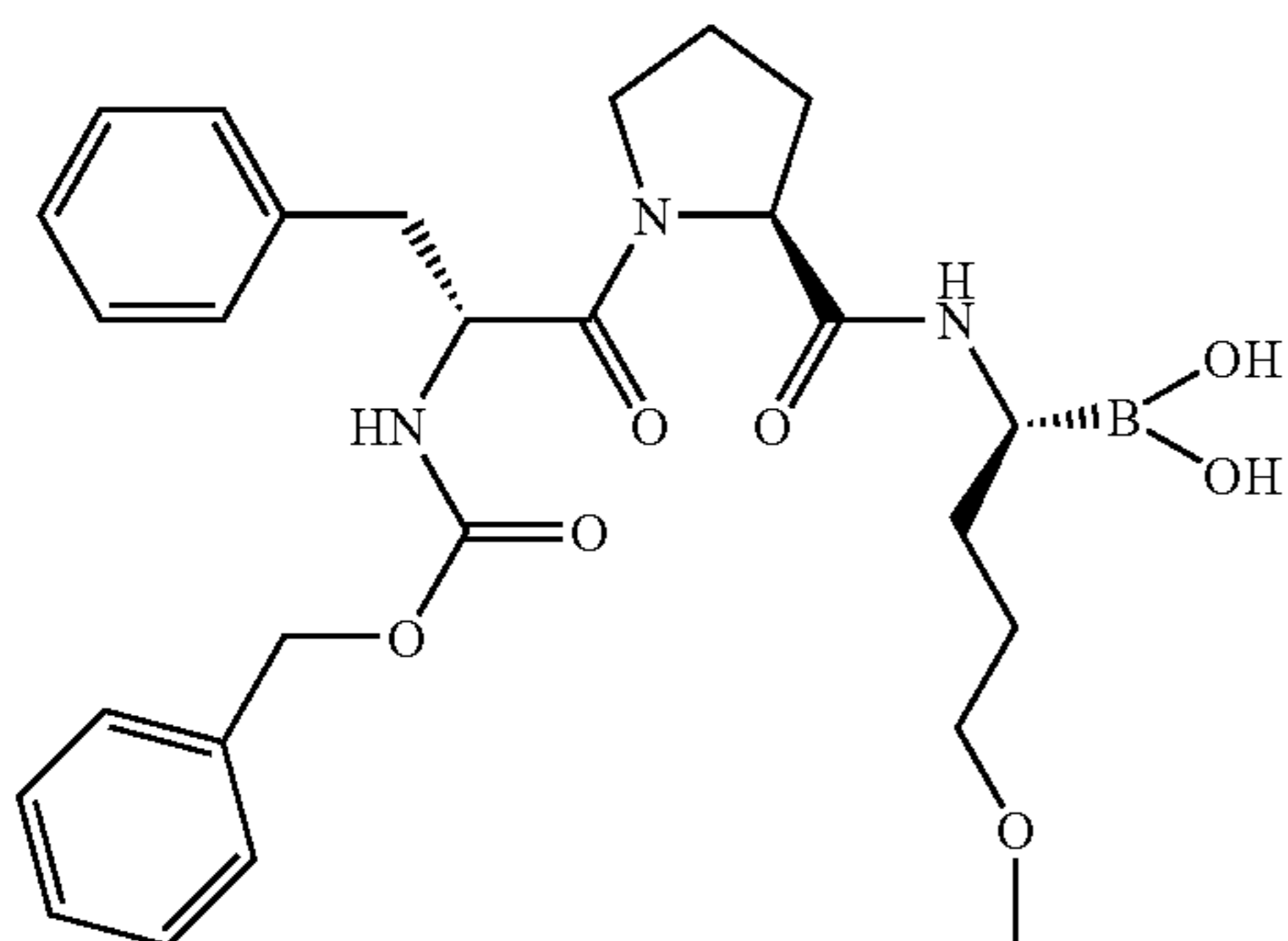
Cbz-(R)-Phe-(S)-Pro-(R)-boroMpg—OH
