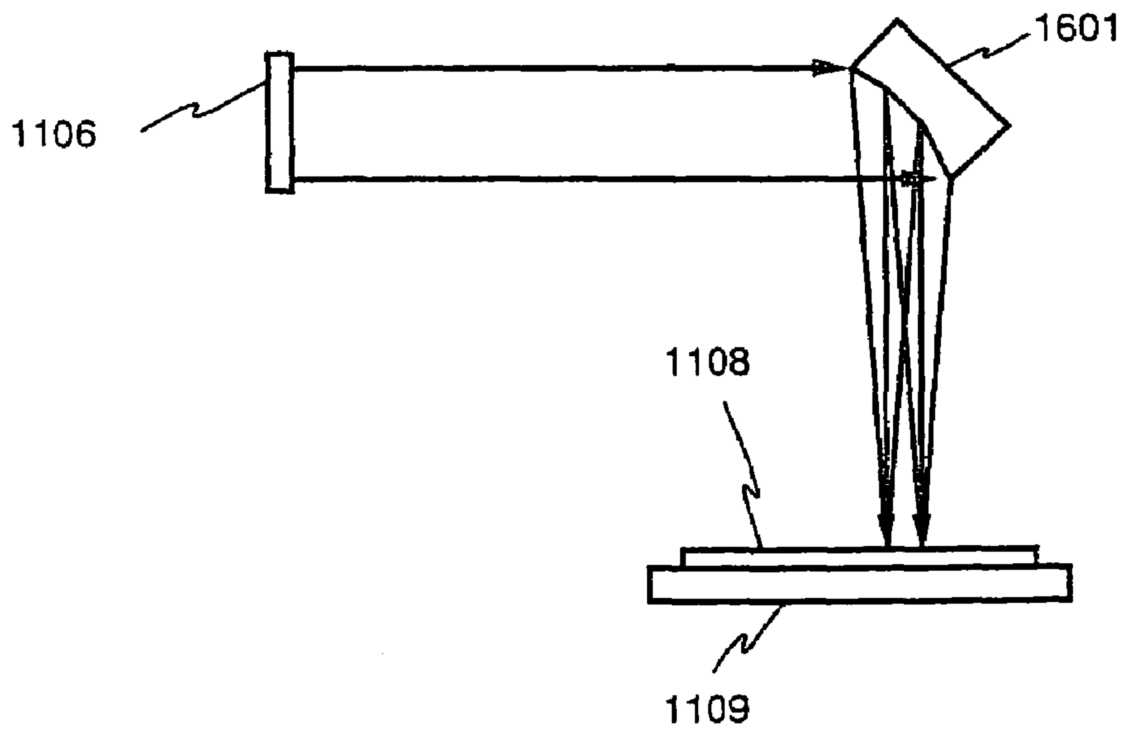
Fig. 6B side view
