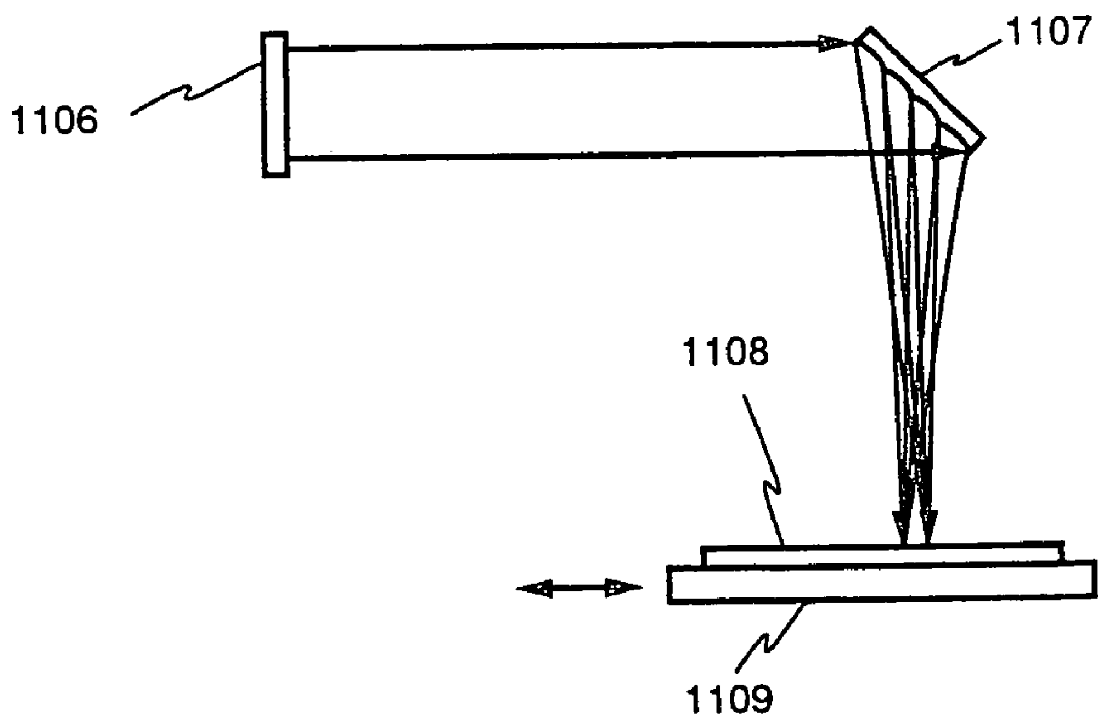
Fig. 1B side view
