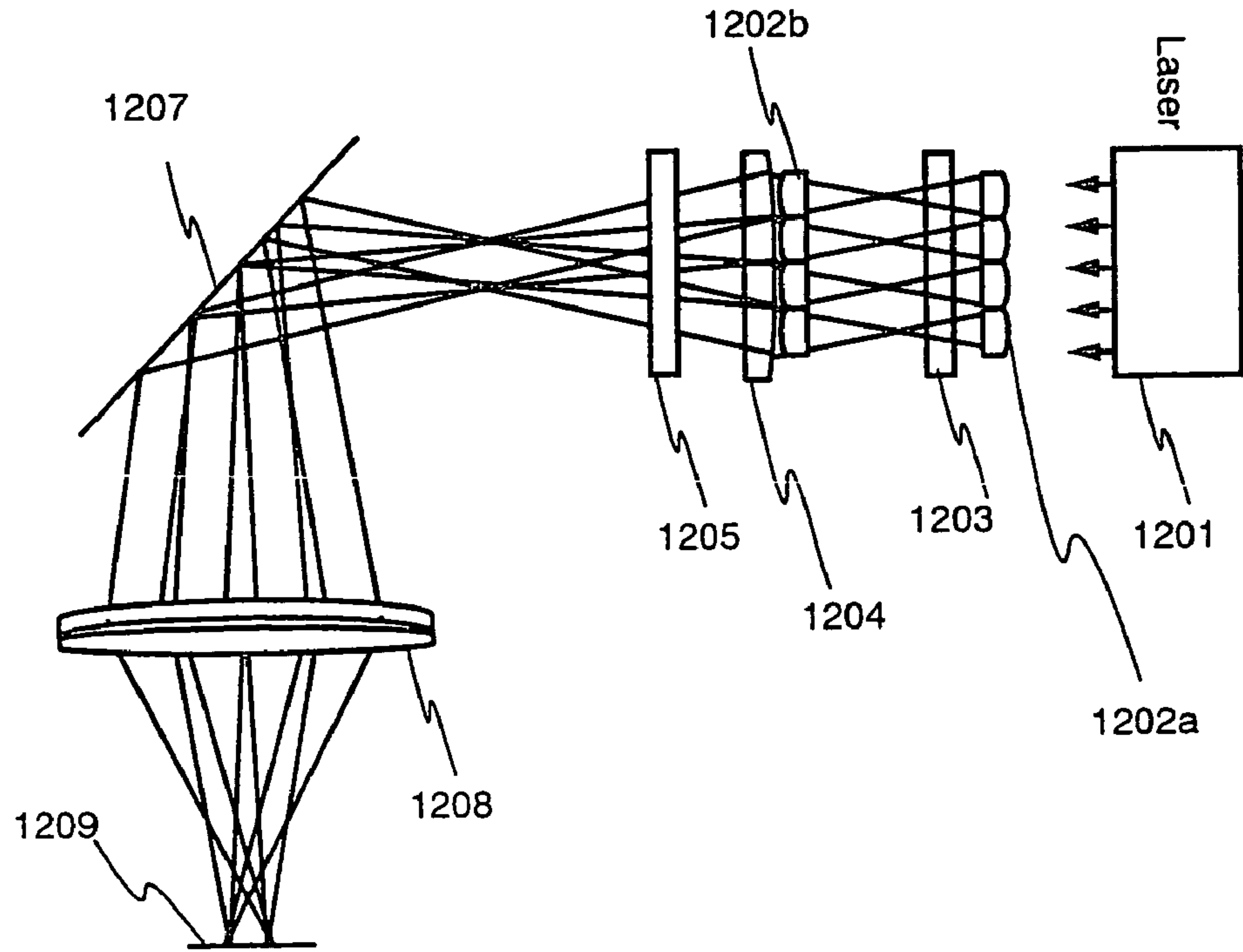
Fig. 2A side view prior art
