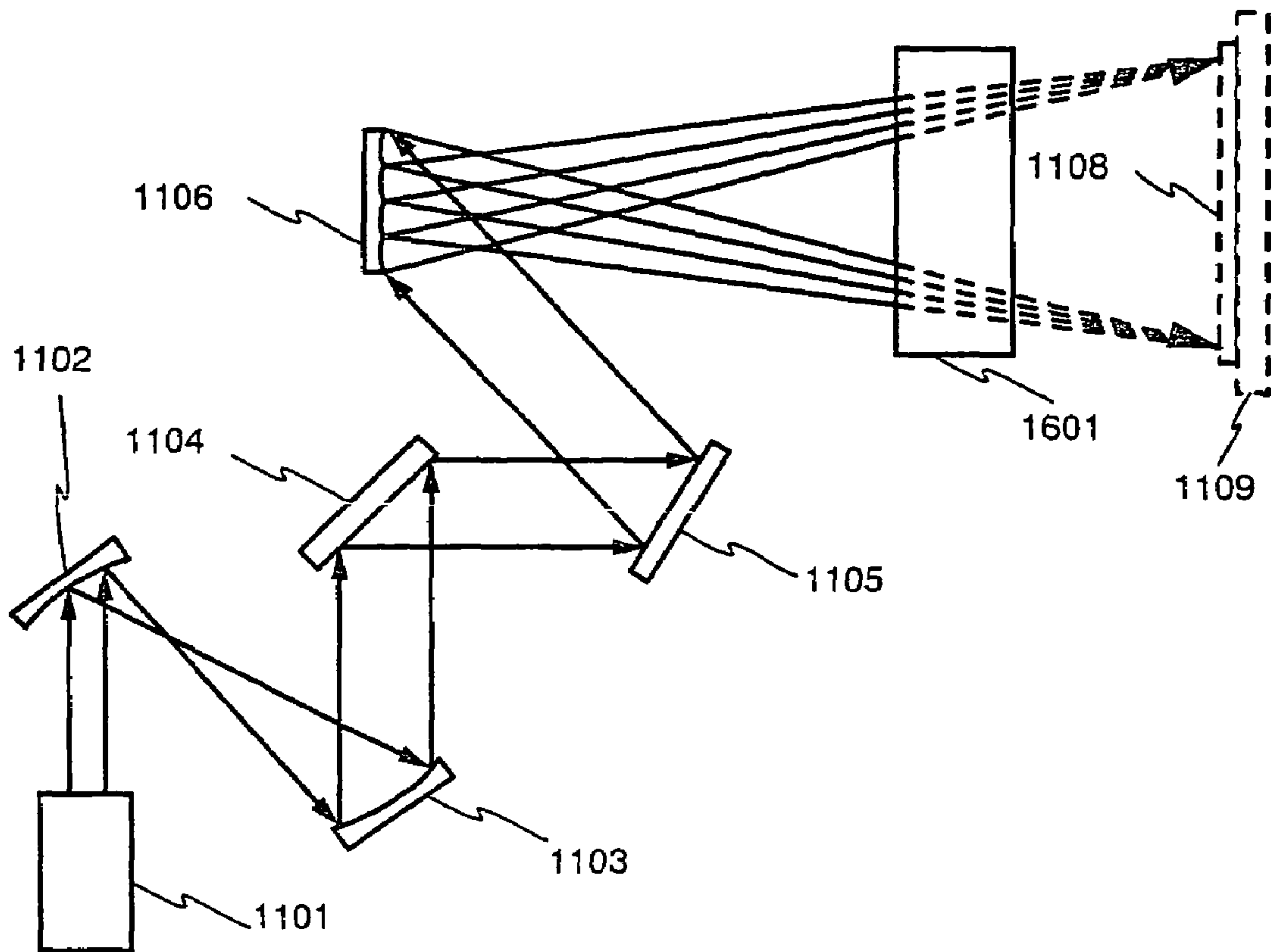
Fig. 6A top view
