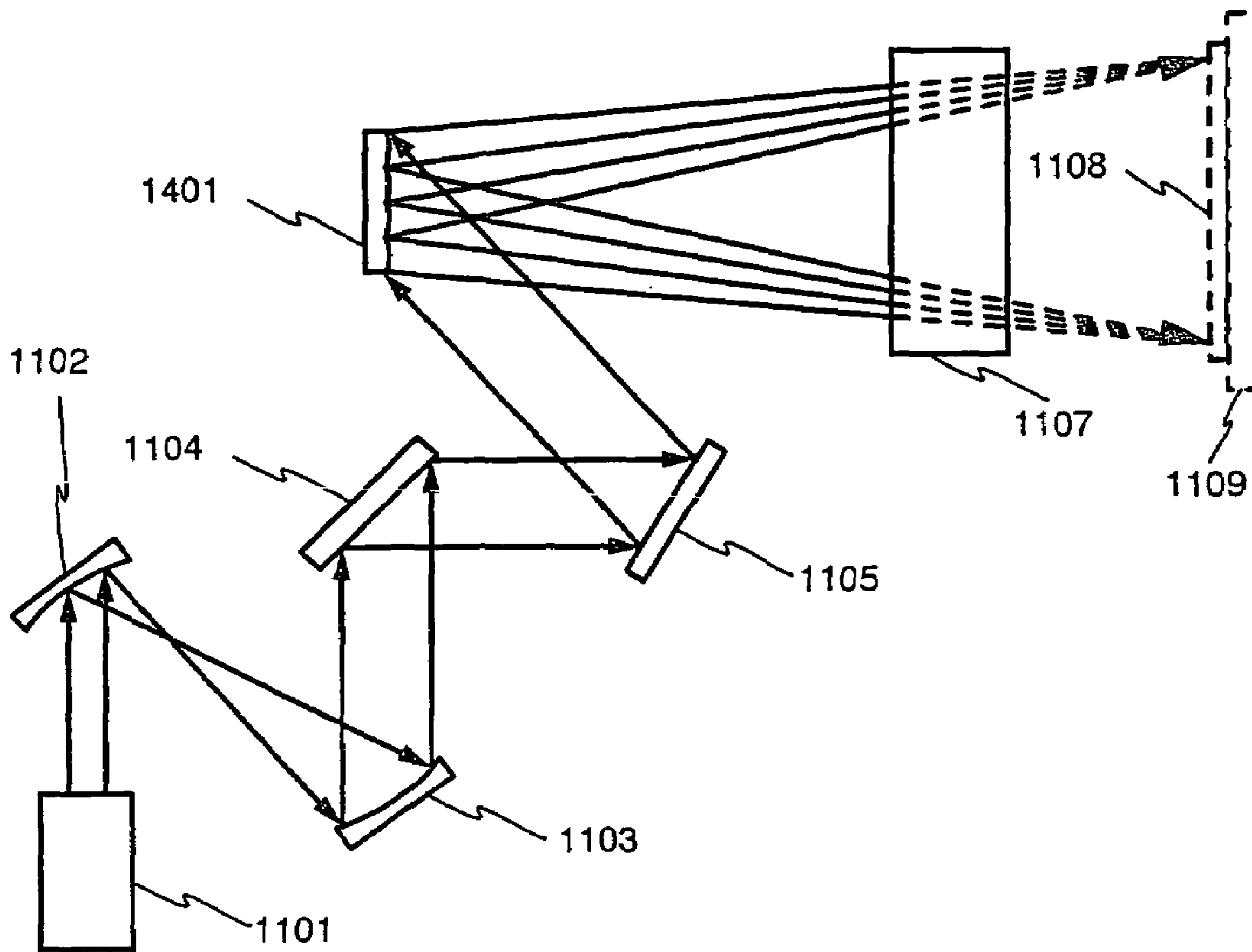
Fig. 4A top view
