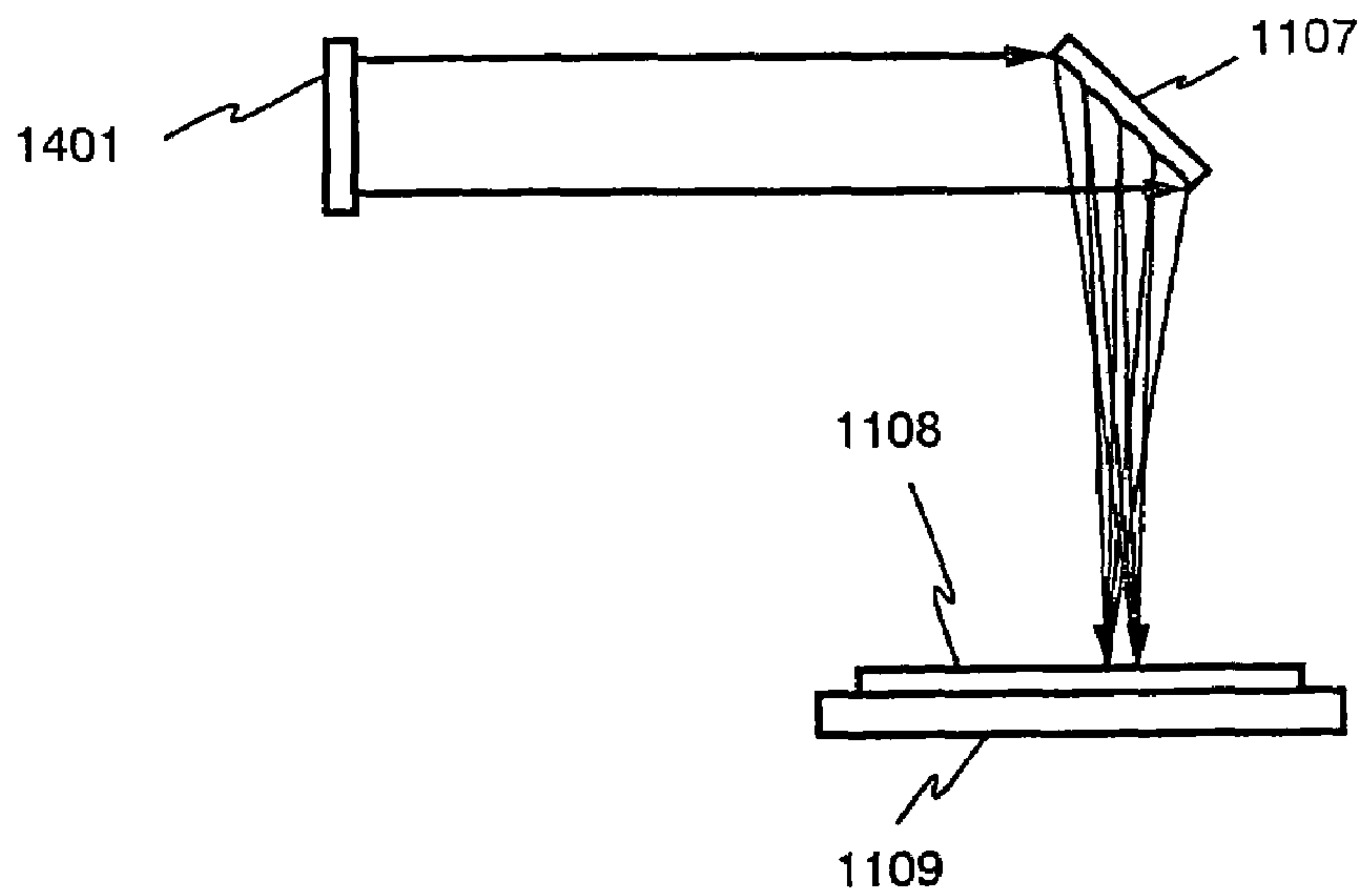
Fig. 4B side view
