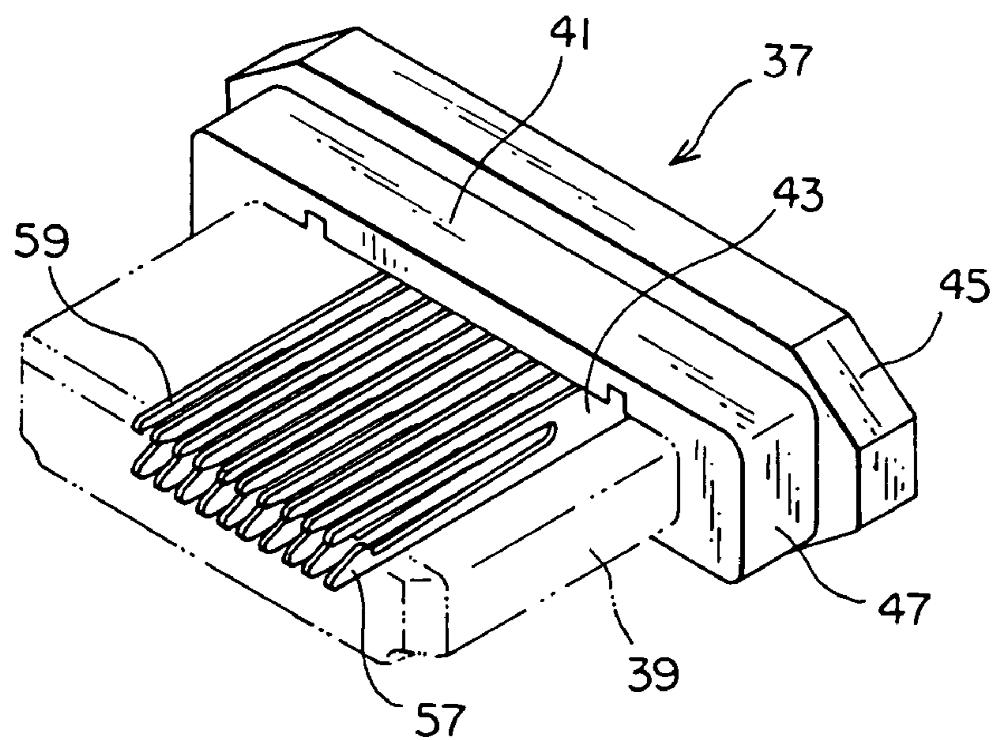
FIG. 4 PRIOR ART
