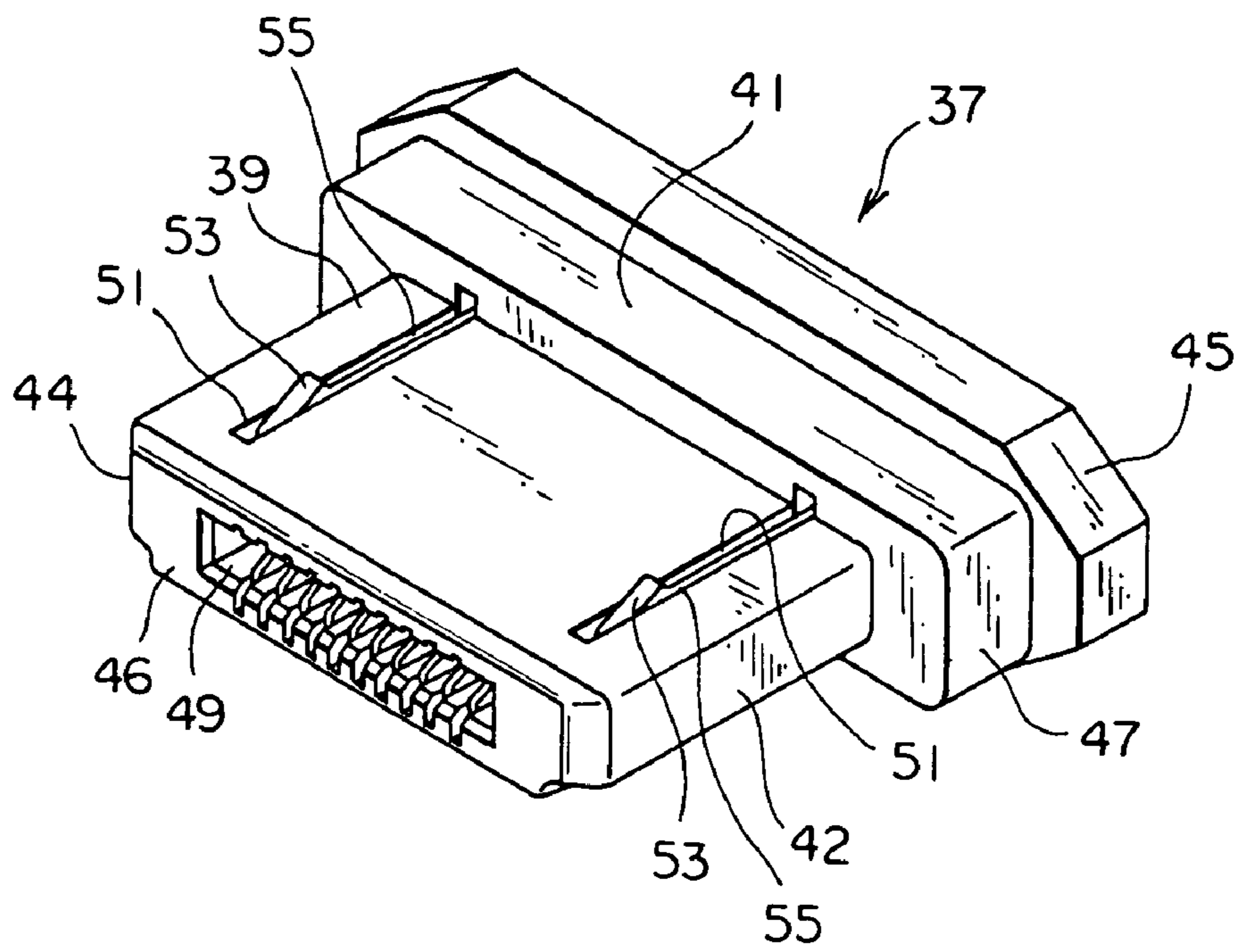
FIG. 3 PRIOR ART
