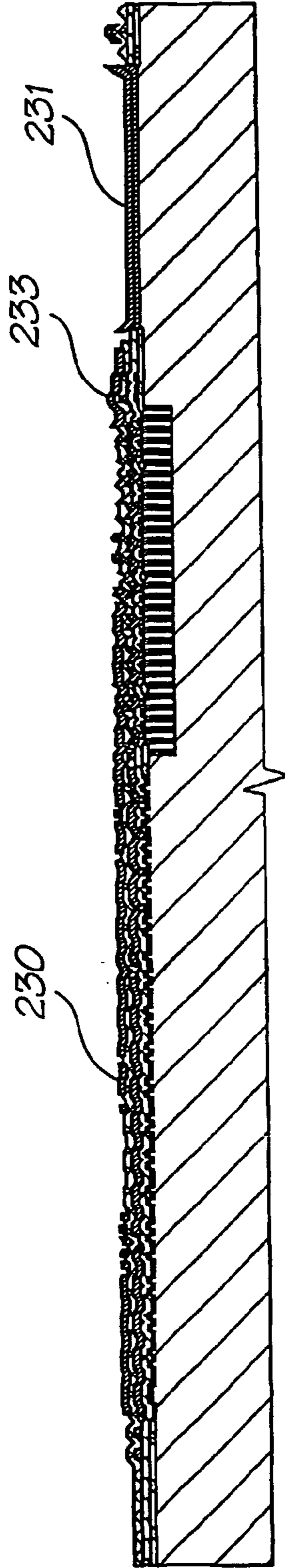
Deposit metal 2
