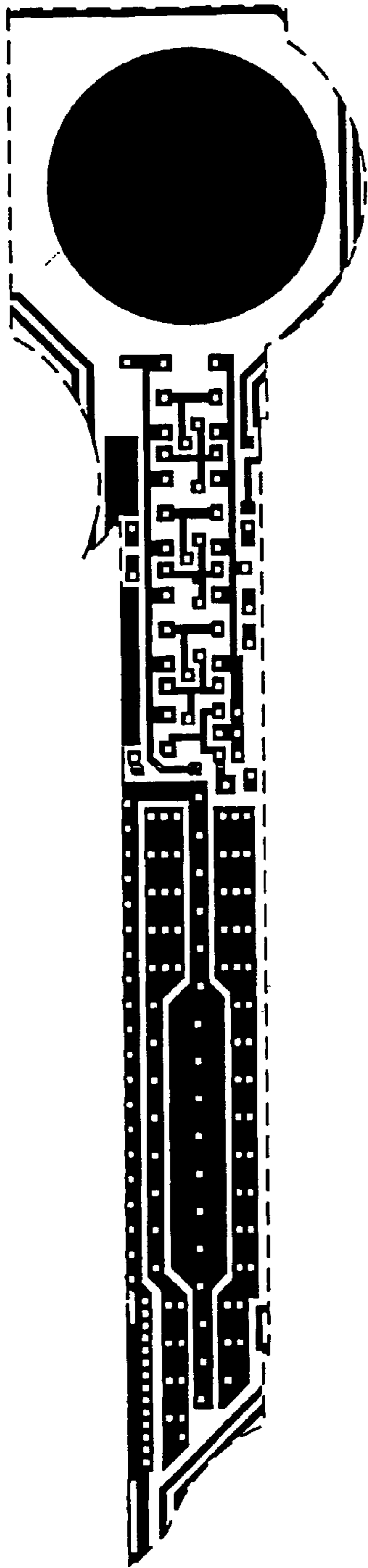
Metal 1 mask
