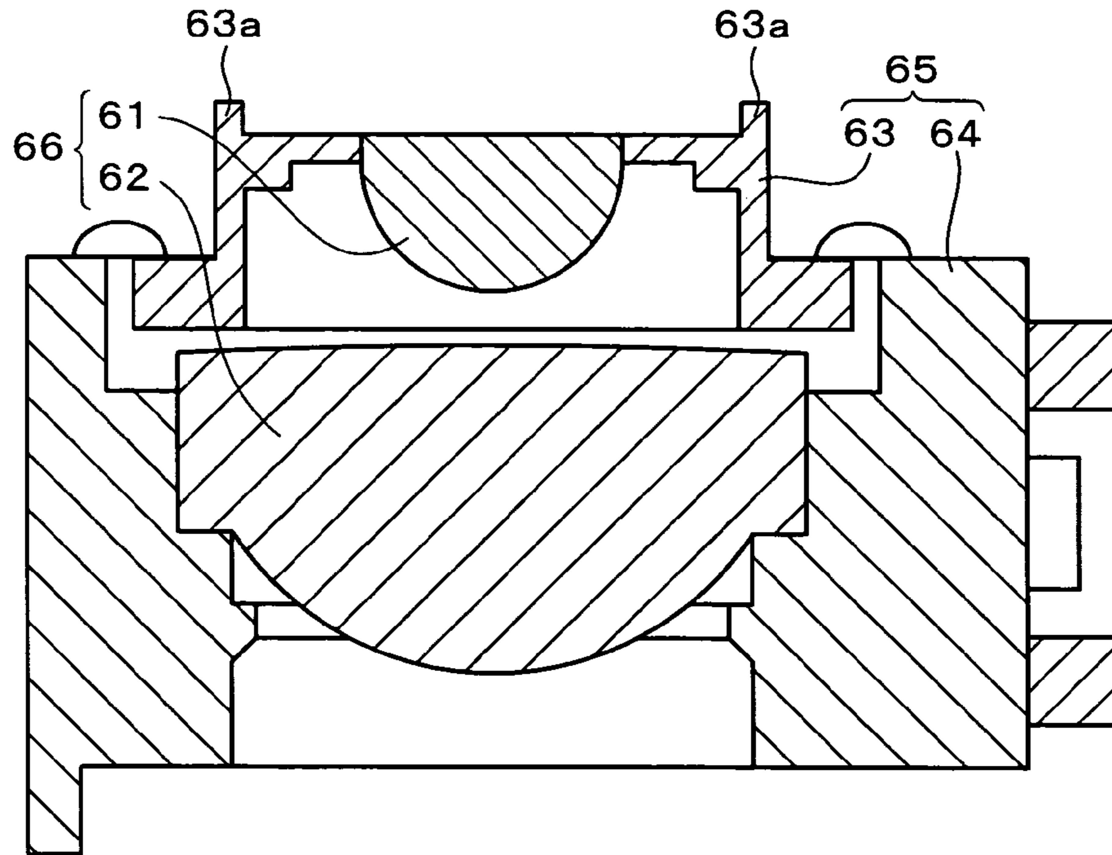
FIG. 8 (PRIOR ART)
