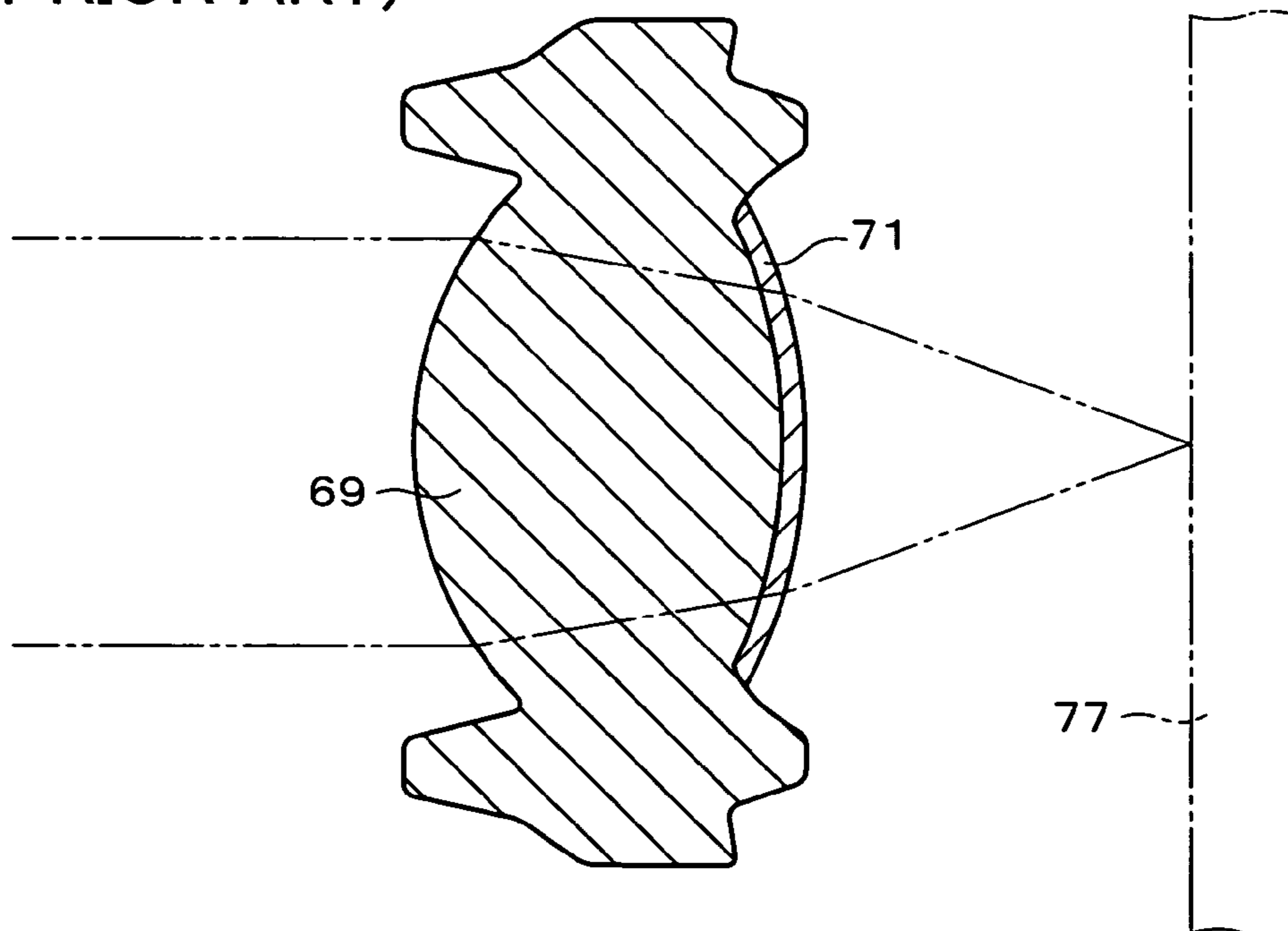
FIG. 9 (PRIOR ART)
