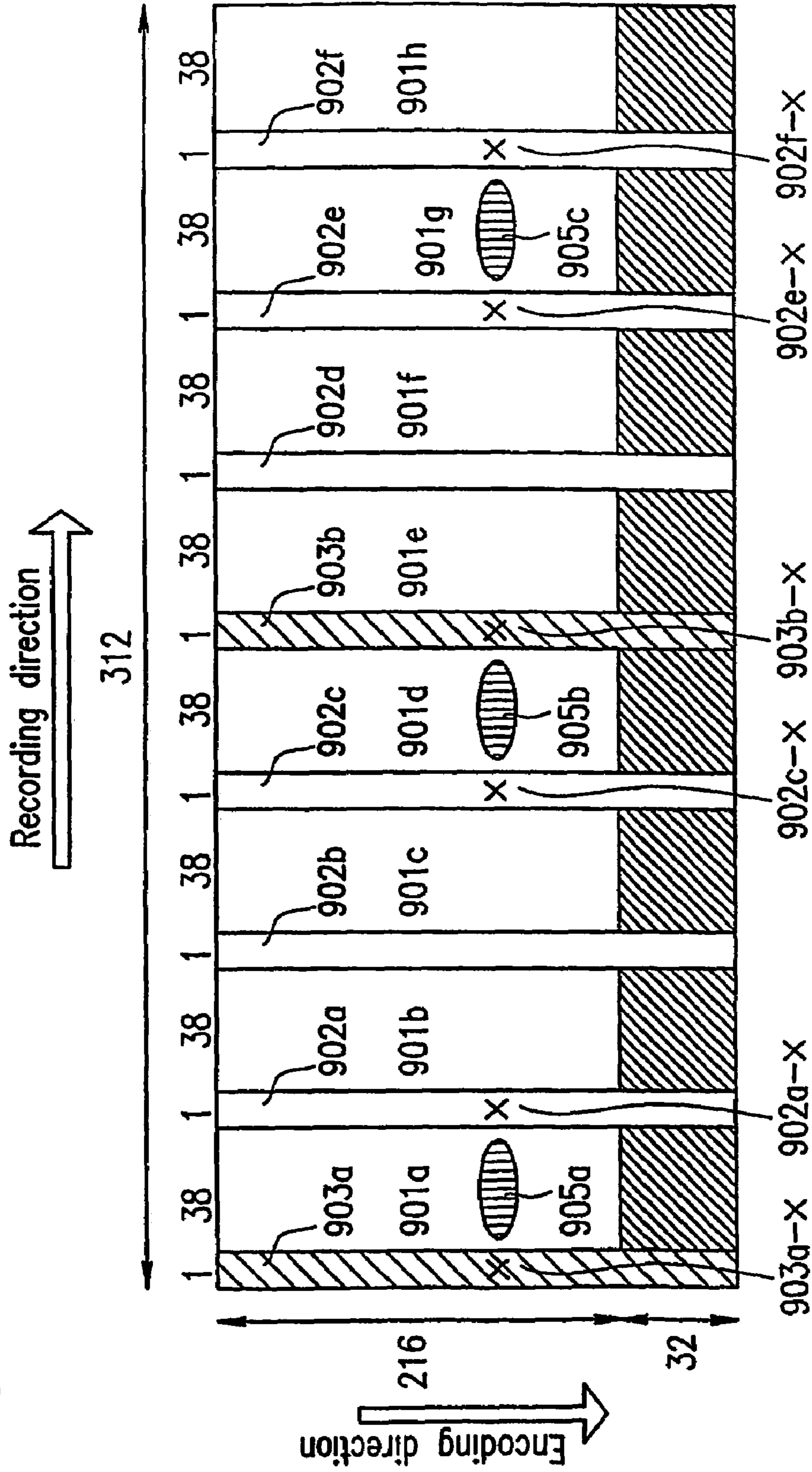
FIG. 10 CONVENTIONAL ART
