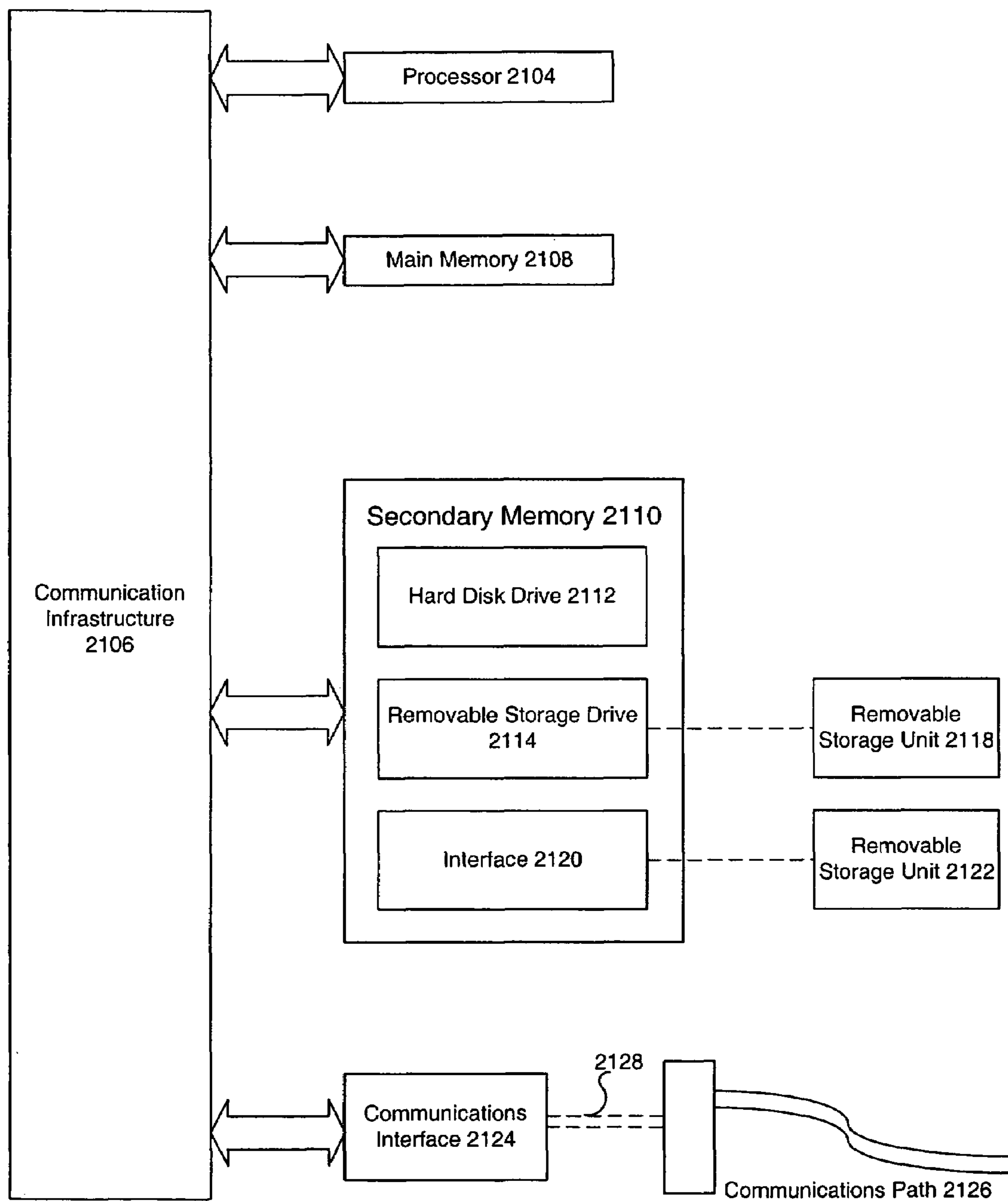
Computer System 2100
