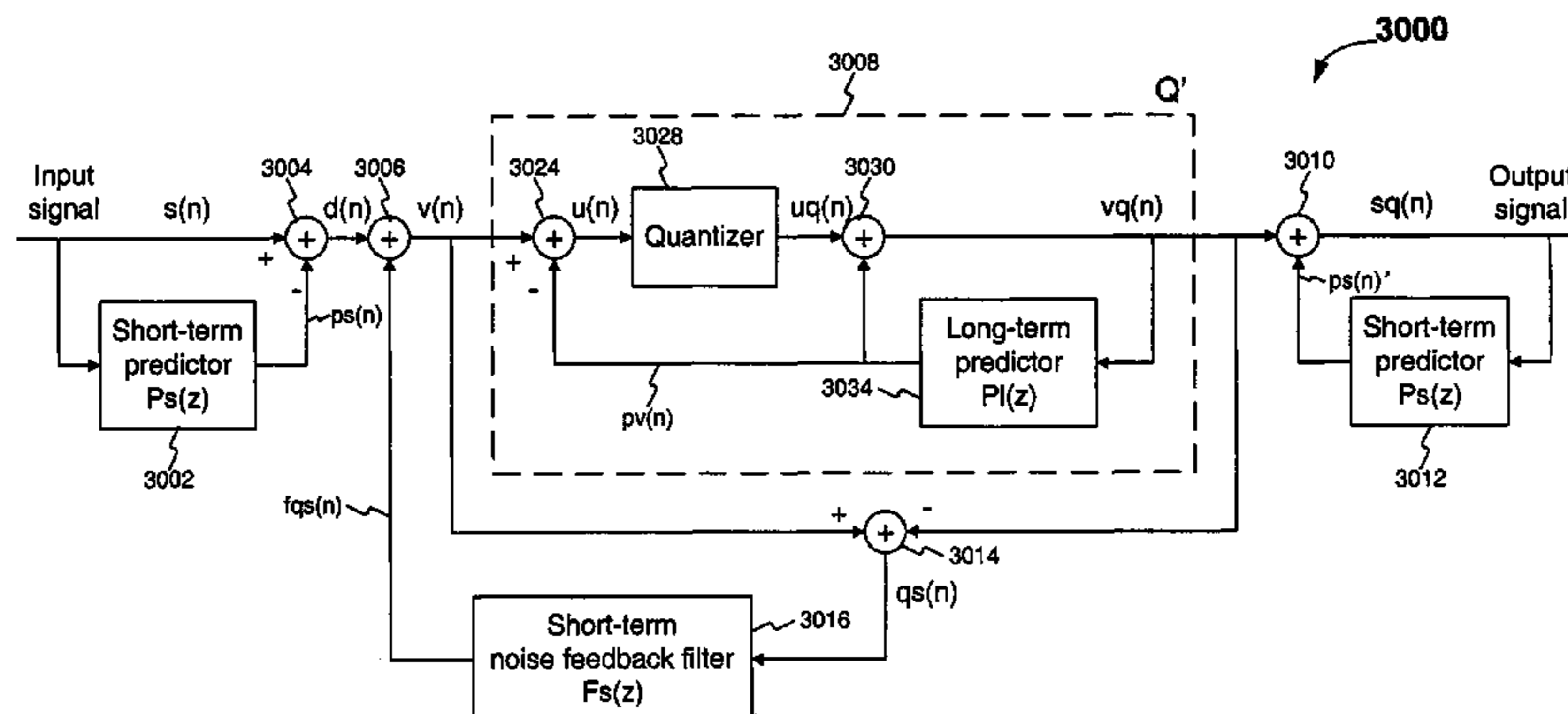
Noise Feedback Coding with short-term and long-term prediction but only short-term noise spectral shaping
