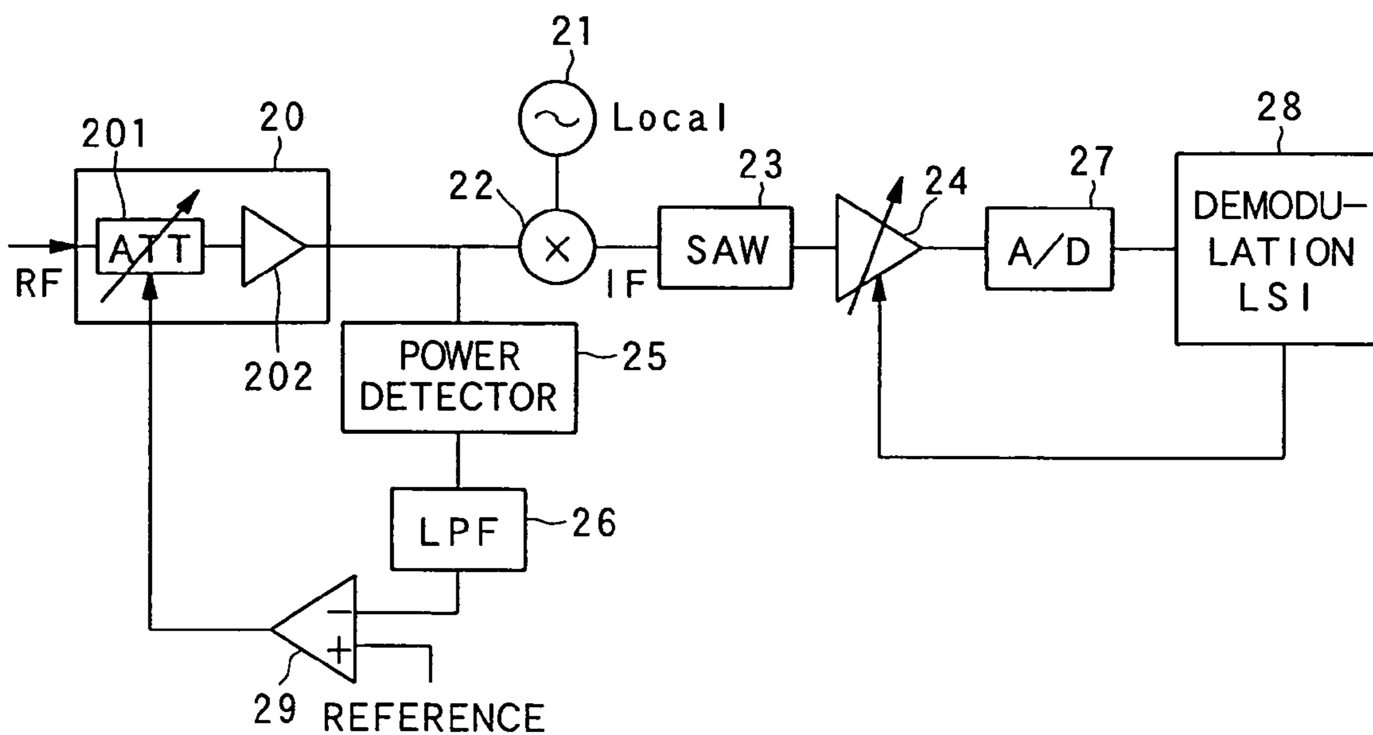
PRIOR ART
