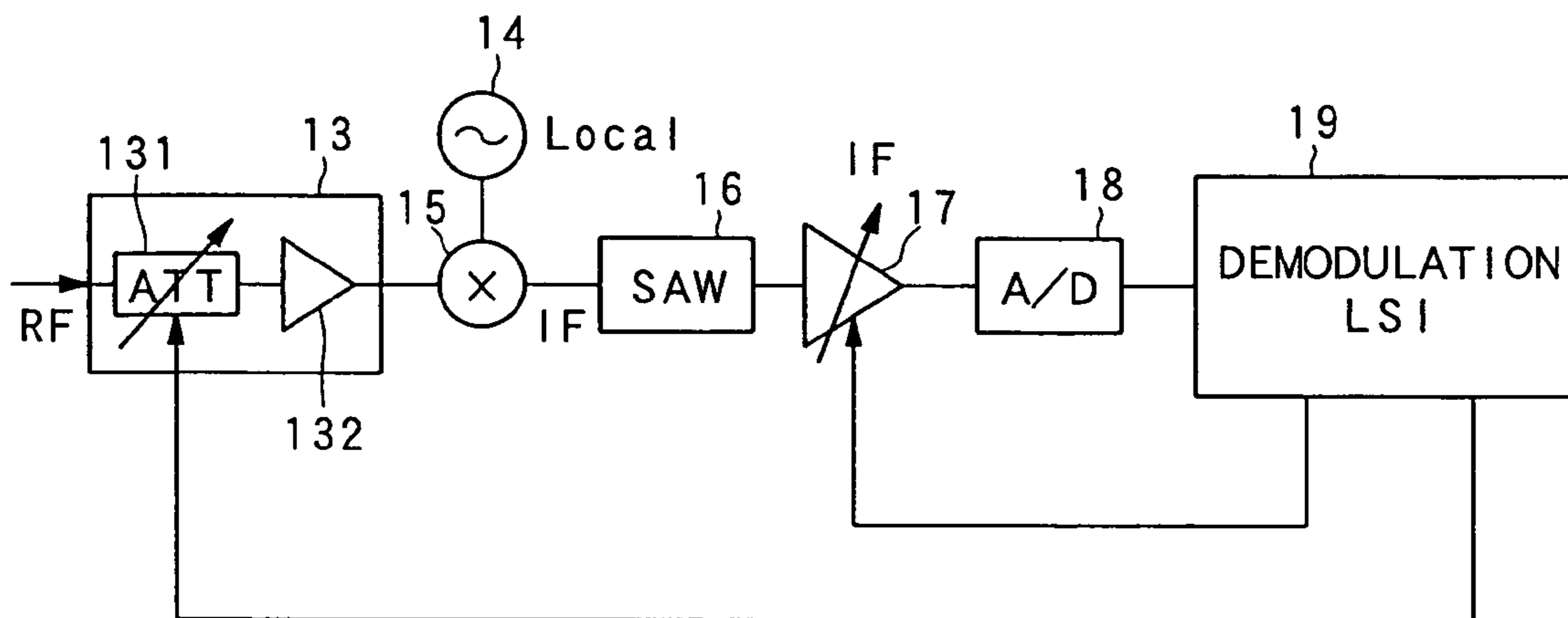
PRIOR ART
