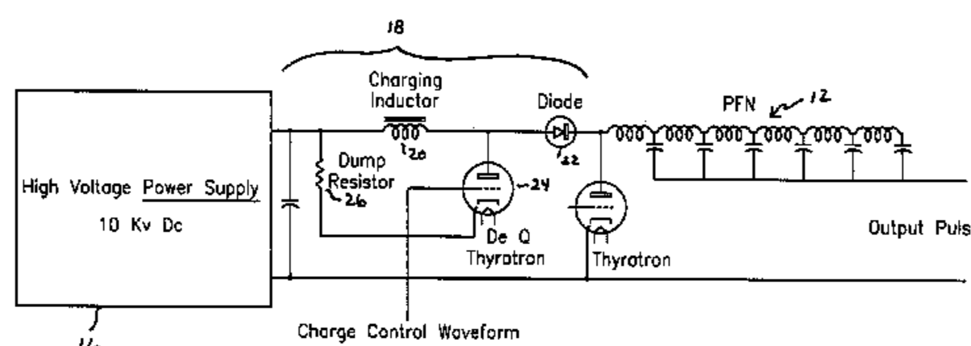
Modulator With Inductive Charging And De Q Control
