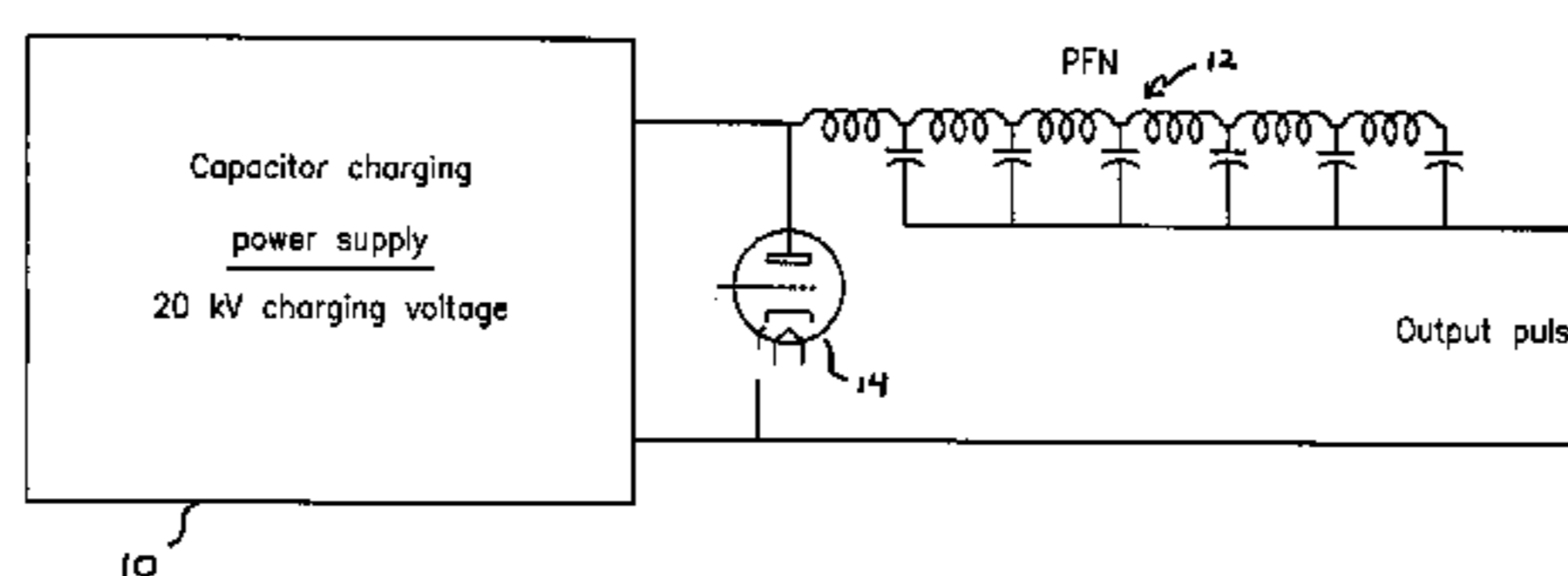
Modulator with Capacitor Charging Power Supply
