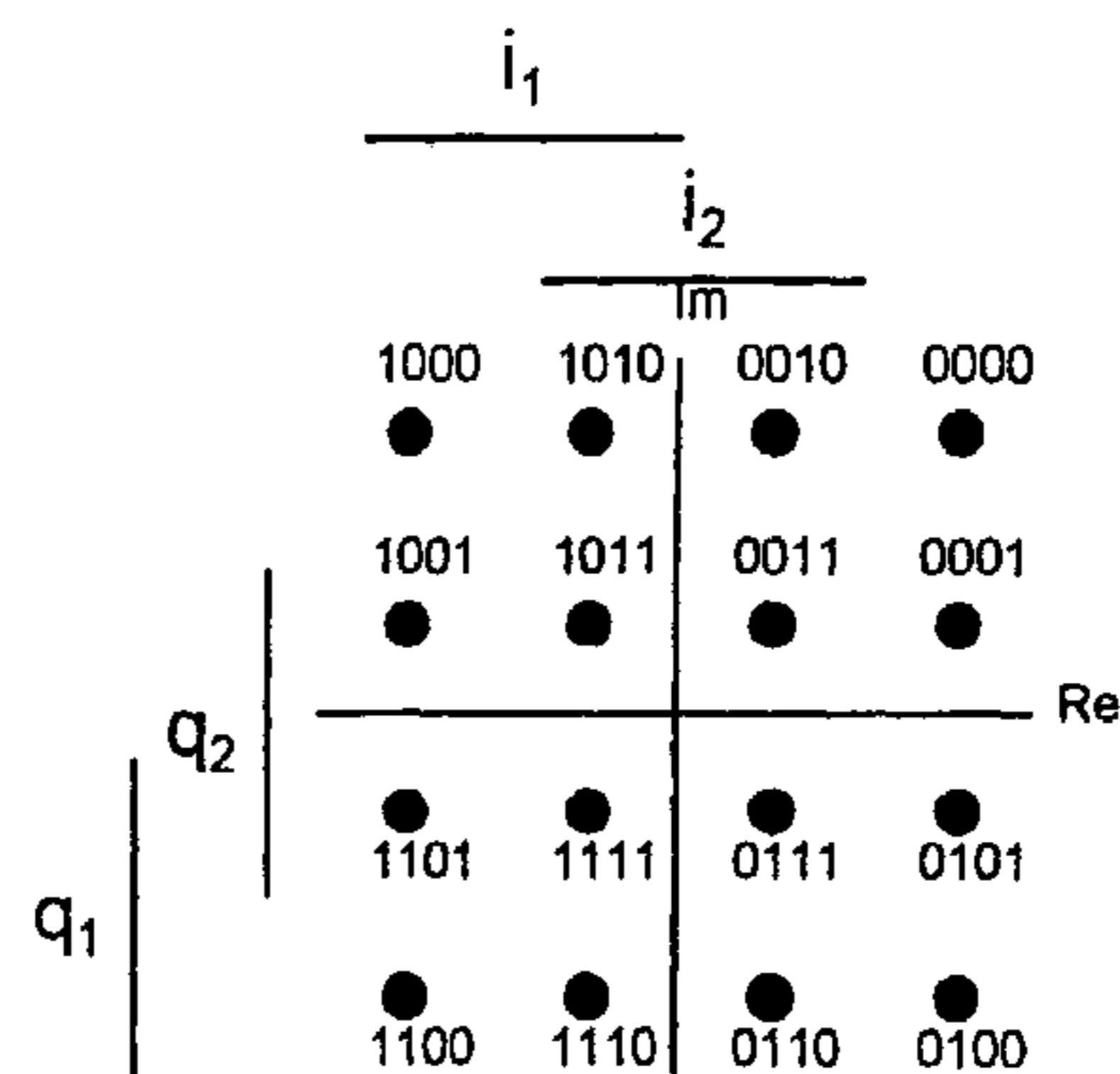
Constellation 4
