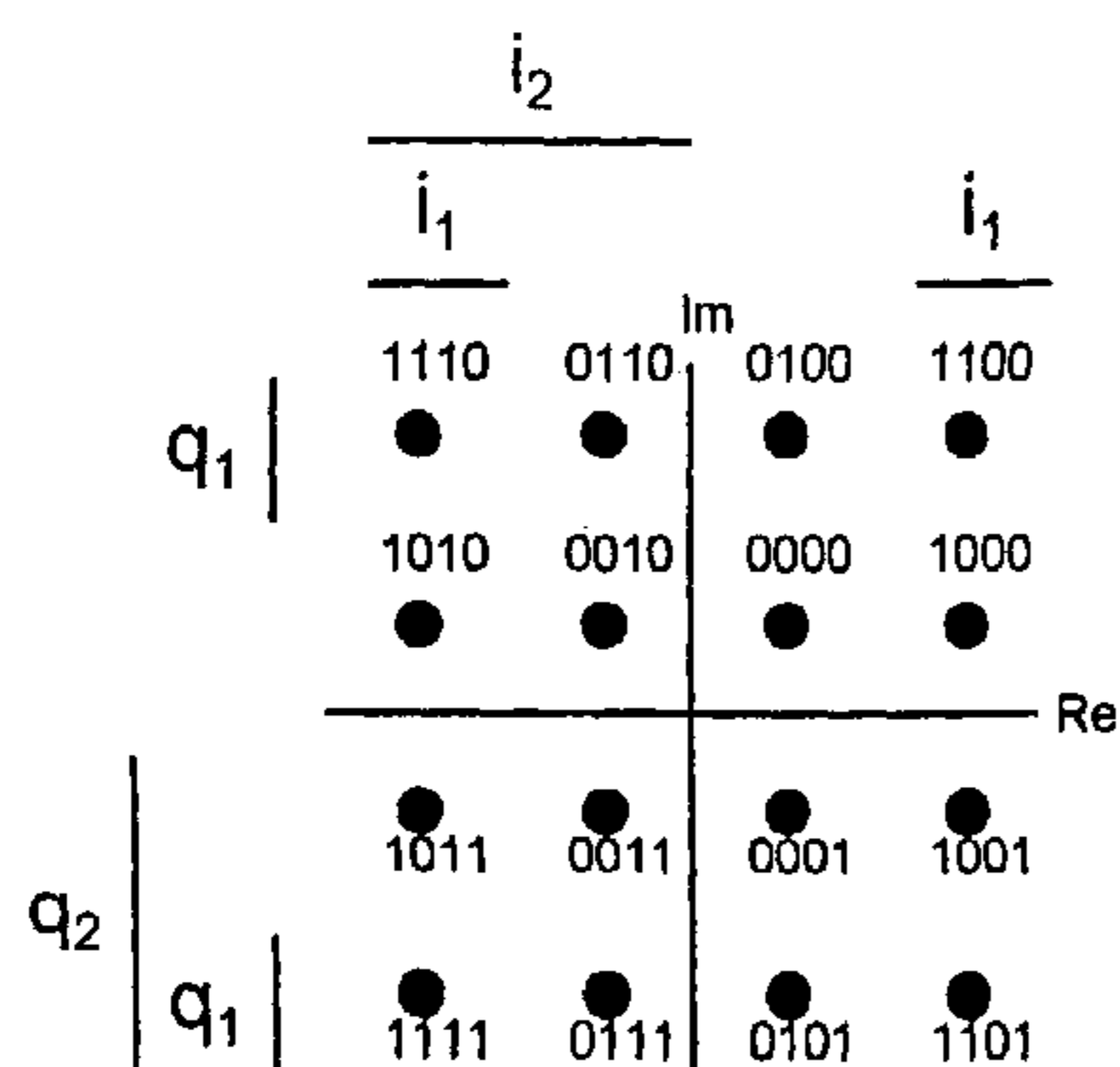
Constellation 3
