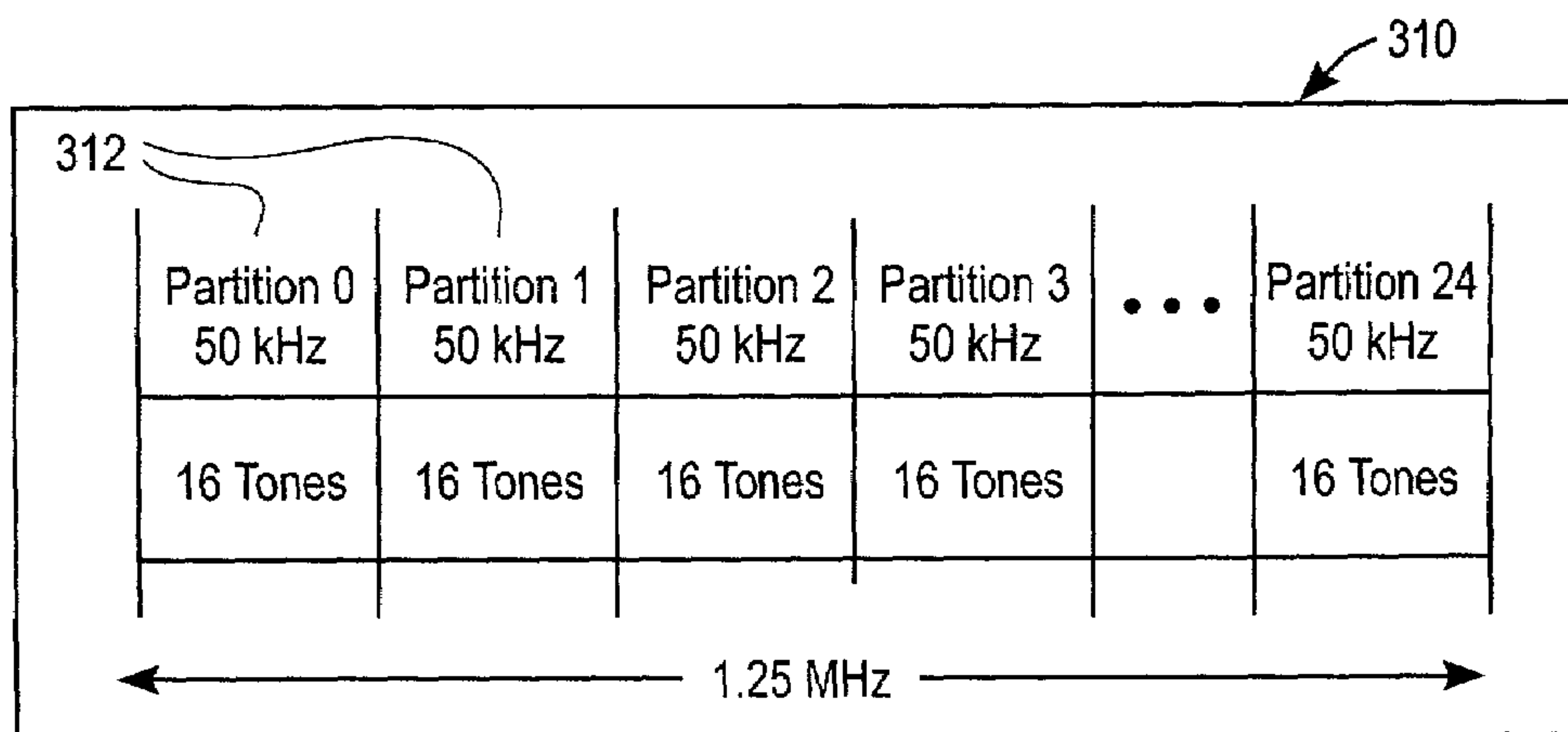
FIG. 20 (PRIOR ART)
