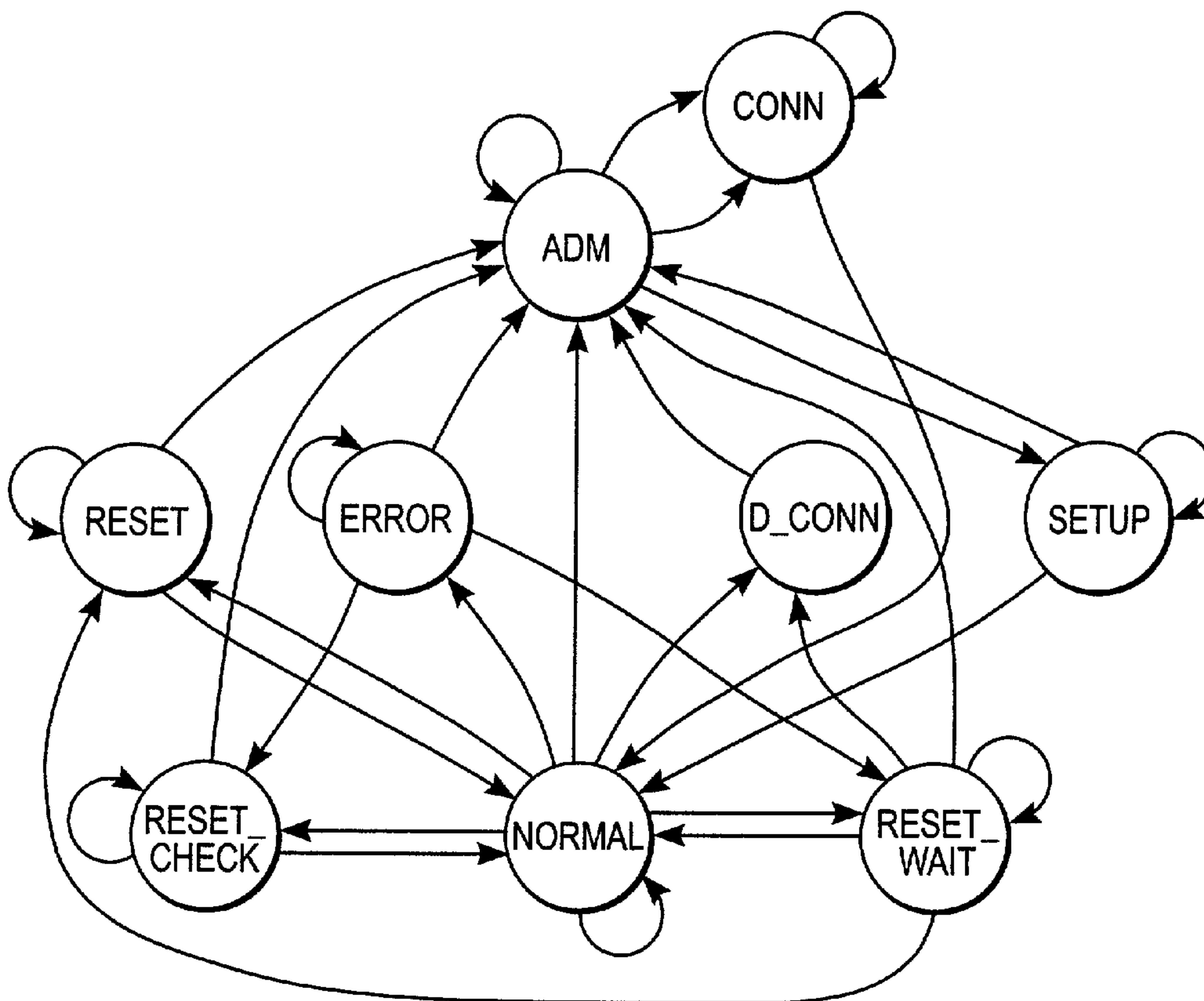
FIG. 82 (PRIOR ART)
