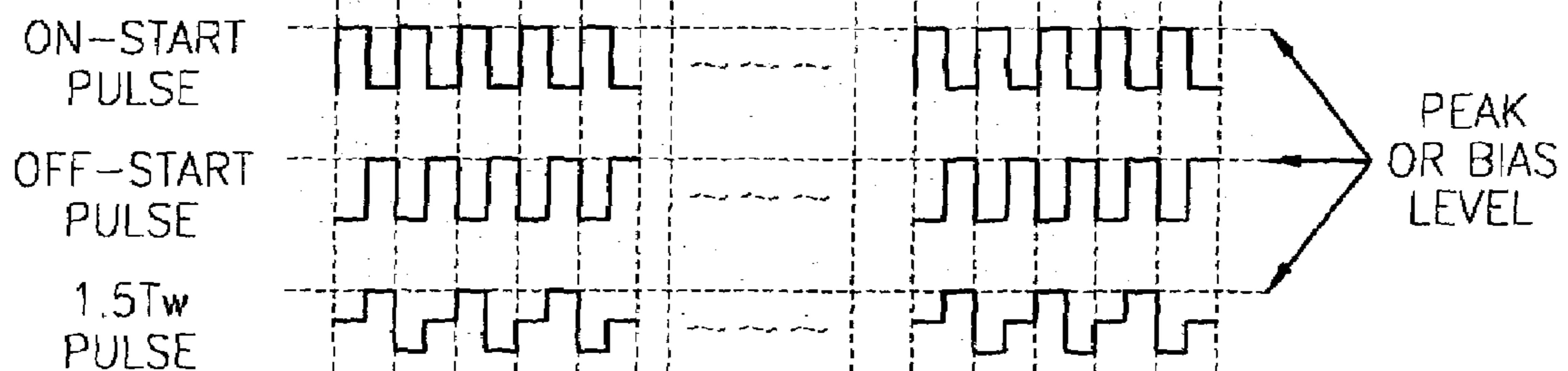
FIG. 6C WHEN REFERENCE LEVEL IS USED AS TOP
