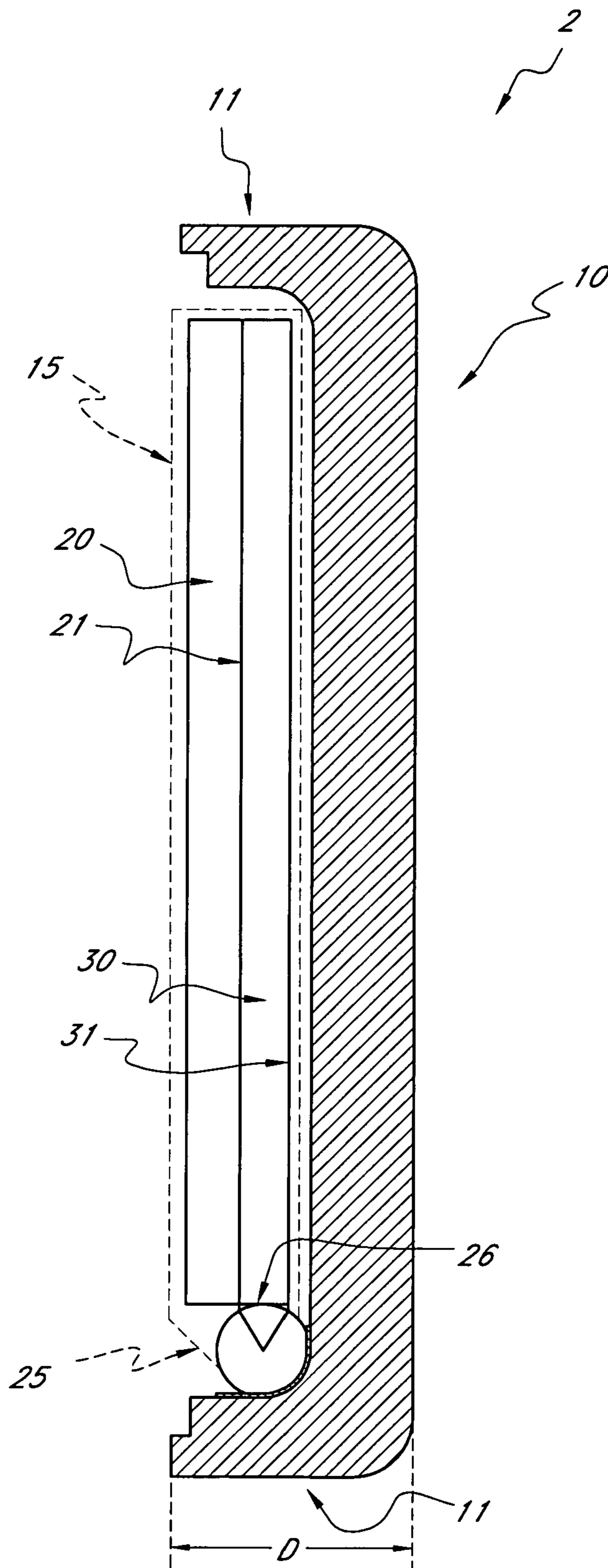
FIG. 2 (PRIOR ART)
