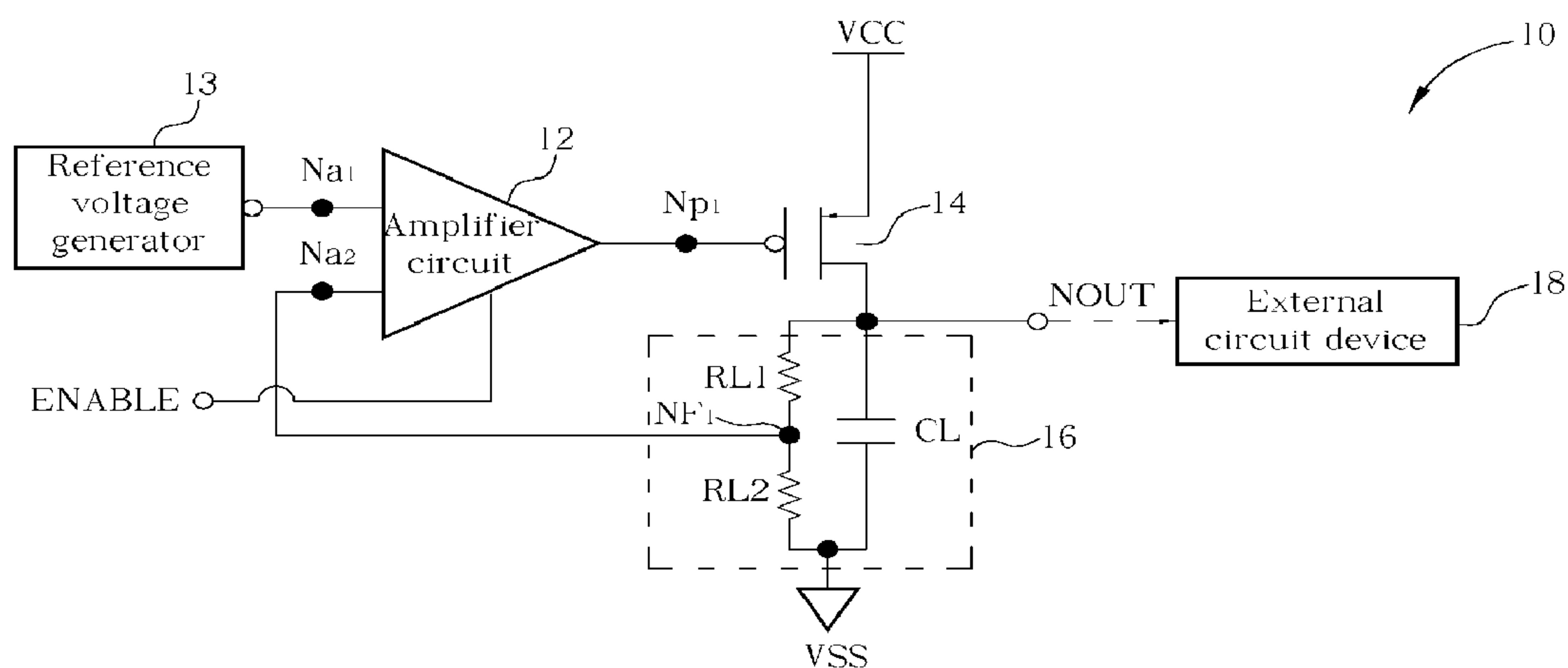
Fig. 1 Related Art
