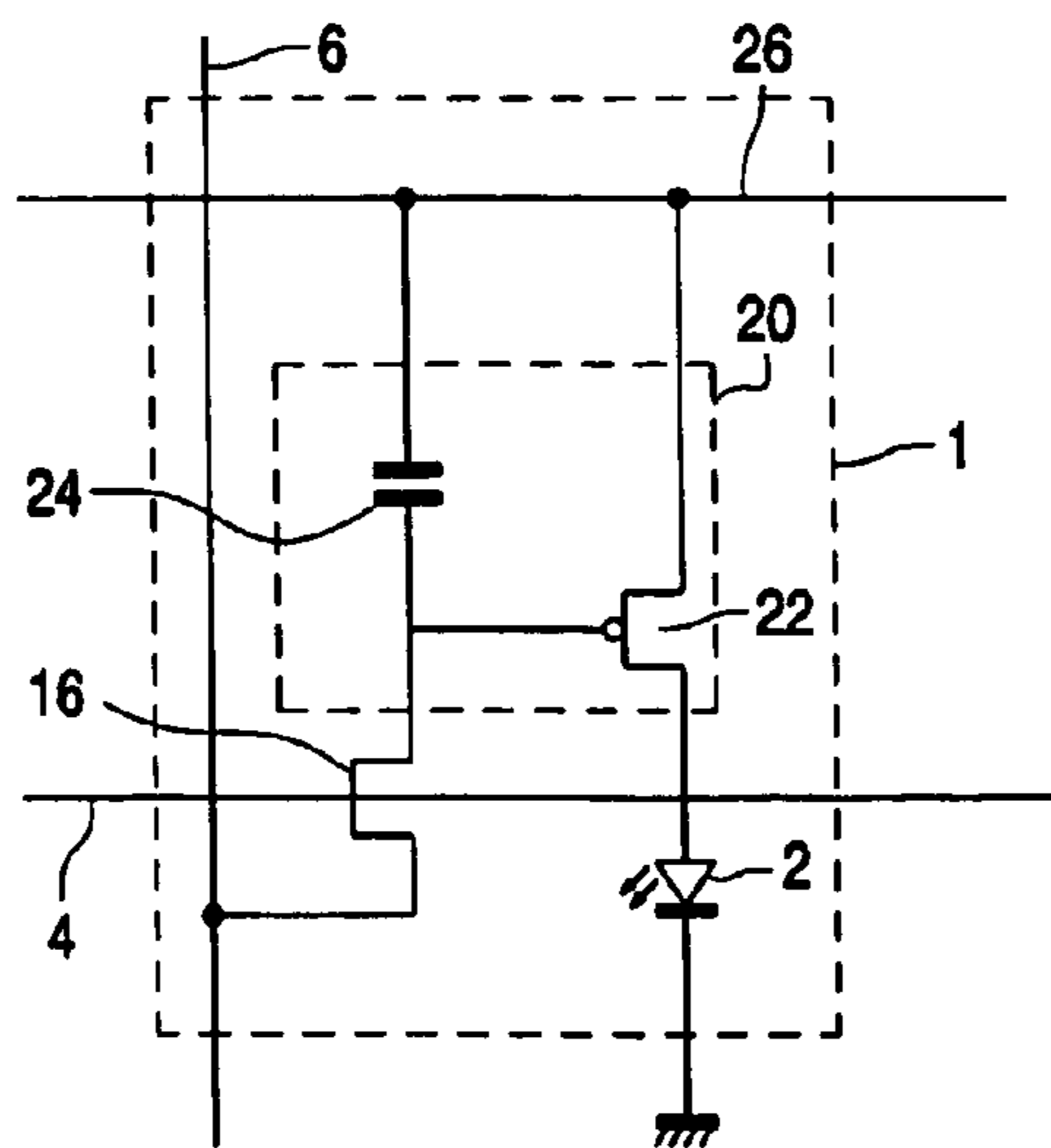
FIG. 2 PRIOR ART
