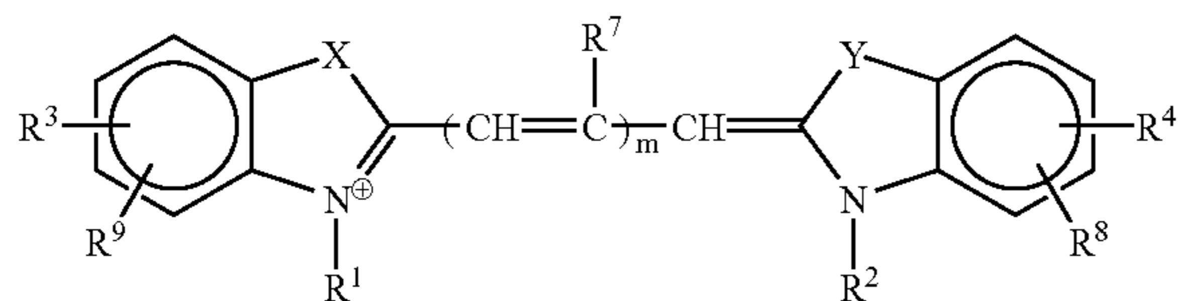
cyanine
