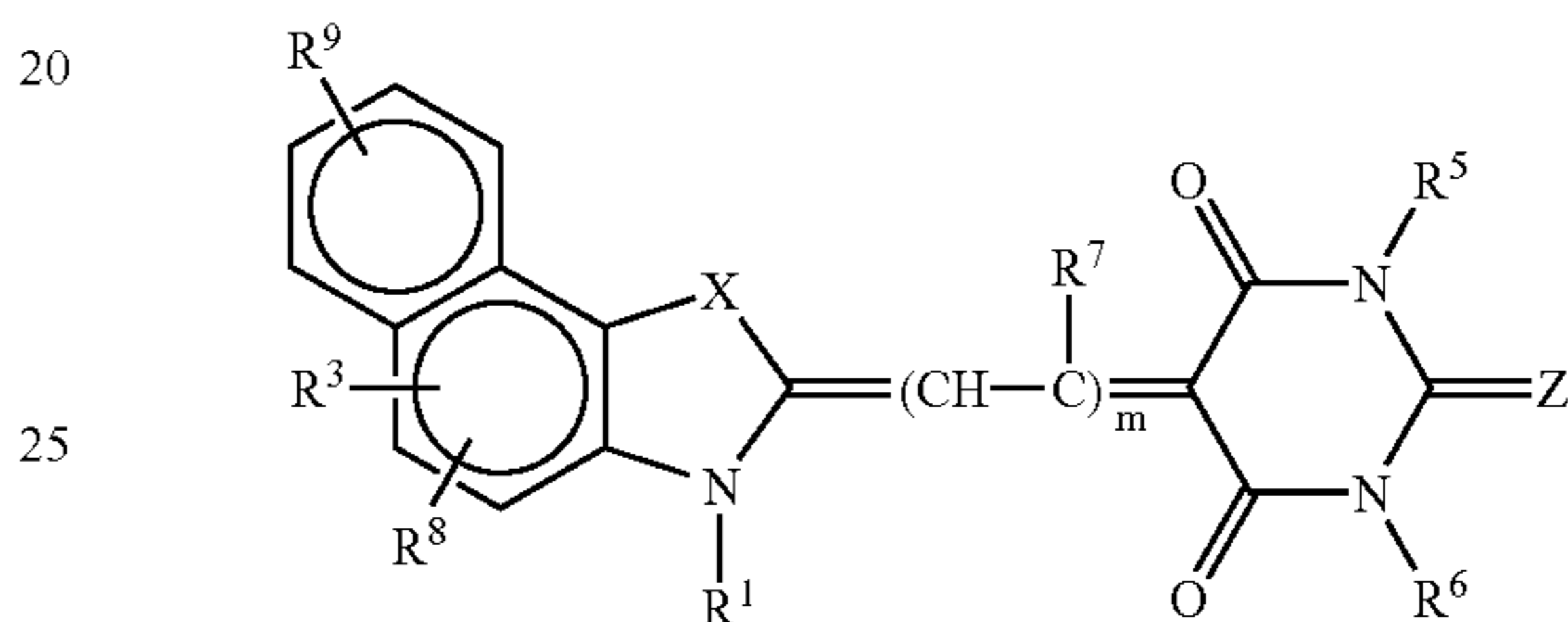
merocyanine
