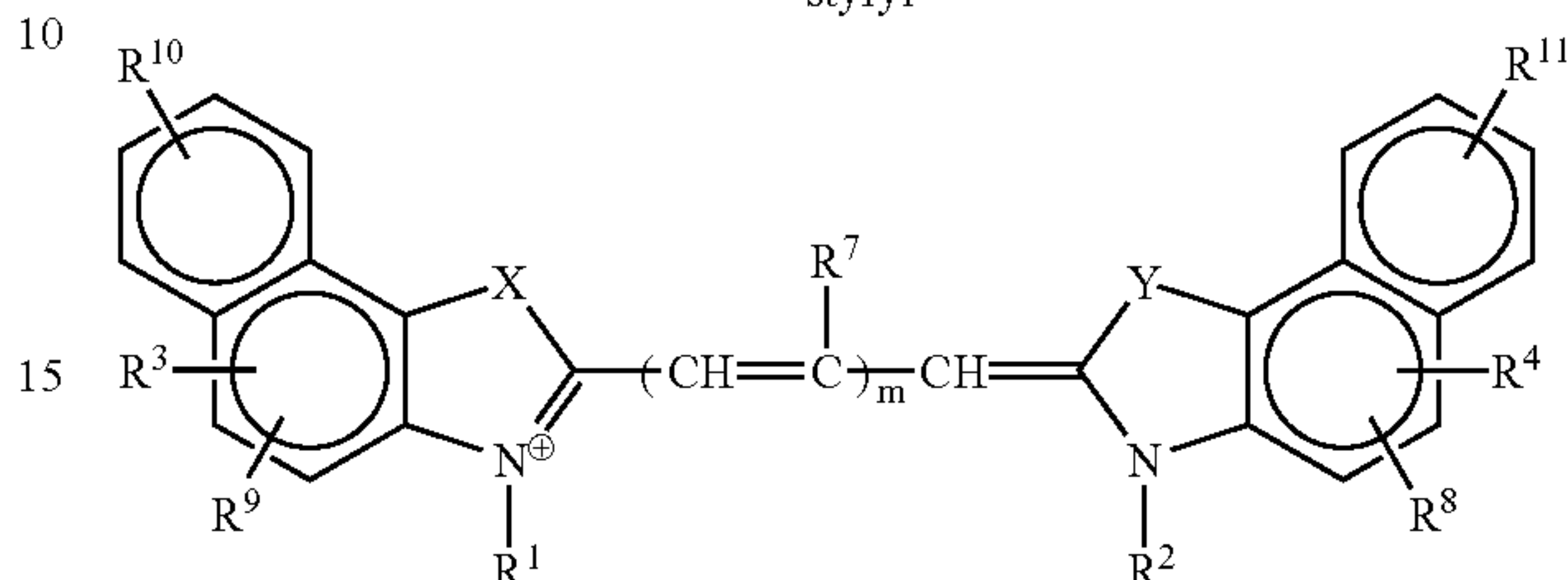
cyanine
