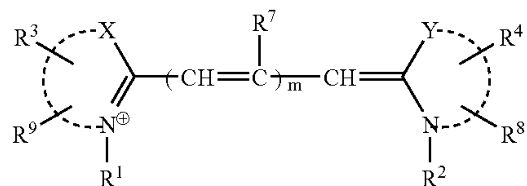
cyanine
