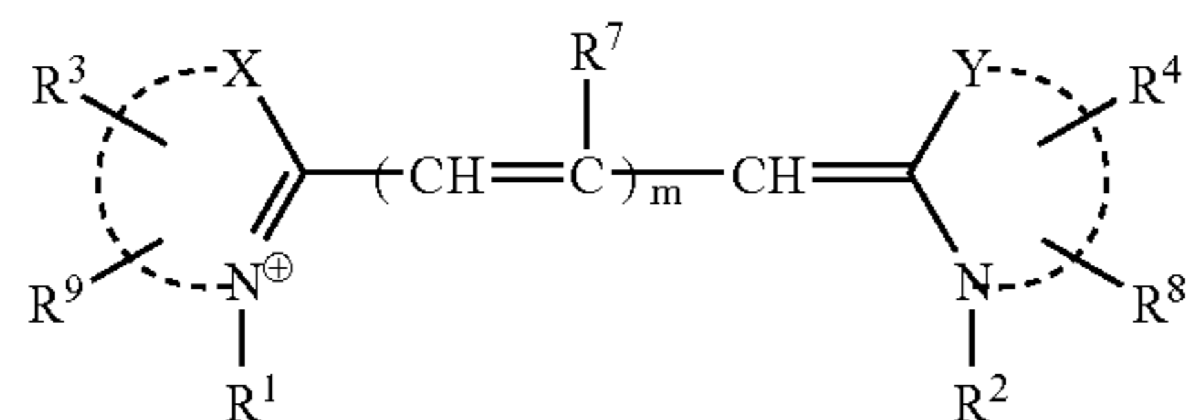
cyanine
