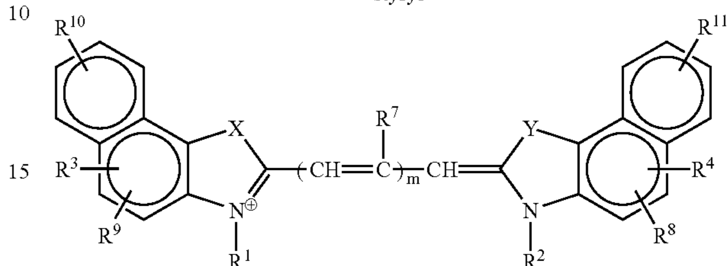
cyanine
