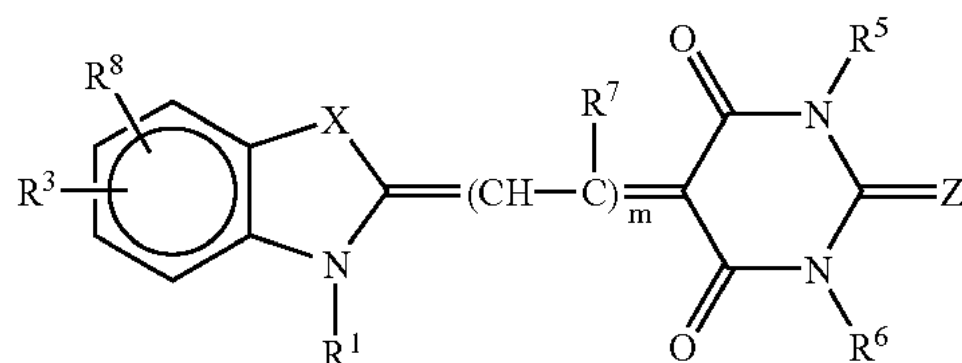
merocyanine
