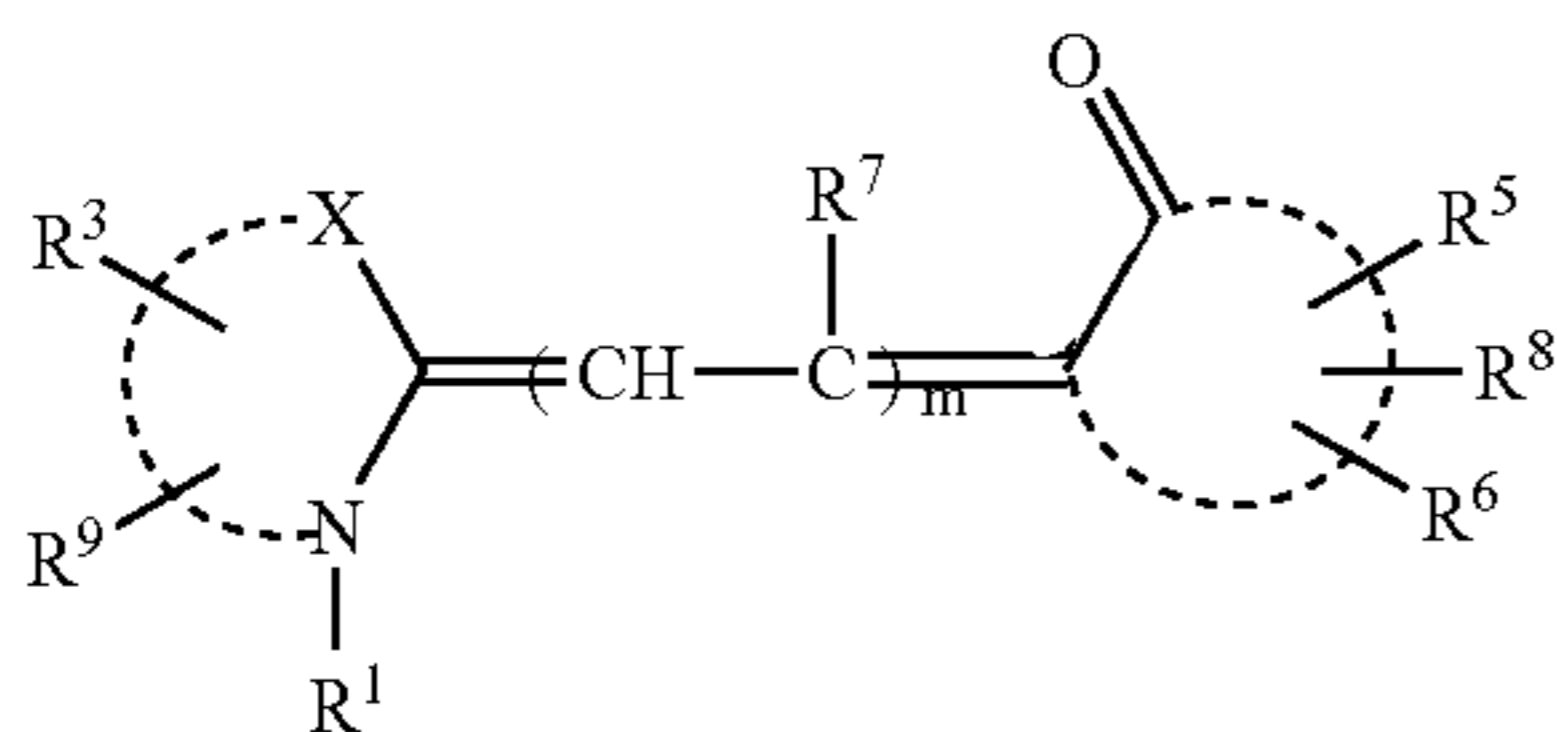
merocyanine
