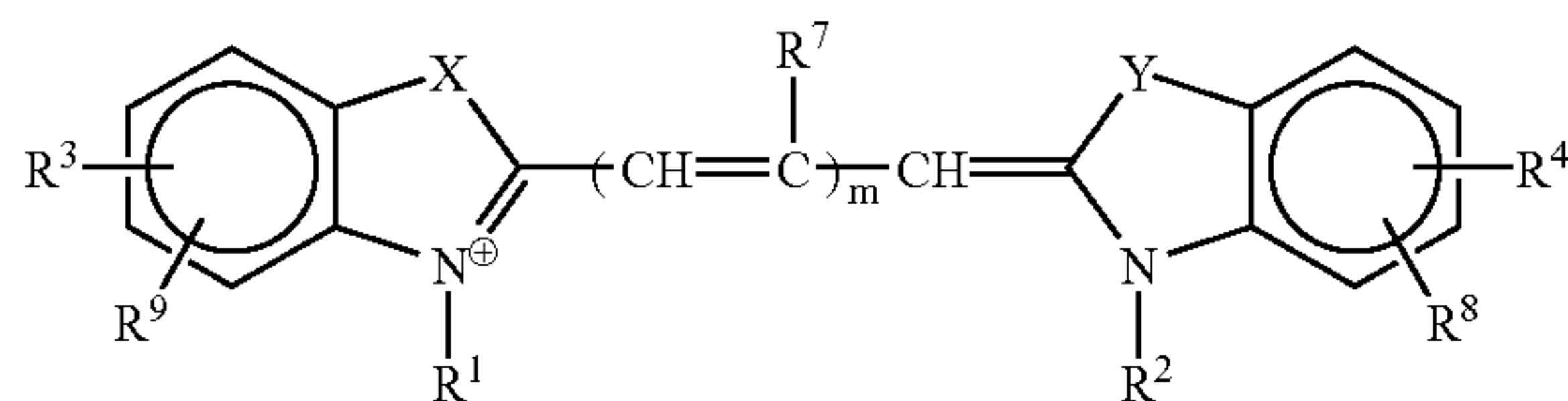
cyanine
