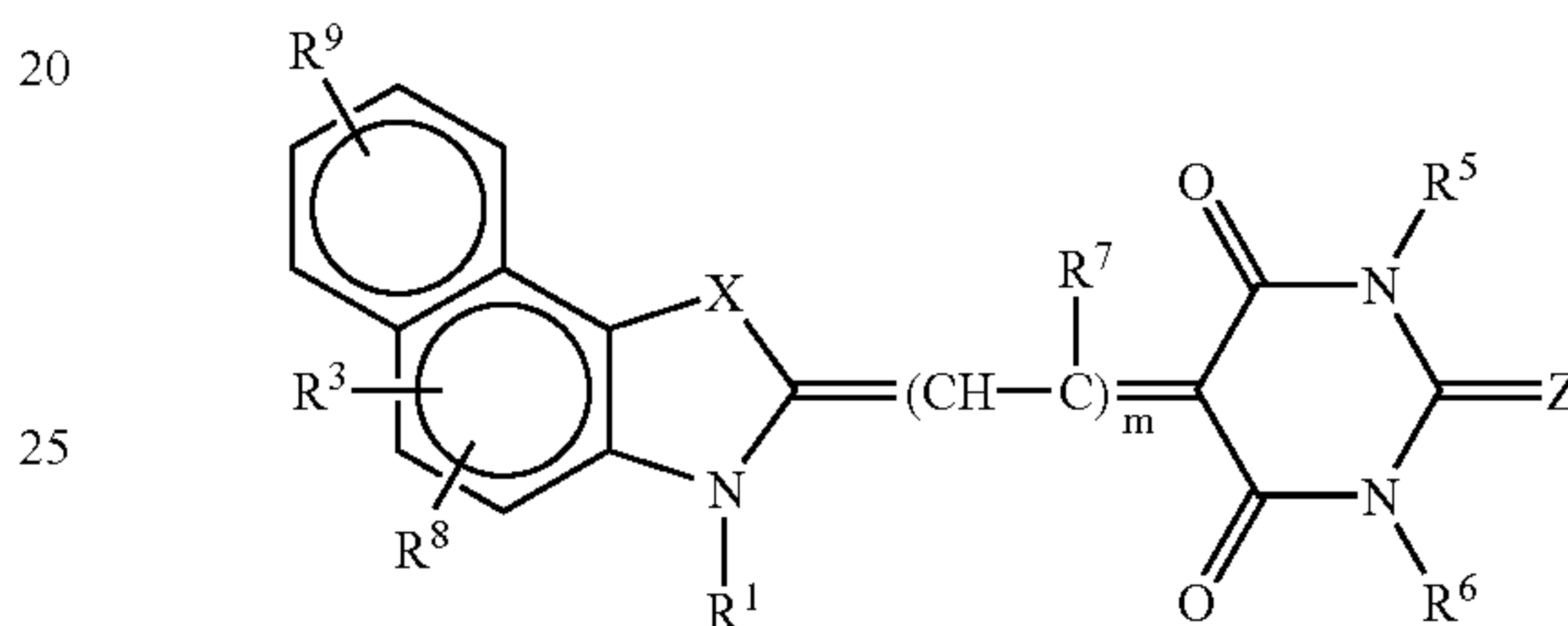
merocyanine
