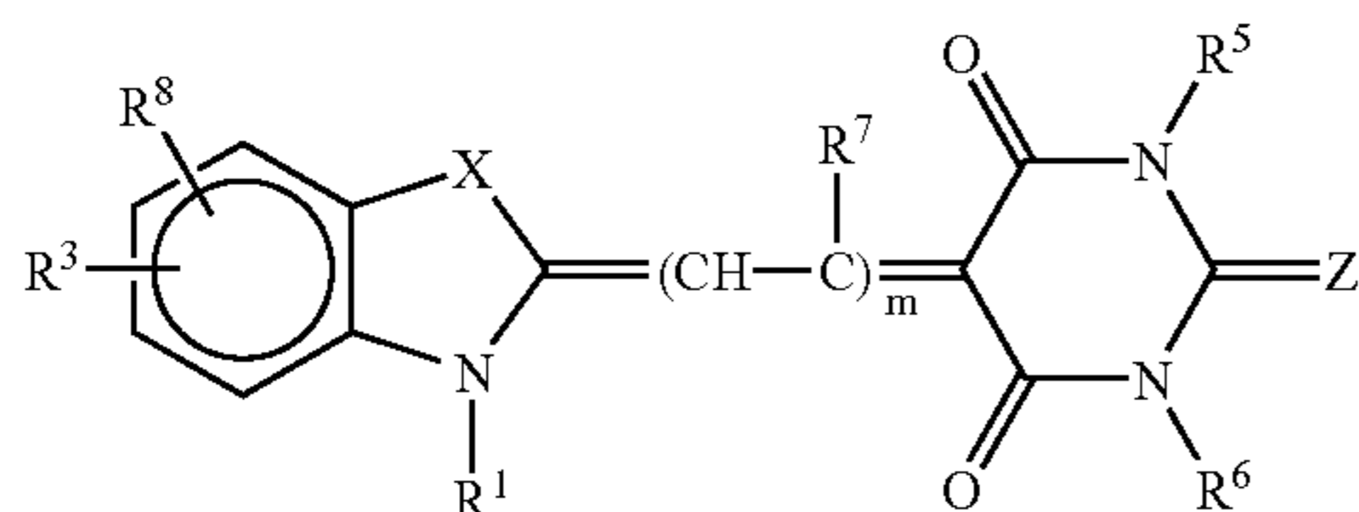
merocyanine
