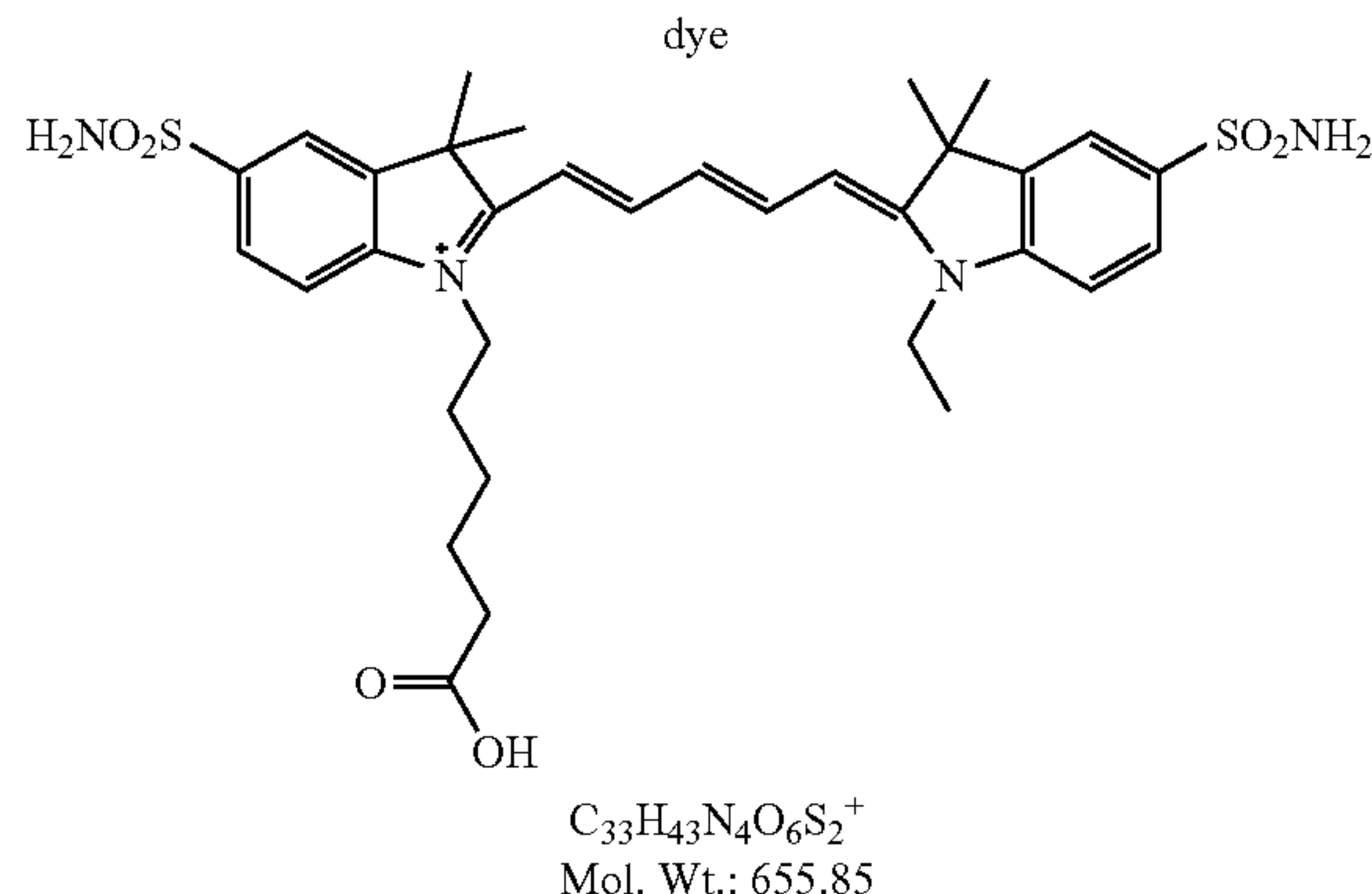
compound 1
