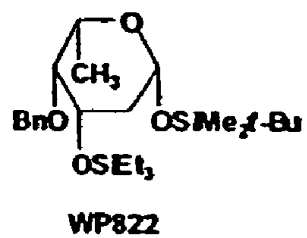
FIG. 29 Structure of WP822
