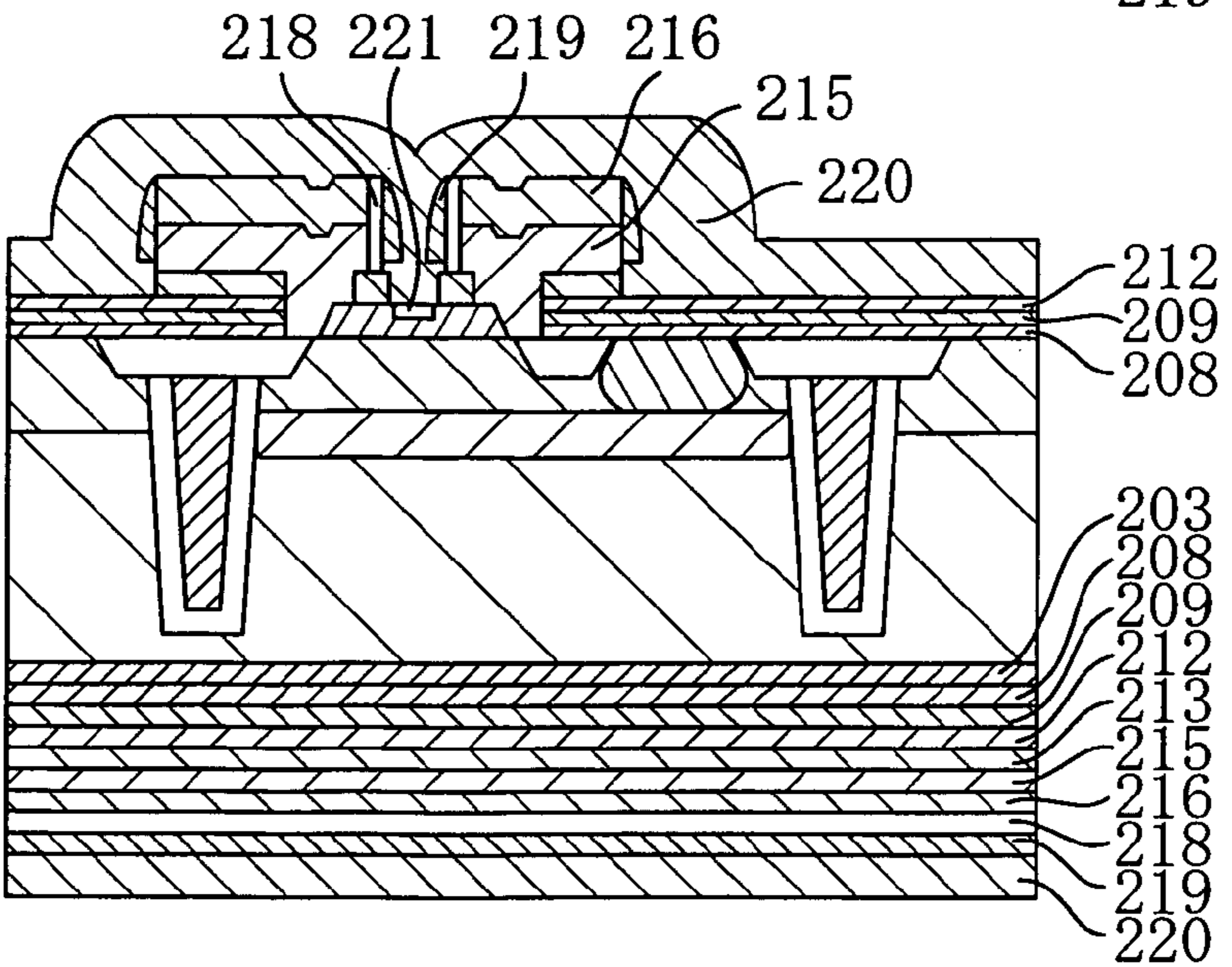
FIG. 7C PRIOR ART
