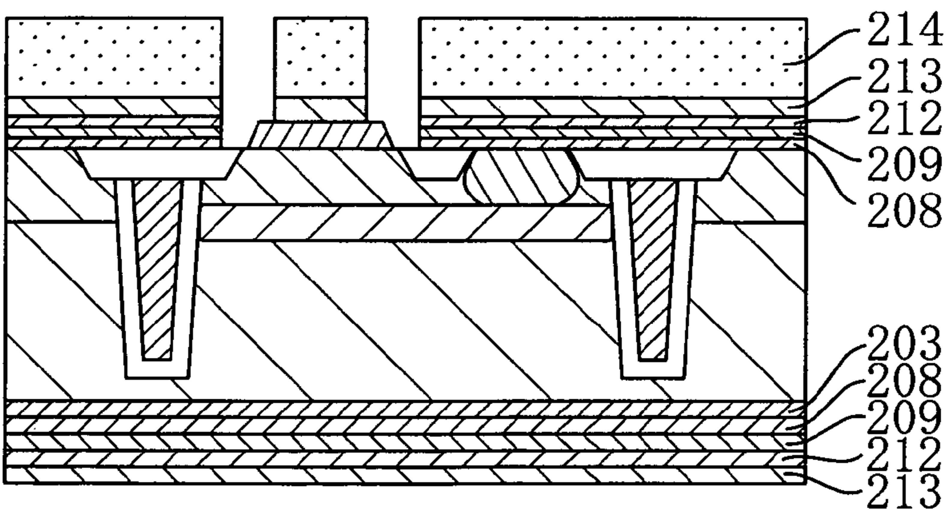
FIG. 6C PRIOR ART
