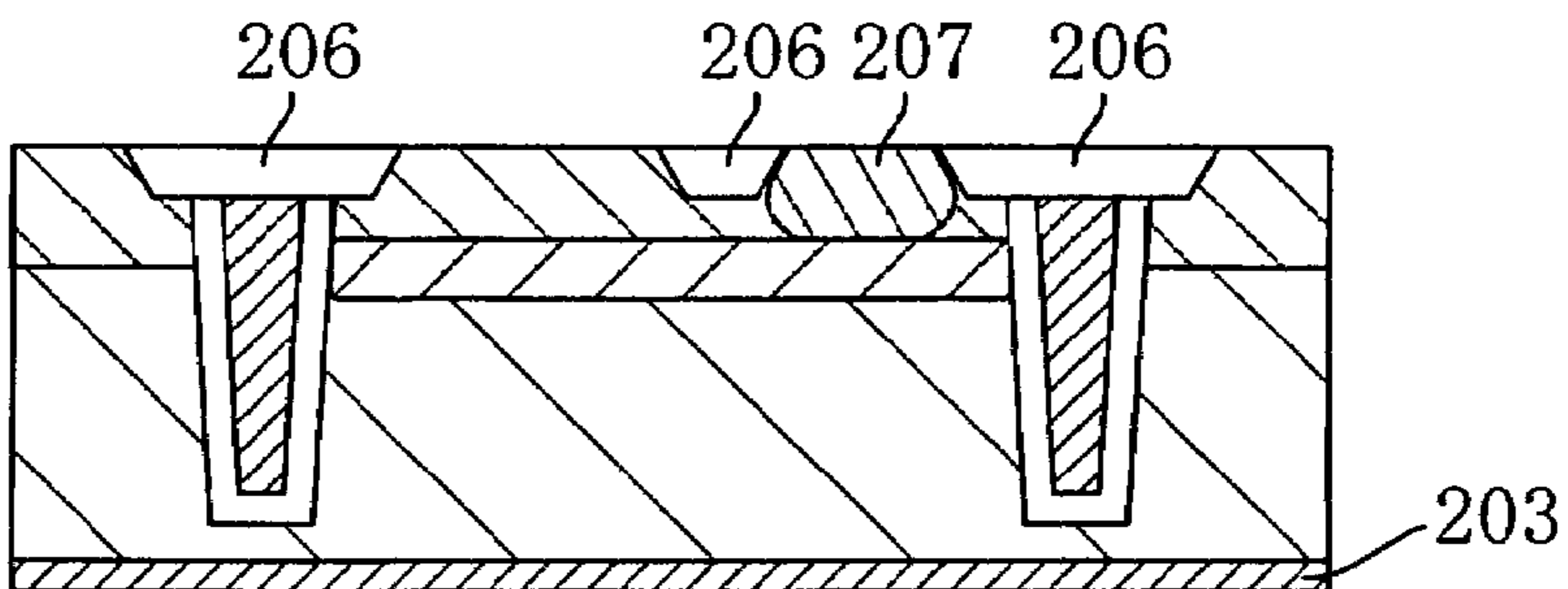
FIG. 5C PRIOR ART
