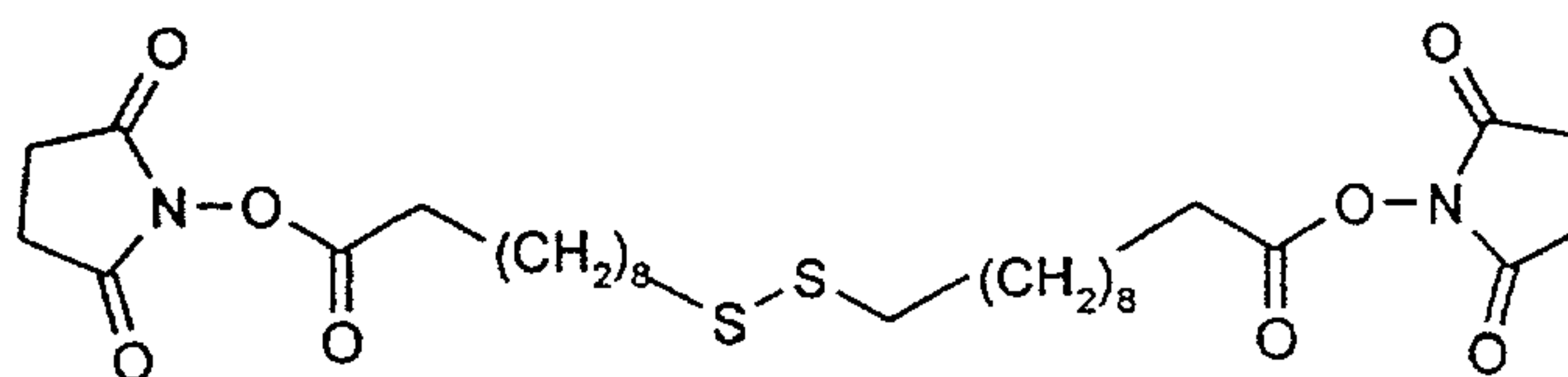
Dithio-bis(succinimidylundecanoate)
