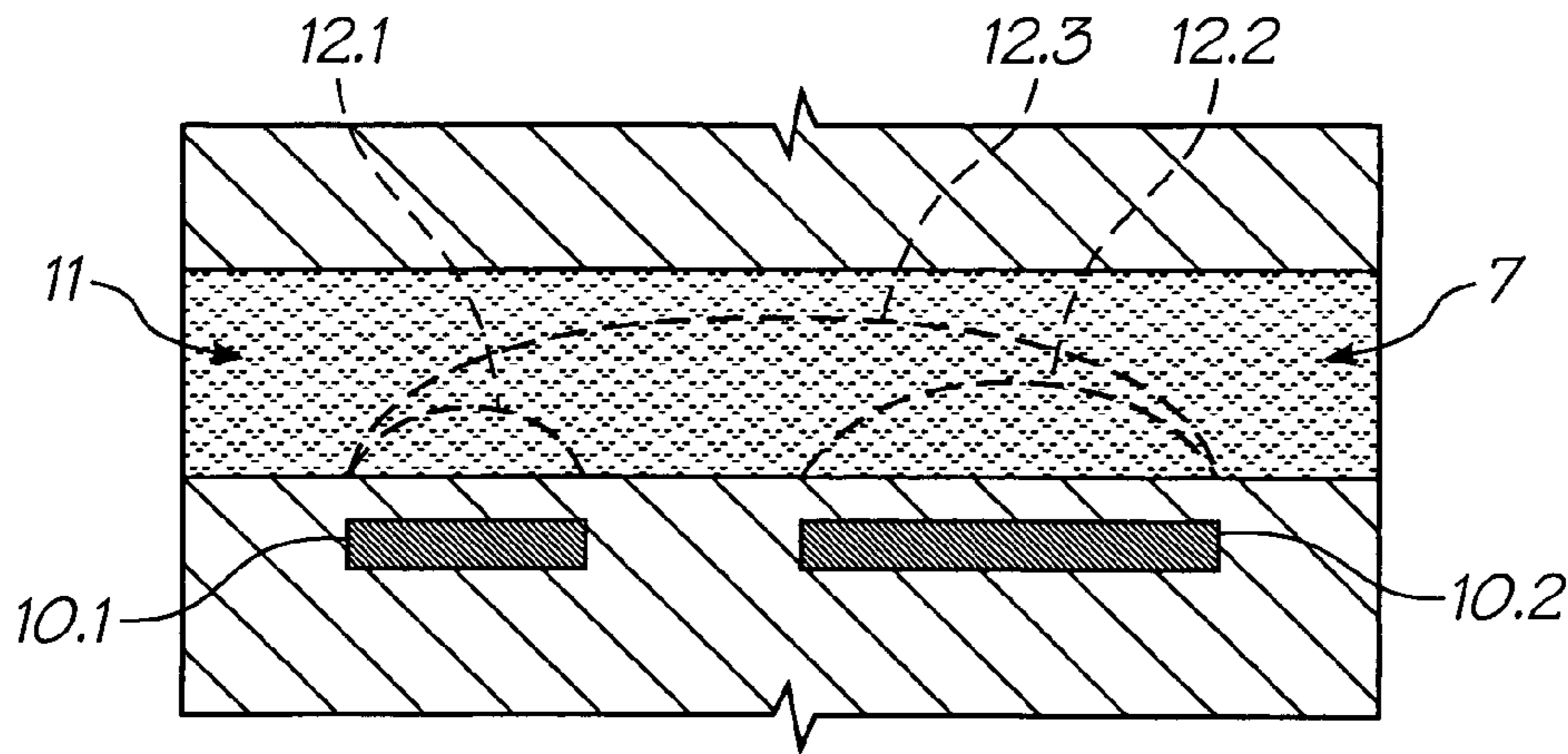
FIG. 52 (PRIOR ART)
