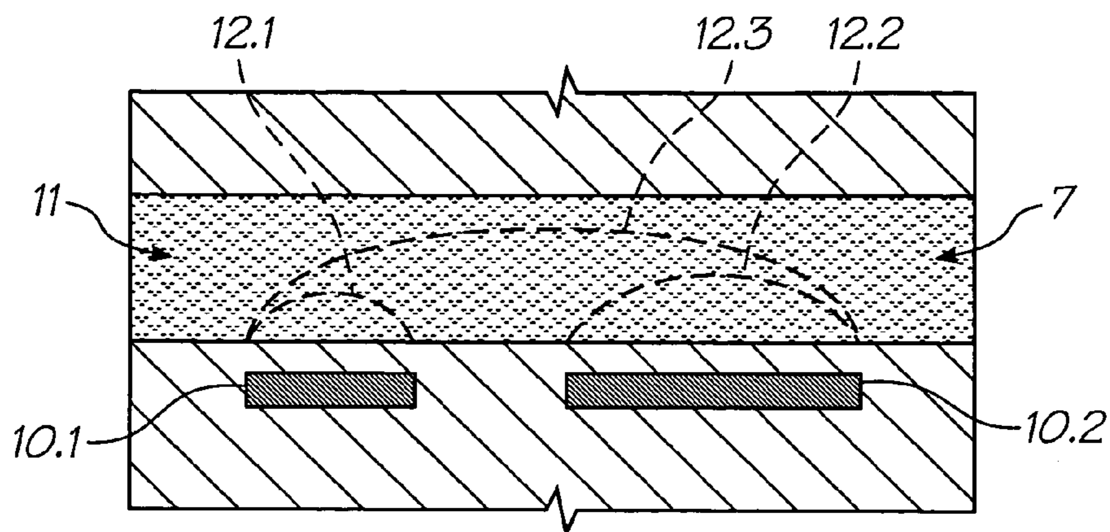
FIG. 52 (PRIOR ART)
