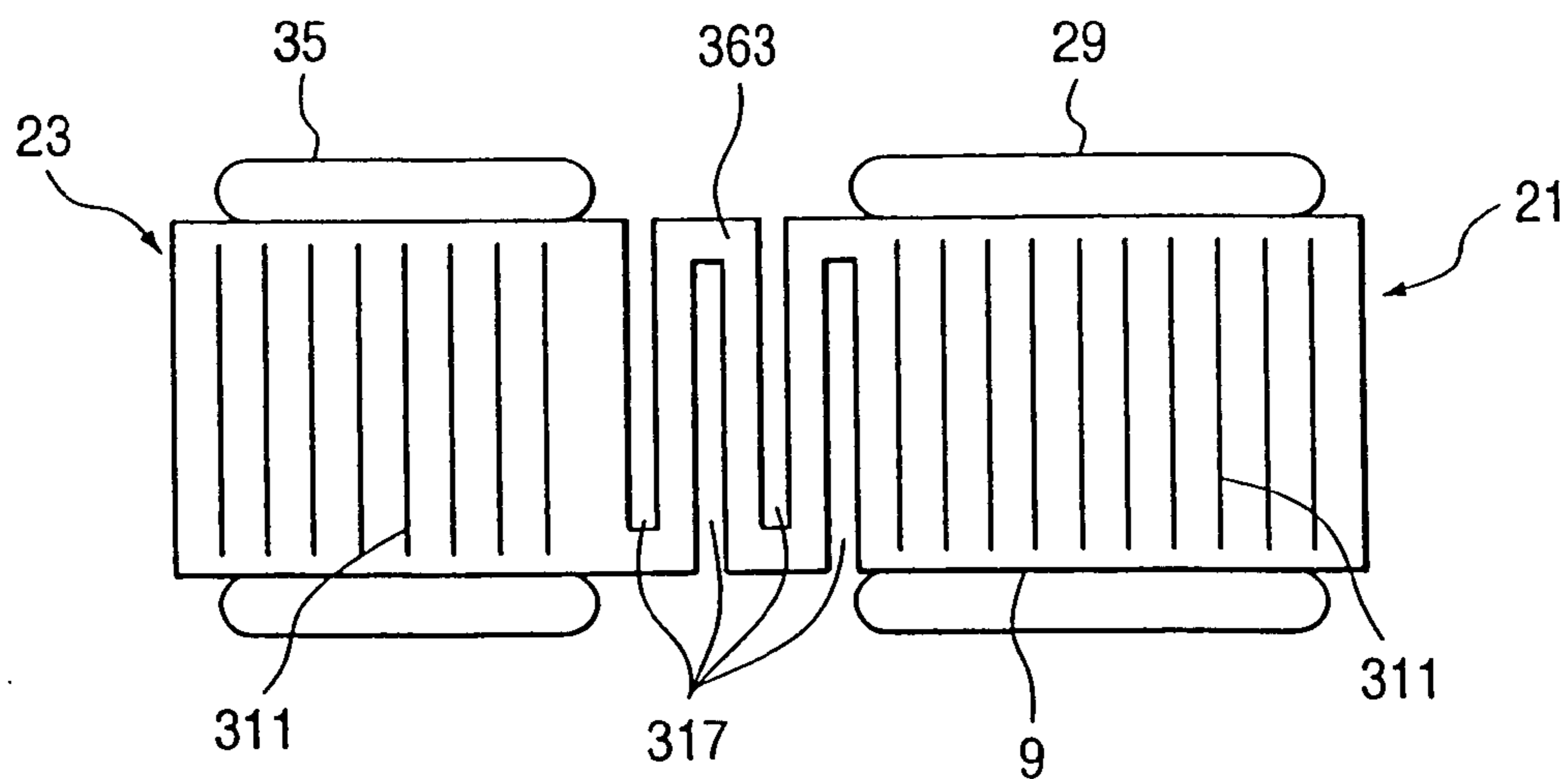
FIG. 43 RELATED ART
