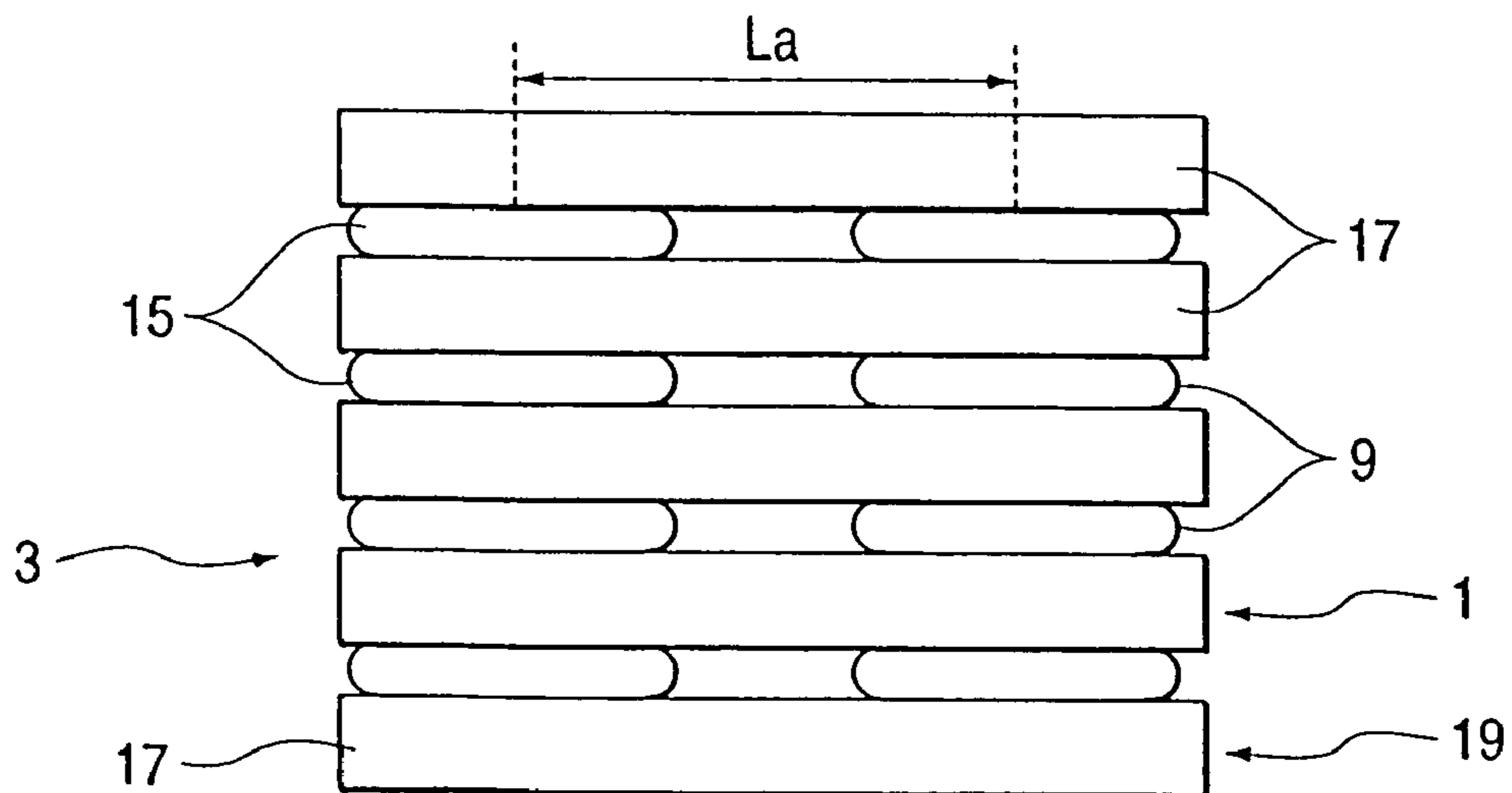
FIG. 40 RELATED ART
