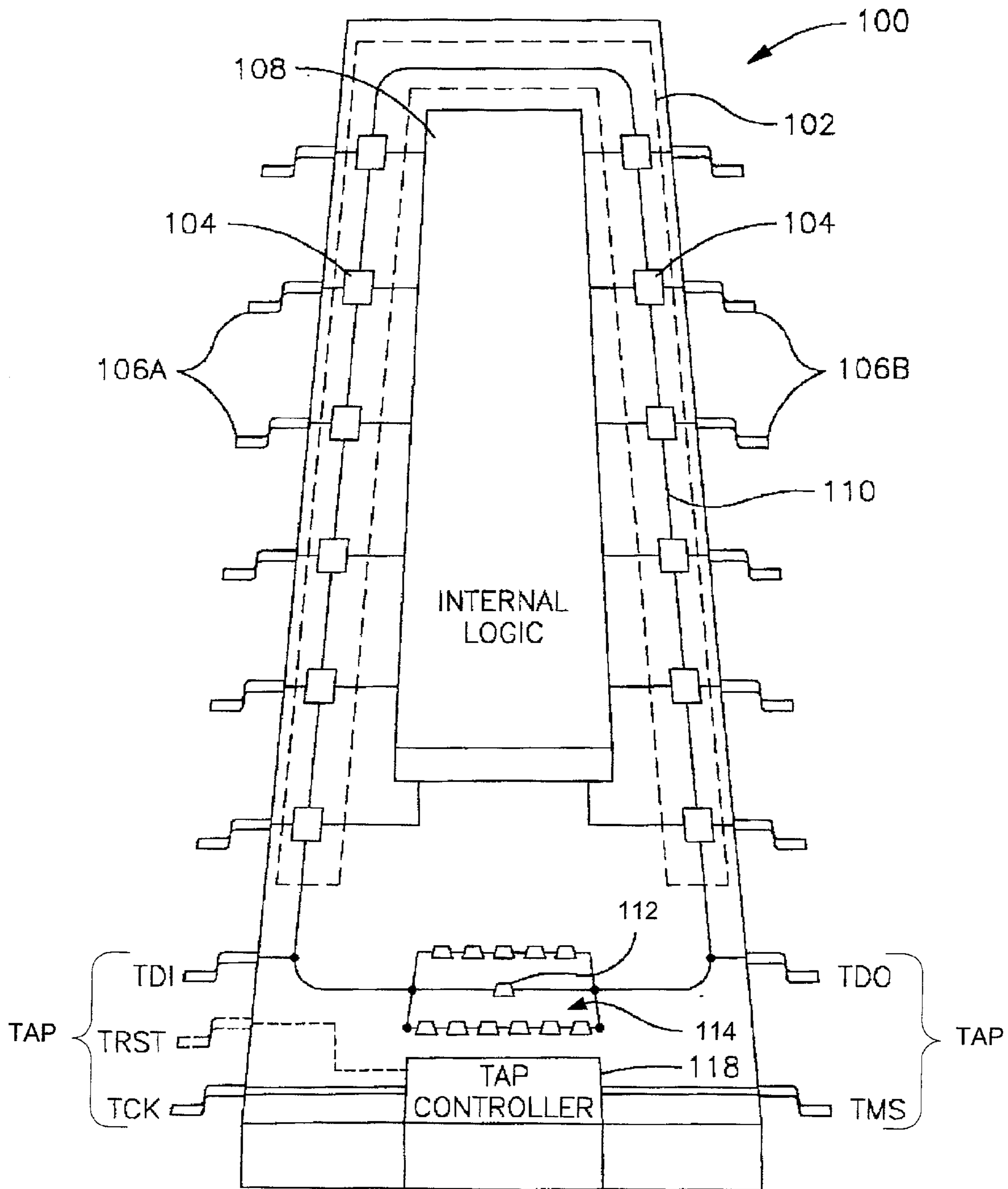
FIG. 1 (PRIOR ART)
