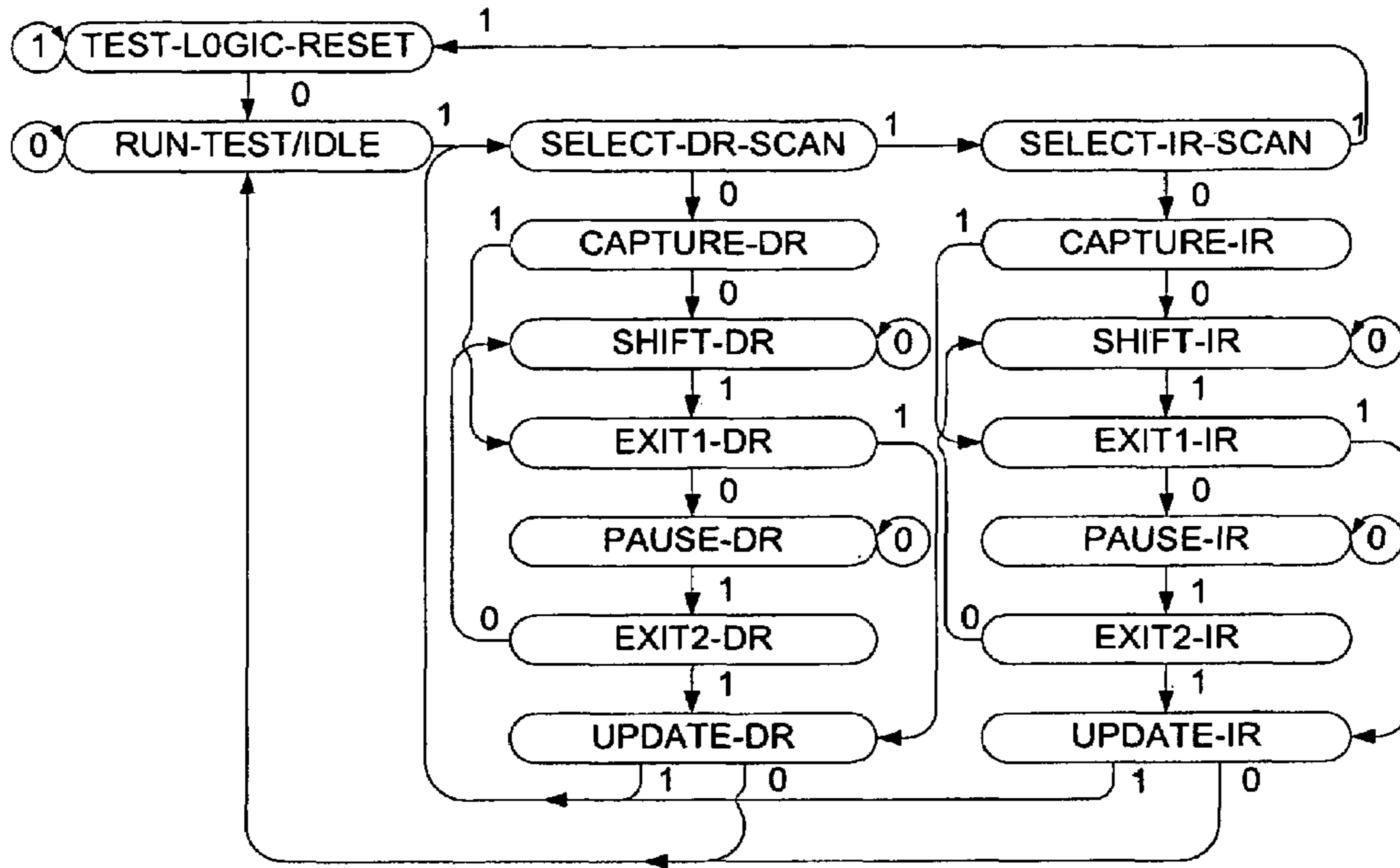
FIG. 3 (PRIOR ART)
