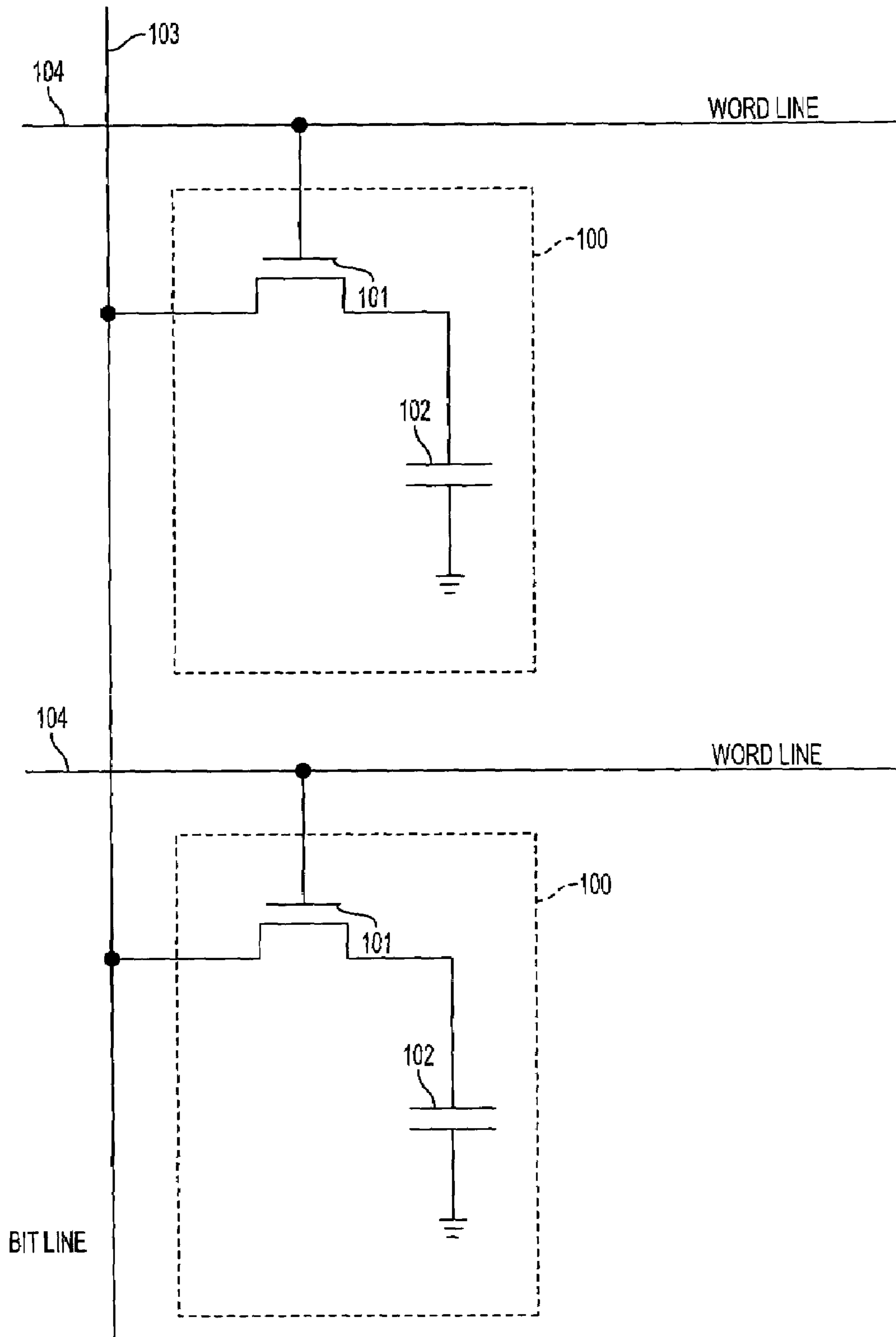
FIG. 1 (PRIOR ART)
