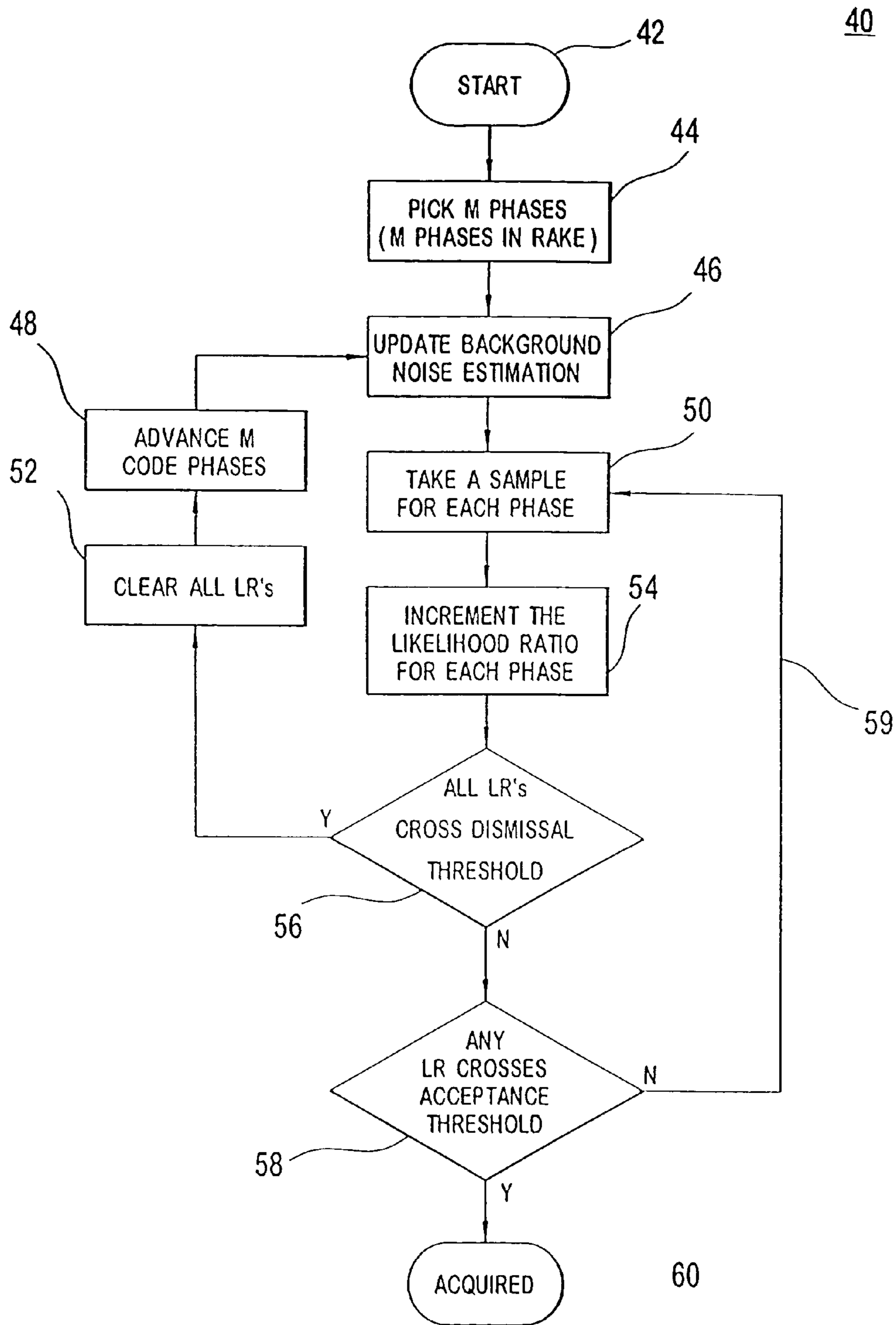
FIG. 2 (PRIOR ART)
