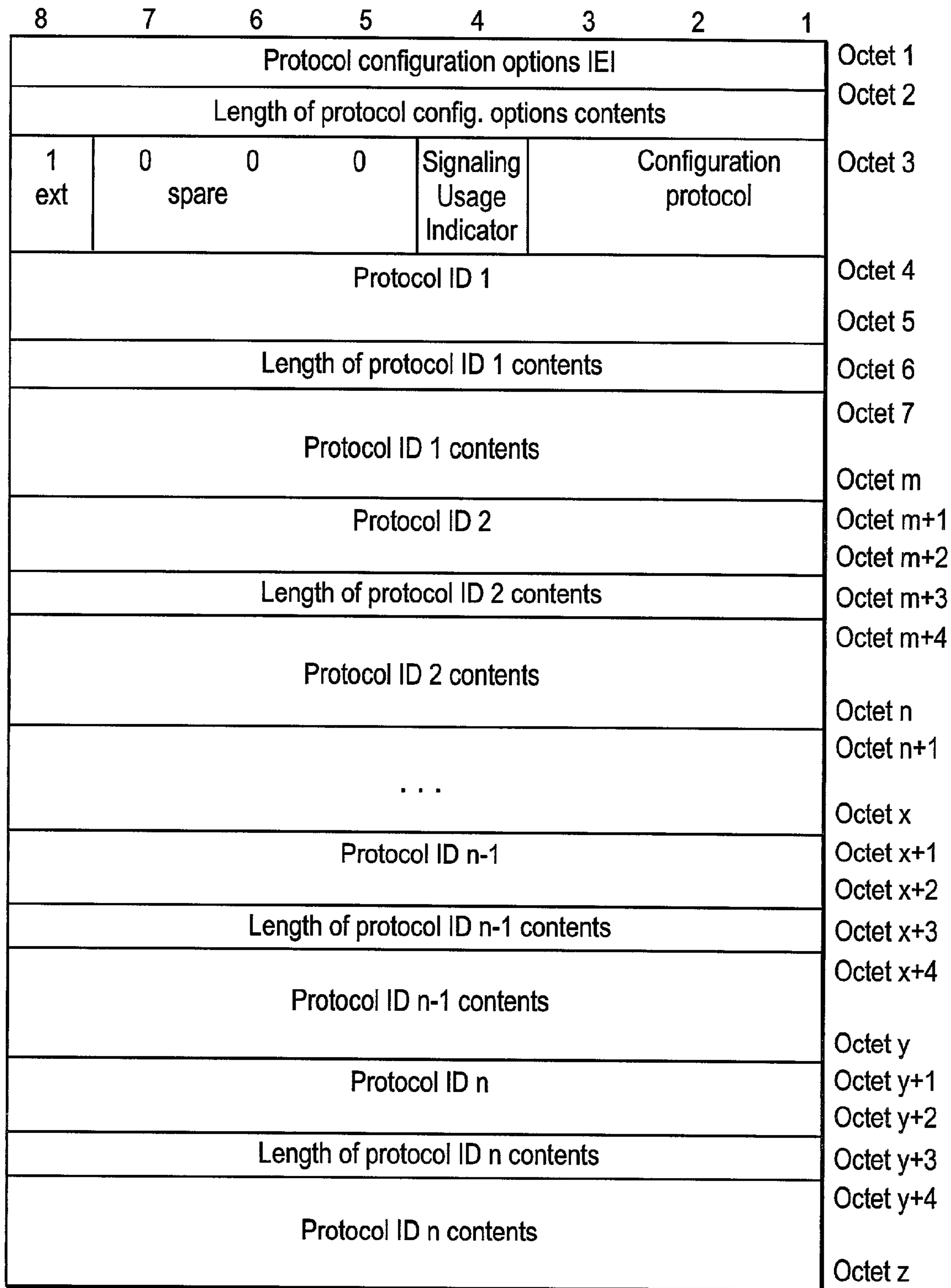
Protocol Configuration Options Information Element
