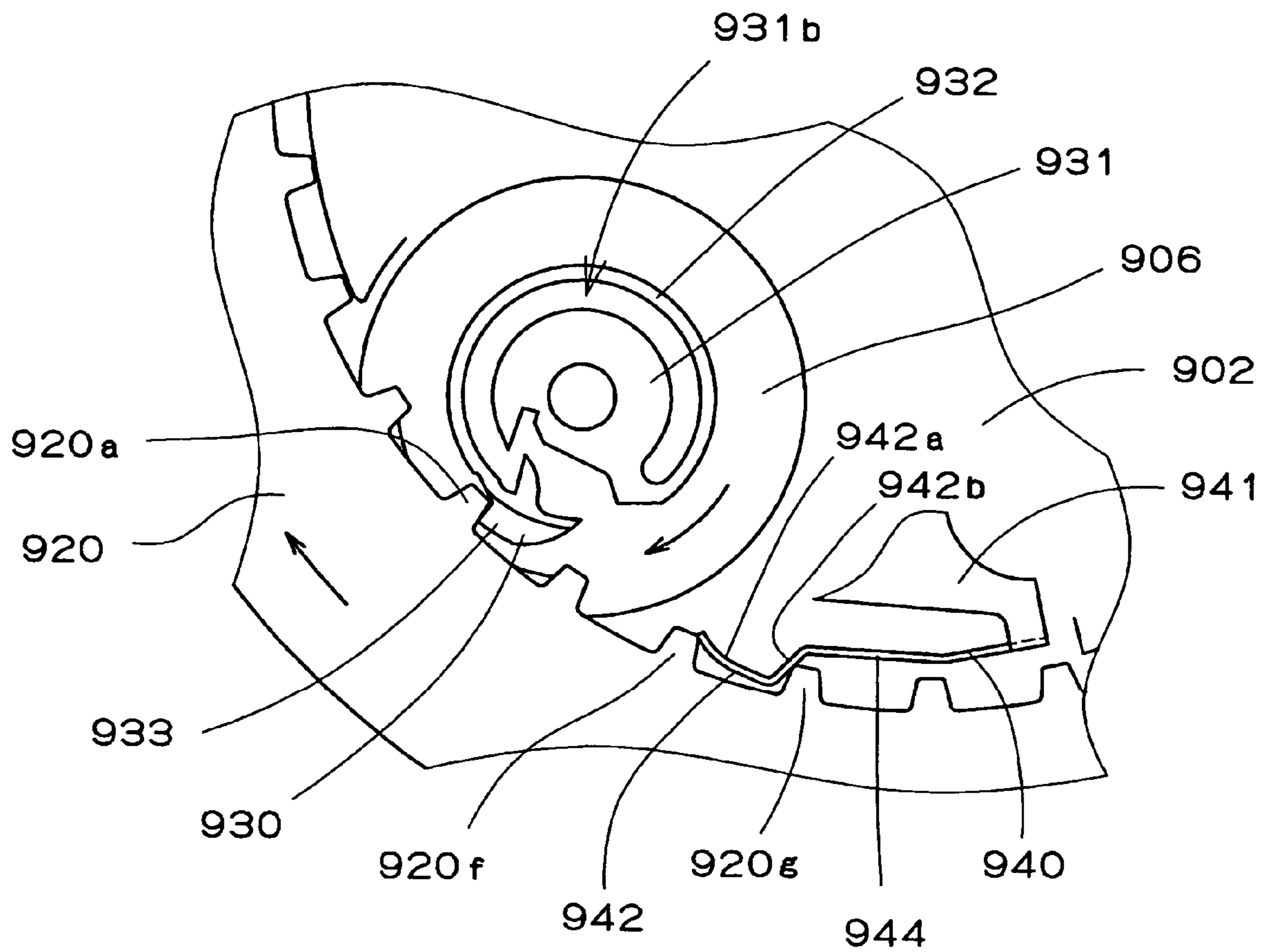
FIG. 29 Prior Art
