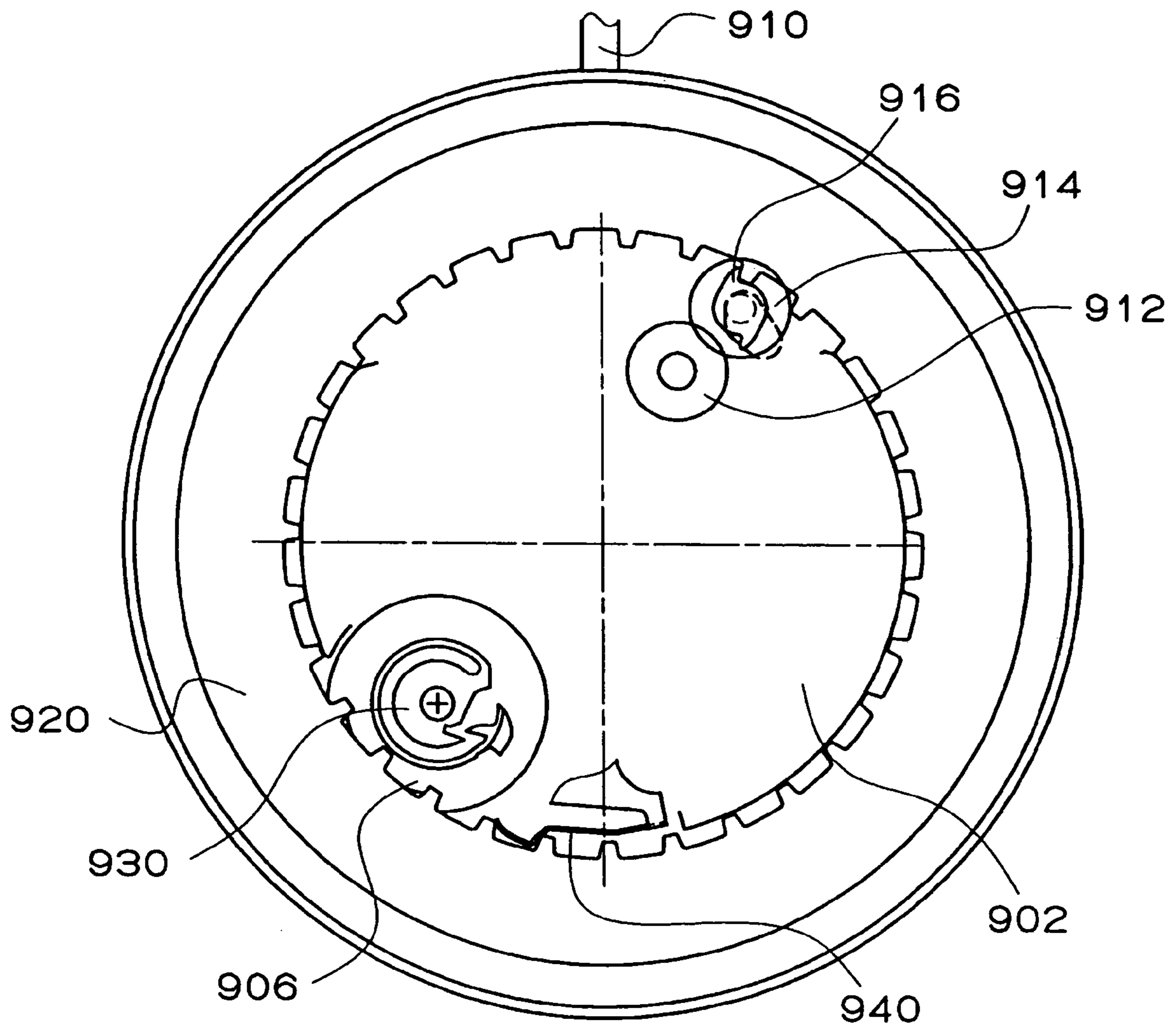
FIG. 25 Prior Art
