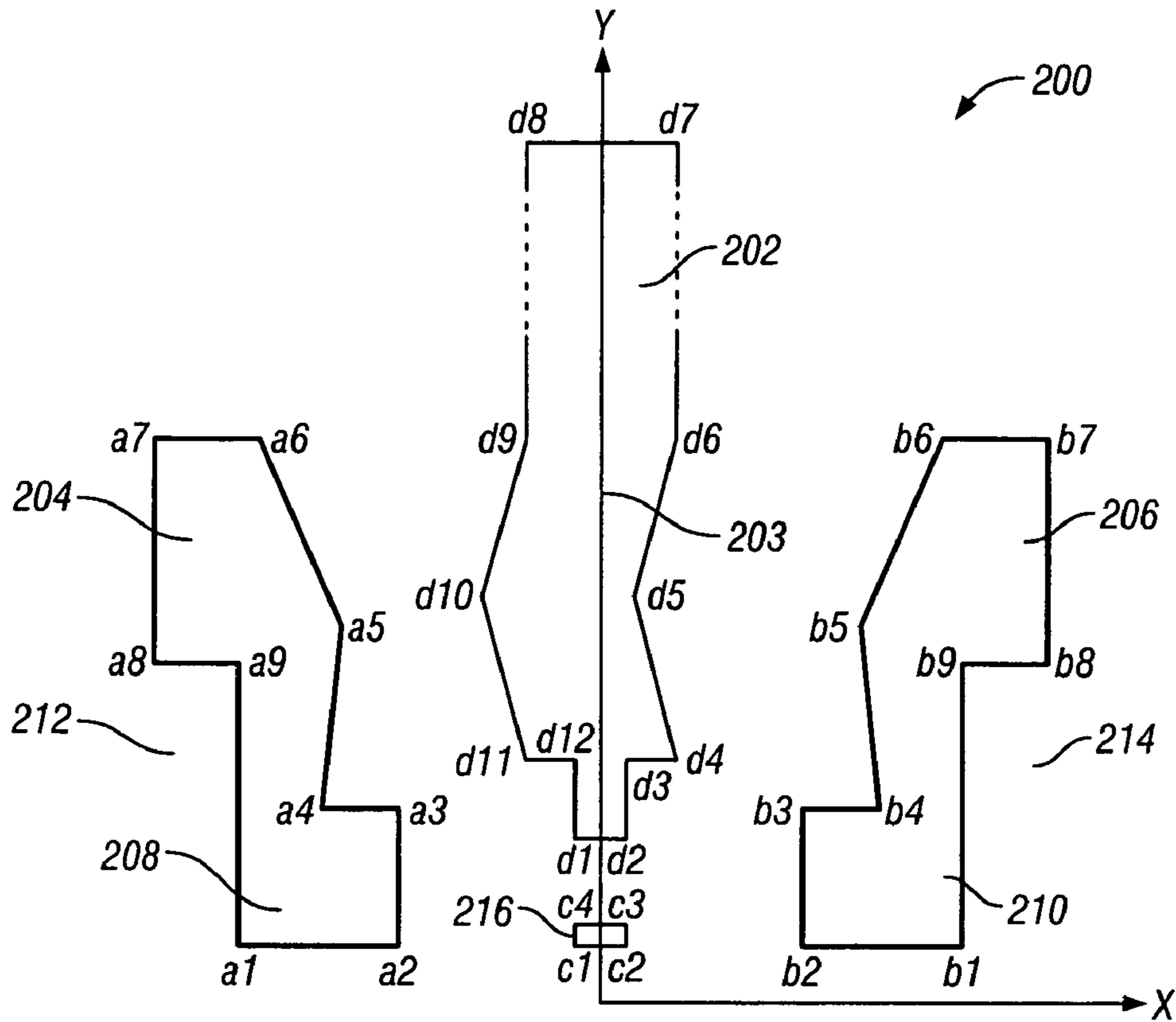
SCHMATIC TEMPLATE OF ANTENNA#2
