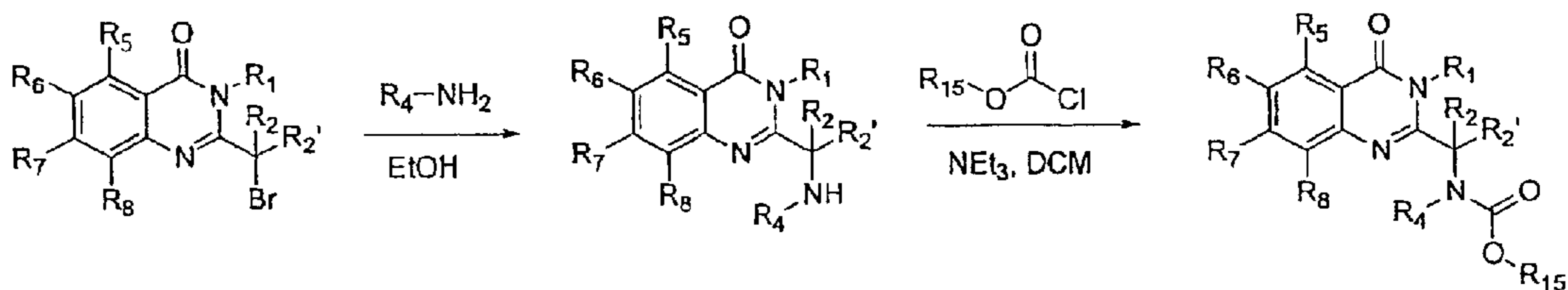
Figure 5c: Urea Synthesis
